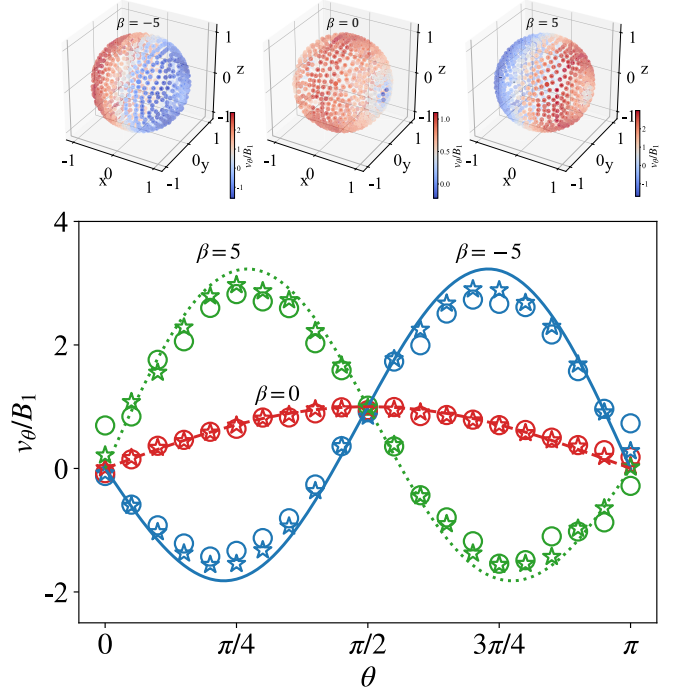
FIG. 2. The distribution of the slip velocity on the squirmer surface. The results of the smoothed particle dynamics for Re = 0.01 are expressed as scatter points. The circle represent a resolution of \Delta x = R/10 , while the star denotes \Delta x = R/16 . The analytic solution for Re = 0 is expressed as lines. Top are the distribution of fluid smoothed particle dynamics particles and their slip velocity within one resolution from the squirmer.
