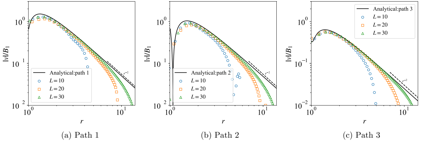
FIG. 14. Box size study: The convergence of the flow field generated by an individual squirmer with increasing box size. (a) Path 1 is along the negative swimming direction, (b) path 2 is along the positive flow direction, and (c) path 3 is perpendicular to the flow direction. The black solid lines represent the analytic solution of the velocity field around a squirmer in bulk. The scatter represents the present simulation results for cubic boxes with different side lengths L .
