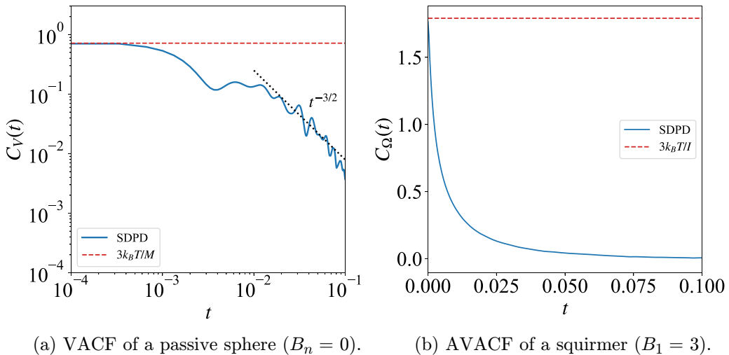
FIG. 9. Velocity autocorrelation function of a passive sphere and angular velocity autocorrelation function of a squirmer.
