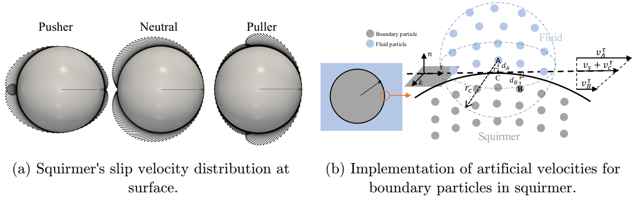
FIG. 1. Schematic of modeling a squirmer. To achieve the slip velocity of the squirmer in (a), artificial velocities of the boundary particles are assigned in (b). Given a fluid particle A, an interface plane tangential to the sphere is defined to be perpendicular to a line AC of length d_A , where C is the point of intersection on the surface. A Cartesian coordinate is chosen such that the direction n is perpendicular to the interface plane and the direction \tau is on the interface plane and coplanar with the plane containing n and the direction of the squirmer head \mathbf{e} . B is an example of neighboring boundary particles with d_B away from the interface plane. During the pairwise dissipative force calculation between A and B, an artificial velocity \mathbf{v}_B is assigned to B so that the linear interpolation between \mathbf{v}_A and \mathbf{v}_B has a tangential velocity \mathbf{v}_s + \mathbf{v}_C^\tau at C and the other directions keep the original velocity component. Given the same fluid particle A, all other nearby boundary particles follow the same procedure of B.
