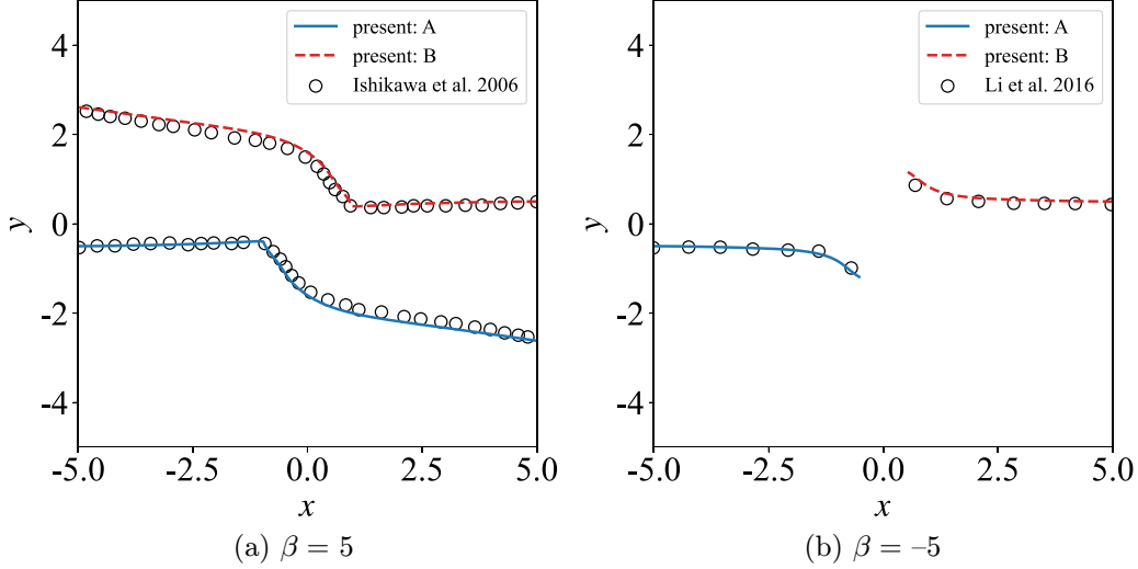
FIG. 7. Comparison of the trajectories of two colliding microswimmers.
