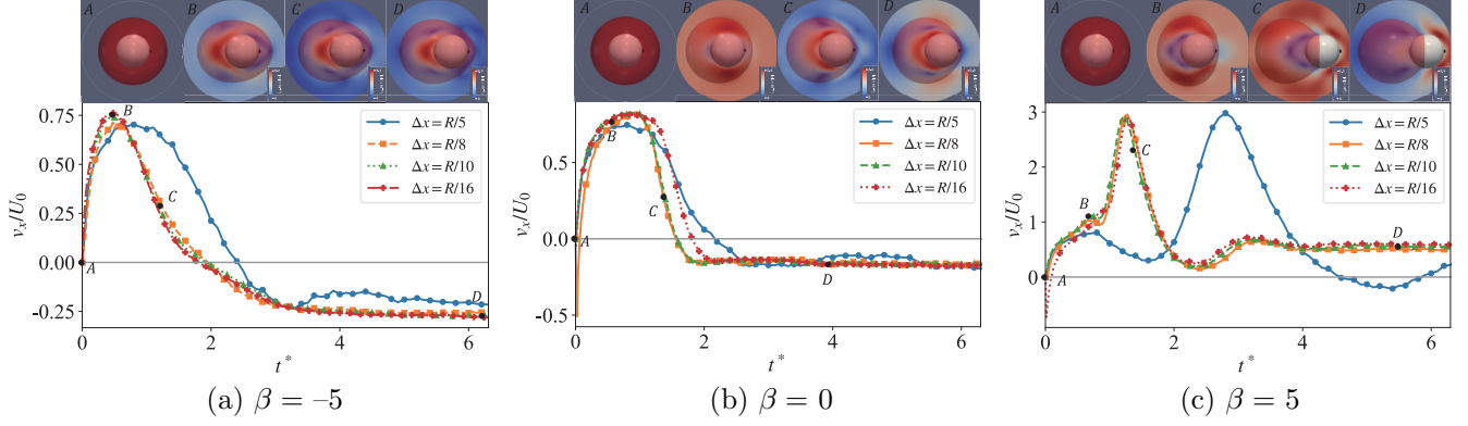
FIG. 12. The evolution of the squirmer's velocity in the x direction. The horizontal coordinate is the dimensionless time t^* = tU_0/R . The initial radius of droplets is R_d = 2 . The velocity field at several moments is displayed at the top.
