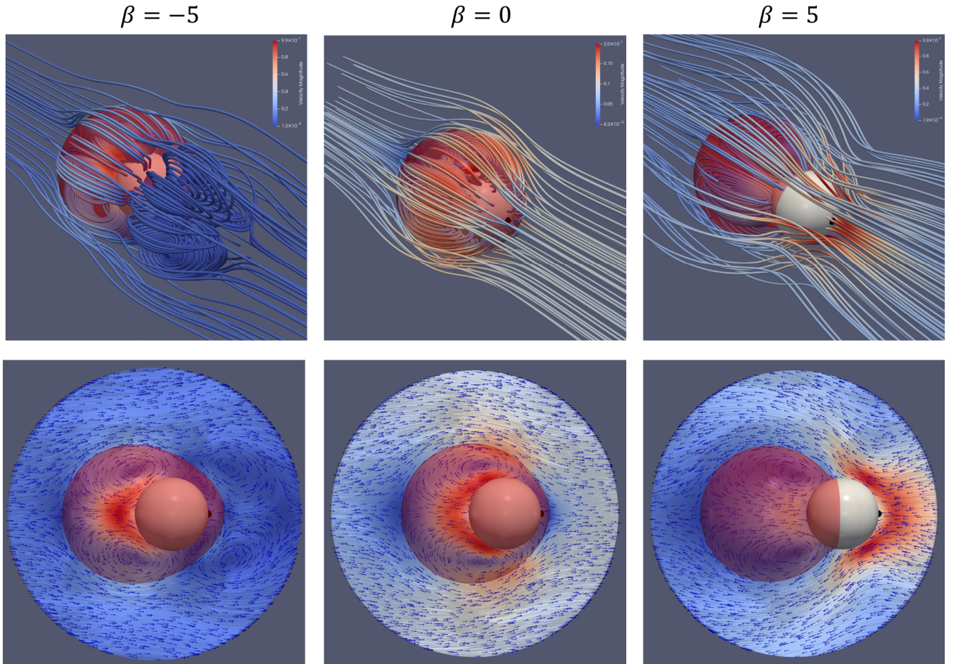
FIG. 13. The streamlines and velocity field for a pusher ( \beta = -5 ), a neutral squirmer ( \beta = 0 ), and a puller ( \beta = 5 ) in multiphase flow in the frame moving with the swimmer.
