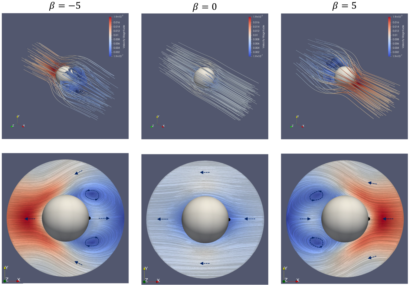
FIG. 4. The streamlines for a pusher ( \beta = -5 ), a neutral squirmer ( \beta = 0 ), and a puller ( \beta = 5 ) in the frame moving with the swimmer. The swimmers swim forward along the x -axis. The upper part shows the streamlines in 3D, and the bottom part shows a slice. The arrows indicate the direction of certain streamlines.
