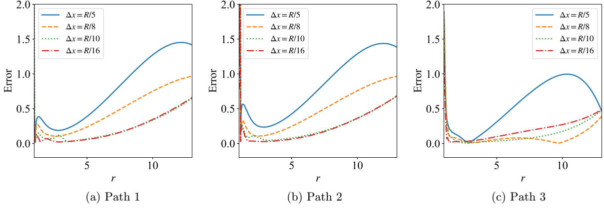
FIG. 15. Relative velocity error along three paths in the flow field at different resolutions.
