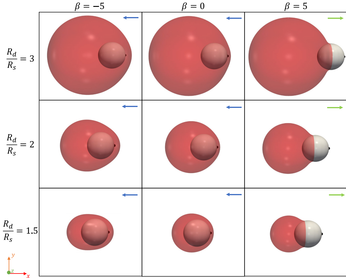
FIG. 11. Types of coswimming motion of different squirmers with different droplet sizes at steady state. The white sphere represent squirmer, the red represents the droplets. The arrows indicate the direction of coswimming of the droplet with the squirmer.
