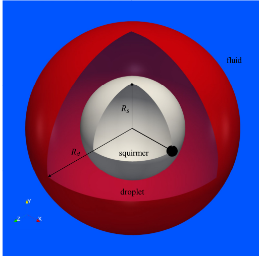
FIG. 10. Initial configuration in multiphase flow. A squirmer (white) with radius R_s is encapsulated by a droplet (red) with a radius R_d . This combination is immersed in a distinct fluid (blue).
