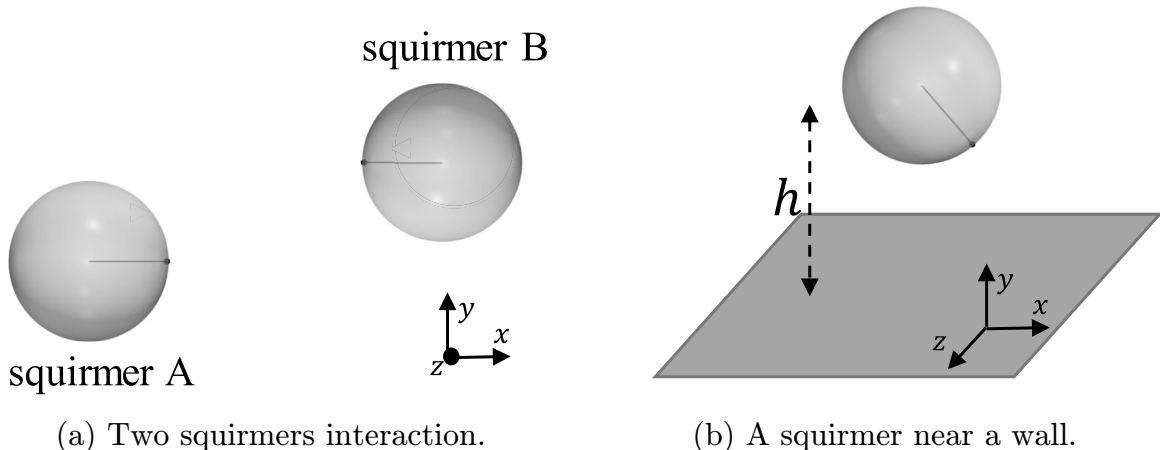
FIG. 6. Schematic of the hydrodynamic interaction of the squirmer(s) at starting point.
