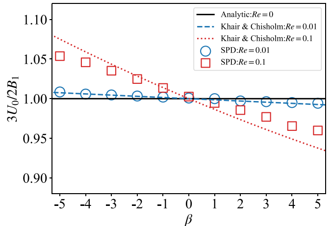
FIG. 3. The velocity magnitude of the squirmer with different \beta . The black line represents the analytical velocity solution at zero Reynolds number. The dashed line results are from Eq. (40) in Khair and Chisholm [63].
