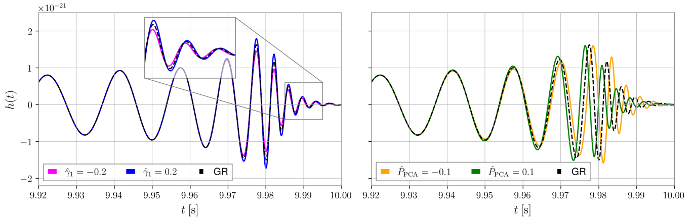
FIG. 1. Left: Comparison of waveforms with \hat{\gamma}_1 = -0.2 (magenta), \hat{\gamma}_1 = 0.2 (blue), and the GR case (black dotted). Since \hat{\gamma}_1 induces additional energy and angular momentum radiation, the remnant mass and spin are modified from the GR prediction, resulting in a change in the QNM frequency. Right: Comparison of waveforms with \hat{P}_{\text{PCA}} = -0.1 (orange), \hat{P}_{\text{PCA}} = 0.1 (green), and the GR case (black dotted). Nonzero values of \hat{P}_{\text{PCA}} introduce phase and time shifts relative to the GR waveform.
