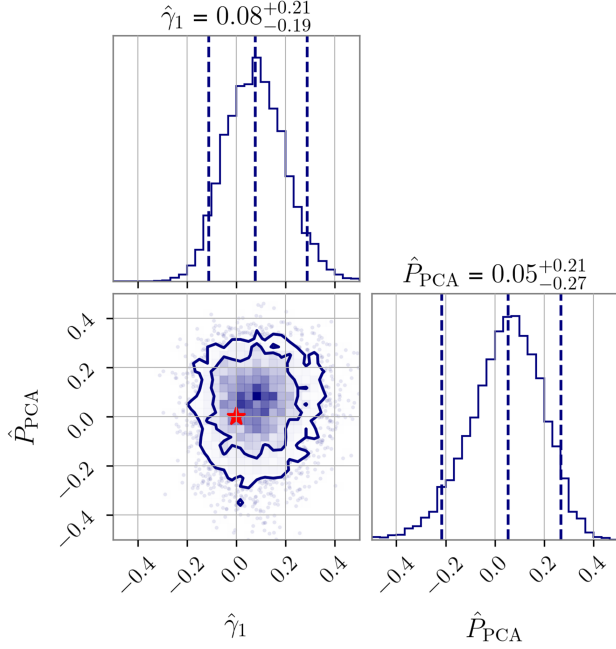
FIG. 6. Posterior probability distributions for \hat{\gamma}_1 and \hat{P}_{\text{PCA}} with GW150914. The dotted lines indicate 90% CL around the mean value. The red star represents (\hat{\gamma}_1, \hat{P}_{\text{PCA}}) = (0, 0) , which means GR. The data is consistent with GR within the 68% error as the contour encloses the star.
