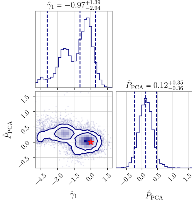
FIG. 9. Same as Fig. 6, but for GW190728.
