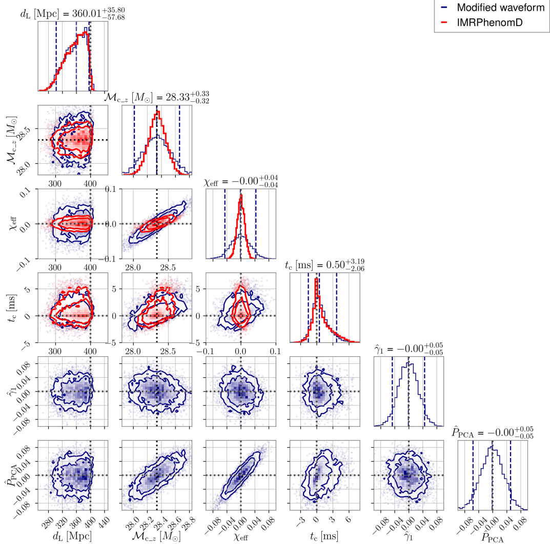
FIG. 2. Posterior probability distributions for \{d_L, \mathcal{M}_{c-z}, \chi_{\text{eff}}, t_c, \hat{\gamma}_1, \hat{P}_{\text{PCA}}\} with a GR injection. The navy and red show the recovery with the modified waveform and the GR waveform. The inner and outer contours indicate 68% and 90% CLs. Black dotted and navy dashed lines show the fiducial values, mean value, and 90% CL, respectively.
