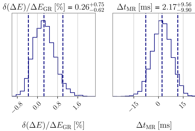
FIG. 7. Updated left: fraction of the additional energy radiation at the merger stage, \delta(\Delta E)/\Delta E_{\text{GR}} , relative to the total GW energy radiation in the IMR process, \Delta E_{\text{GR}} . Right: deviation in the peak time \Delta t_{\text{MR}} induced by \hat{P}_{\text{PCA}} , derived using Eq. (C1). Note that the right panel does not include the intrinsic t_c uncertainty of the GR waveform.
