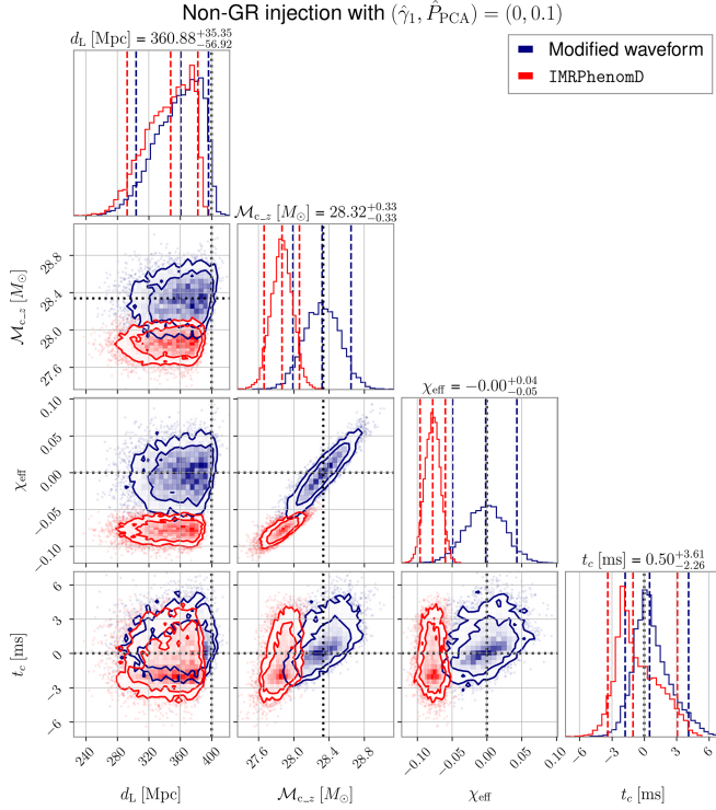
FIG. 5. Same as Fig. 4, but the injection with (\hat{\gamma}_1, \hat{P}_{\text{PCA}}) = (0, 0.1) .
