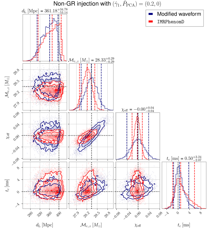
FIG. 4. Posterior probability distributions for \{d_L, \chi_{\text{eff}}, t_c\} with the injection with (\hat{\gamma}_1, \hat{P}_{\text{PCA}}) = (0.2, 0) . The navy and red show the results using the modified and GR waveforms.
