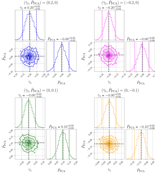
FIG. 3. Posterior probability distributions for \hat{\gamma}_1 and \hat{P}_{\text{PCA}} with the injection with (\hat{\gamma}_1, \hat{P}_{\text{PCA}}) = (0.2, 0) (top left), (-0.2, 0) (top right), (0, 0.1) (bottom left), and (0, -0.1) (bottom right). The colors are identical to those used in Fig. 1.
