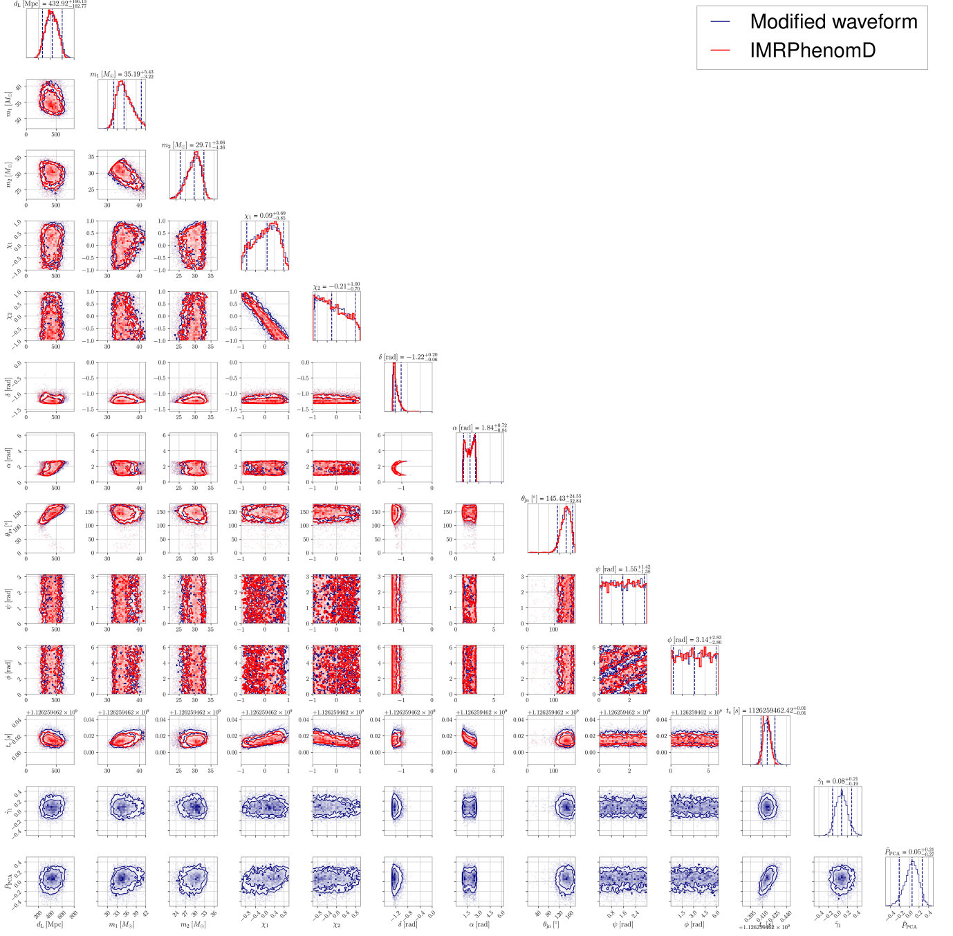
FIG. 8. Full posterior probability distributions for \vec{\theta}_{\text{GR}} (red) and \vec{\theta}_{\text{MG}} (navy) with GW150914. The results for \vec{\theta}_{\text{GR}} agree with Ref. [4]. The results for beyond-GR parameters are consistent with zero within 68% CLs. Figure 6 shows the posterior probability distribution only for the beyond-GR parameters.
