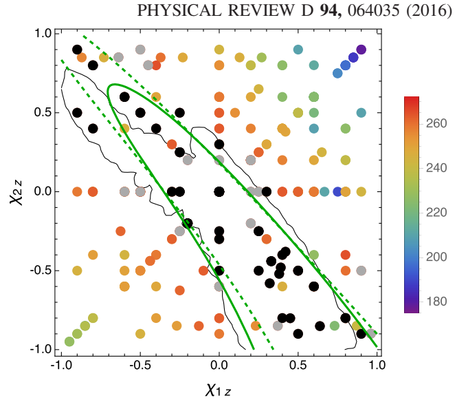
FIG. 7. Aligned spin components not well constrained (aligned only shown) : Colors represent the marginalized log likelihood as a function of the aligned spin components \chi_{1,z} and \chi_{2,z} . Each point represents an NR simulation; only nonprecessing simulations are included. Points with 265.8 < \ln L < 268.6 are shown in light gray, those with \ln L > 268.6 are shown in black, and those with \ln L < 265.8 are shown according to the color scale on the right (points with \ln \mathcal{L}_{\text{marg}} < 172 have been suppressed to increase contrast). [The quantity \ln L is the maximum value of \ln \mathcal{L}_{\text{marg}} with respect to mass; see Eq. (7).] Consistent with our other results, f_{\text{low}} = 30 Hz. For comparison, the solid black contours show the 90% credible intervals derived in LVC-PE [2], assuming spin-orbit alignment and omitting corrections for waveform systematics. The solid and dashed green contours are the nominal 90% credible interval derived using an approximation to our data for \ln \mathcal{L}_{\text{marg}} , assuming both spins are exactly parallel to the orbital angular momentum, for l = 2 (solid) and l = 3 (dashed), respectively; see Sec. IV B for more details.
