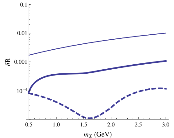
FIG. 5. \delta R for the parameters depicted in Fig. 2.
