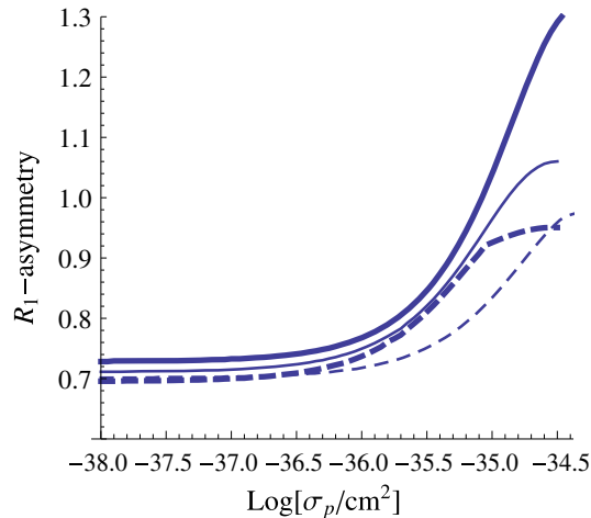
FIG. 3. R_1 asymmetry for the parameters depicted in Fig. 1.
