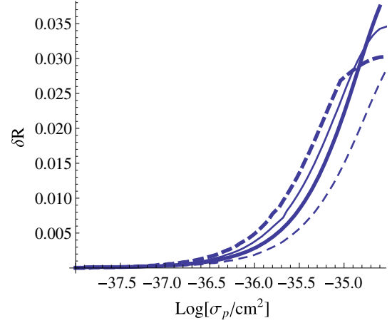
FIG. 4. \delta R for the parameters depicted in Fig. 1.
