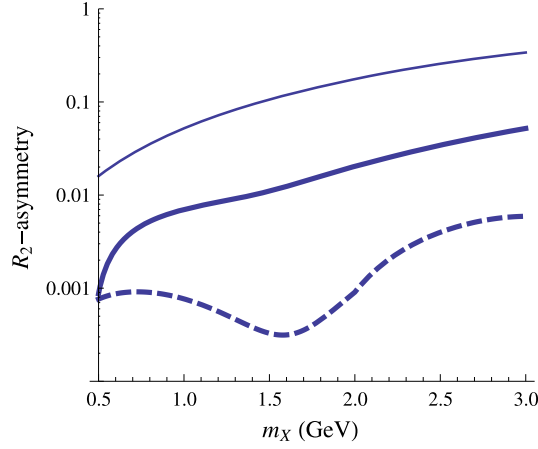
FIG. 2. R_2 asymmetry as a function of DM mass (in GeV) at a recoil energy of 0.1 keV for three values of DM-nucleon cross section 10^{-36} \text{ cm}^2 (thin line), 10^{-37} \text{ cm}^2 (thick line), and 10^{-38} \text{ cm}^2 (dashed line).
