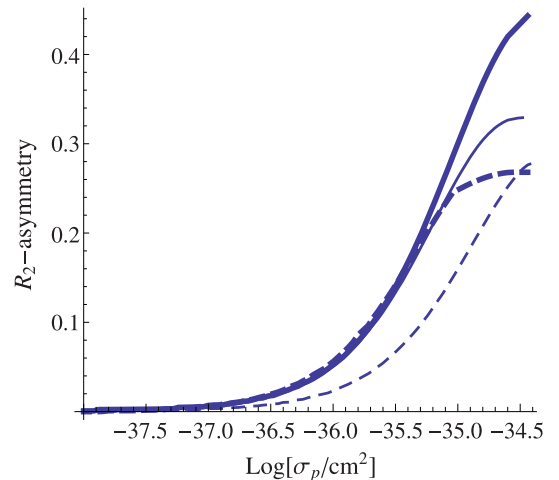
FIG. 1. R_2 asymmetry as a function of the DM-nucleon cross section for a DM particle of mass 1 GeV at recoil energies 0.1 keV (solid thick), 0.2 keV (solid thin), and 0.3 keV (thick dashed line). The thin dashed line corresponds to a 0.6 GeV DM particle with recoil 0.1 keV. We assume a \text{CF}_4 detector.
