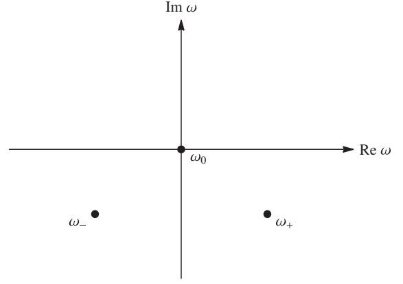
FIG. 1. Shear channel eigenmodes in the zero wave number limit. Shown are the two degenerate hydrodynamic modes at \omega_0 = 0 and the first two nonhydrodynamic modes at \omega_\pm that exhibit transient oscillatory behavior.
