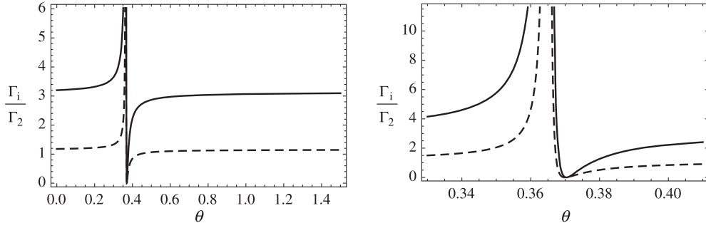
FIG. 2. \Gamma_0/\Gamma_2 (solid) and \Gamma_1/\Gamma_2 (dashed) as a function of \theta .
