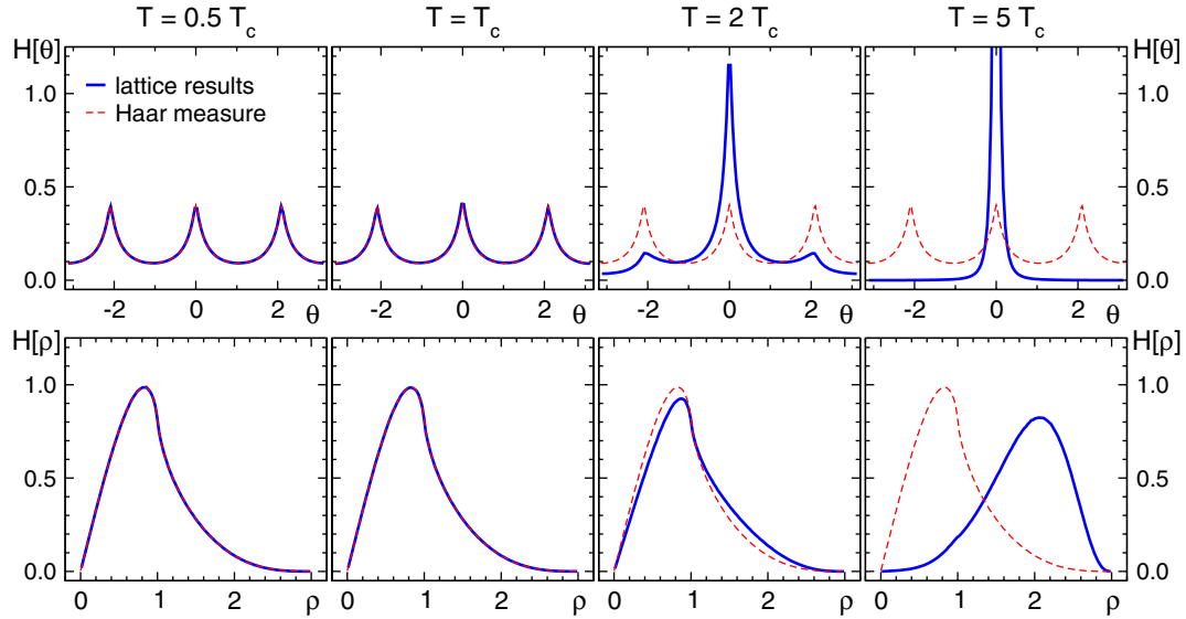
FIG. 3 (color online). Histograms H[\theta] of the phase \theta(x) (top row of plots) and the modulus \rho(x) (bottom) of the local Polyakov loops. We show results for four different temperatures and compare our Monte Carlo results (full curves) to the Haar measure distribution (dashed curves, which up to T_c fall exactly on top of the Monte Carlo data).
