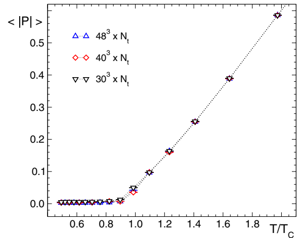
FIG. 1 (color online). The order parameter \langle |P| \rangle as a function of the temperature. The results are for our \beta = 6.2 ensembles.
