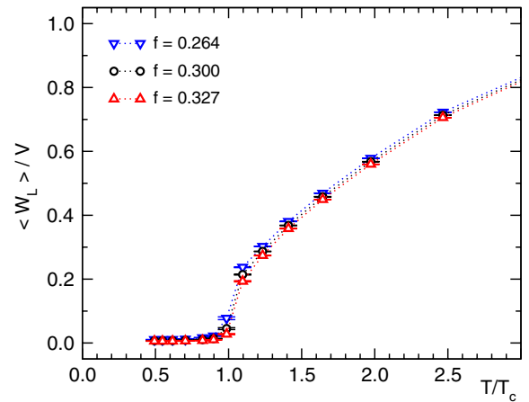
FIG. 6 (color online). Expectation value \langle W_L \rangle / V of the weight of the largest cluster normalized by the 3-volume as a function of the temperature. We show results for \beta = 6.2 , 40^3 \times N_t and compare three different values of the cut parameter f .
