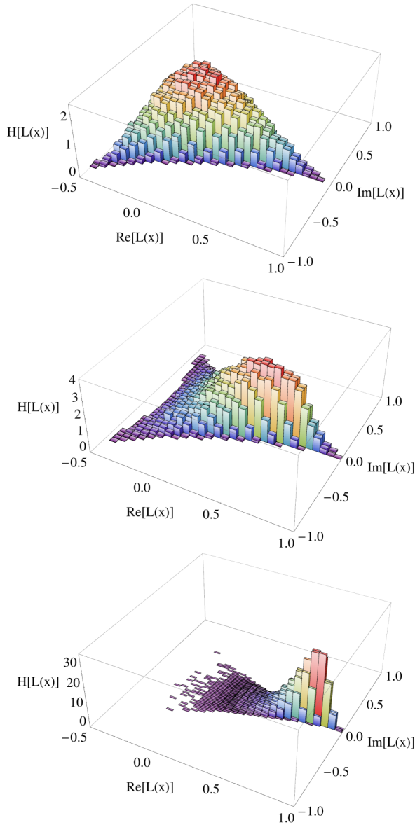
FIG. 2 (color online). Histograms H[L(x)] for the distribution of local Polyakov loop values L(x) in the complex plane. We show the results for 3 configurations from our \beta = 6.2 , 40^3 \times N_t ensembles, corresponding to temperatures T = T_c , T = 2T_c and T = 5T_c (top to bottom).
