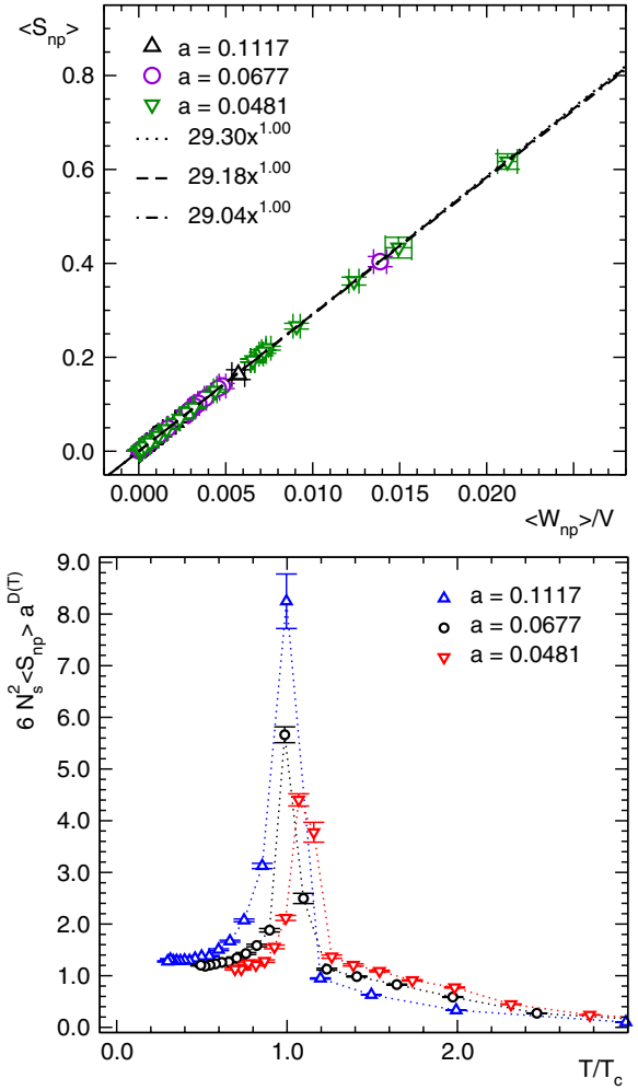
FIG. 18 (color online). Upper panel: Average surface of the nonpercolating clusters versus their average weight. The data are for our 48^3 \times N_t lattices using all N_t and all three values of the lattice constant a . We also show the results of straight line fits of the data. Lower panel: The surface in physical units (for details see the text) as function of the temperature.
