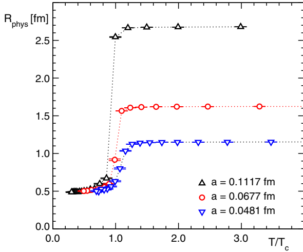
FIG. 10 (color online). Radius of the largest cluster as a function of the temperature. We compare the results from our 48^3 \times N_t lattices for all three values of the lattice constant a .
