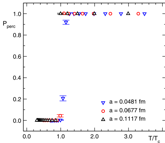
FIG. 11 (color online). The probability P_{\text{perc}} of finding a percolating cluster as a function of the temperature. We use our 48^3 \times N_t ensembles and show results for all three values of the lattice spacing a .
