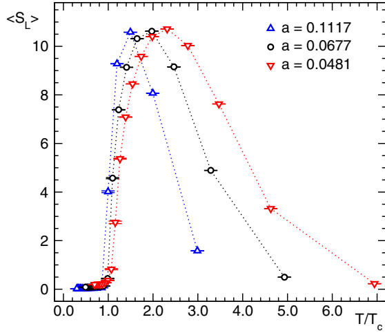
FIG. 17 (color online). Average surface \langle S_L \rangle of the largest cluster as function of the temperature. Results are shown for our 48^3 \times N_t lattices, for all three values of the lattice constant.
