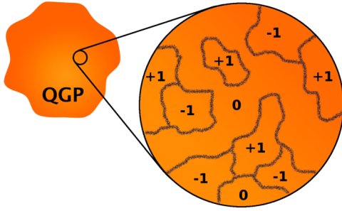
FIG. 19 (color online). Schematic illustration of center clusters slightly above T_c ; figure adapted from Ref. [1].
