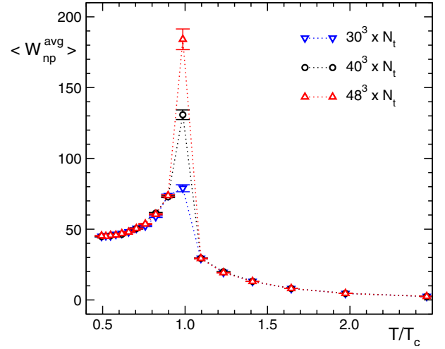
FIG. 8 (color online). Expectation value \langle W_{\text{np}}^{\text{avg}} \rangle of the average weight of nonpercolating clusters as a function of the temperature. The results are for our \beta = 6.2 ensembles with a cut parameter of f = 0.3 and we compare three different spatial volumes V = 30^3 , V = 40^3 and V = 48^3 .
