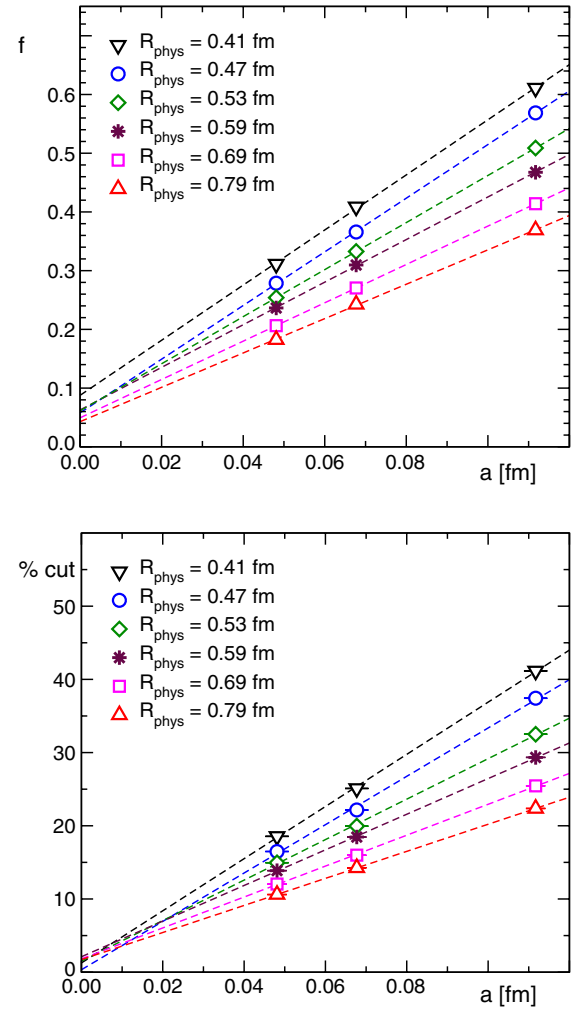
FIG. 9 (color online). Dependence of the cut on the lattice constant a . In the top panel we show the cut parameter f(a, R_{\text{phys}}) that is necessary to obtain a given R_{\text{phys}} of the largest clusters for several values of R_{\text{phys}} . In the bottom plot we show the corresponding percentage of sites that has to be cut. Both plots are for our 48^3 \times 20 lattices, i.e., the lowest temperatures we consider.
