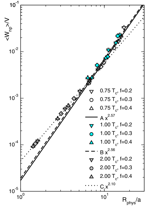
FIG. 16 (color online). Weight of the largest nonpercolating cluster against its radius for three representative values of the temperature. Results are shown for various values of f and the lattice spacing, as measured on our 48^3 \times N_t lattices. The lines indicate fits for the scaling dimension as described in the text.
