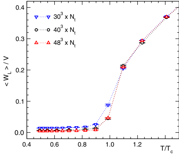
FIG. 7 (color online). Expectation value \langle W_L \rangle / V of the weight of the largest cluster normalized by the 3-volume as a function of the temperature. The results are for our \beta = 6.2 ensembles with a cut parameter of f = 0.3 and we compare three different spatial volumes V = 30^3 , V = 40^3 and V = 48^3 .
