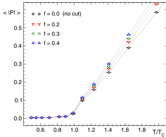
FIG. 5 (color online). Influence of the cut parameter f on the order parameter \langle |P| \rangle as a function of the temperature. The results are for our \beta = 6.2 , 40^3 \times N_t ensembles.
