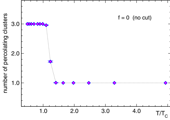
FIG. 4 (color online). The number of percolating clusters for cut parameter f = 0 (no cut) as a function of the temperature. The results are for our \beta = 6.2 , 40^3 \times N_t ensembles.
