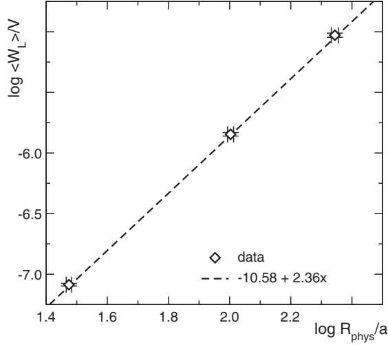
FIG. 15. Logarithm of the weight of the largest cluster on our 48^3 \times 20 lattices versus the logarithm of its radius for the three different lattice spacings. The data (symbols) are fit with a straight line (dashed).
