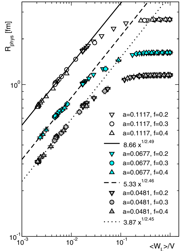
FIG. 14 (color online). Radius of the largest cluster against its weight. We show the results for different values of f and compare all three lattice spacings on our 48^3 \times N_t lattices. In the plot we also show the results of fits of the asymptotic behavior at small \langle W_L \rangle with a power law R_{\text{phys}} \propto \langle W_L \rangle^{1/D_{\text{sc}}} .
