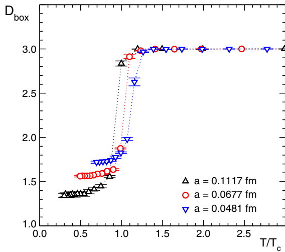
FIG. 13 (color online). The fractal dimension from the box-counting method as a function of the temperature. We show results for our 48^3 \times N_t lattices for all three lattice spacings.
