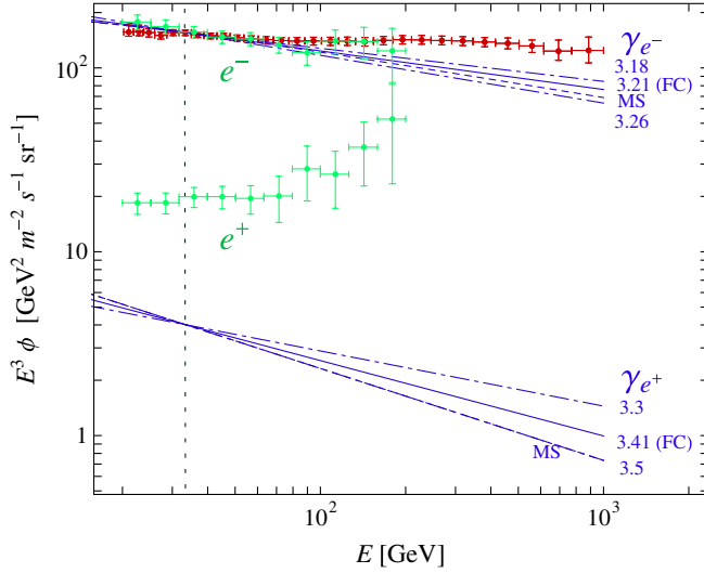
FIG. 1 (color online). Models for background fluxes: MS (dashed line), and SI for extreme (dot-dashed line) and intermediate (solid line) values of the spectral indices. The latter corresponds to the FC model. The fluxes have been normalized by choosing N_{e^\pm}^B = 0.73 . The Fermi-LAT experimental data on the total flux [5] (upper) and separate electron and positron fluxes [6] are also shown for comparison.
