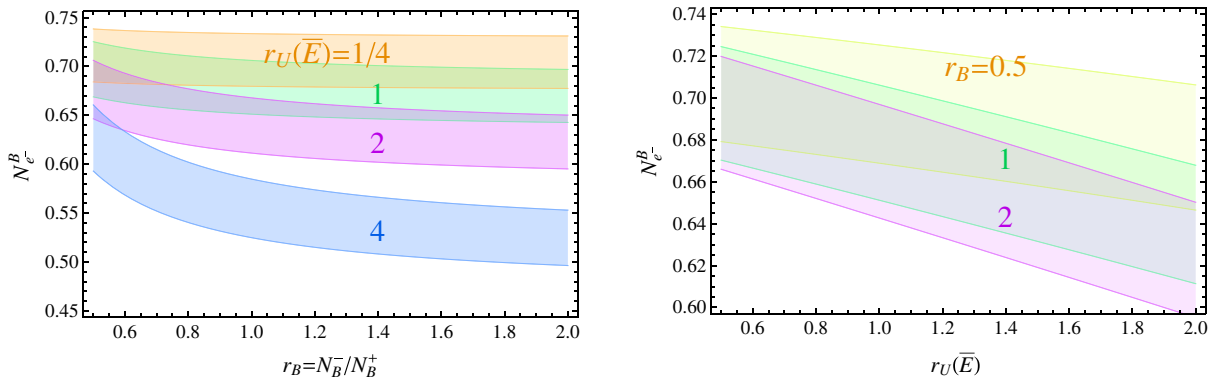
FIG. 2 (color online). Values of N_{e^-}^B according to Eq. (10) assuming \bar{E} = 33.35 GeV. Left panel: as a function of r_B for different values of r_U(\bar{E}) . Right panel: as a function of r_U(\bar{E}) for different values of r_B . The thickness of the bands is obtained by considering the 1\sigma ranges of F_+(\bar{E}) from AMS-02 [4] and T(\bar{E}) from Fermi-LAT [5].
