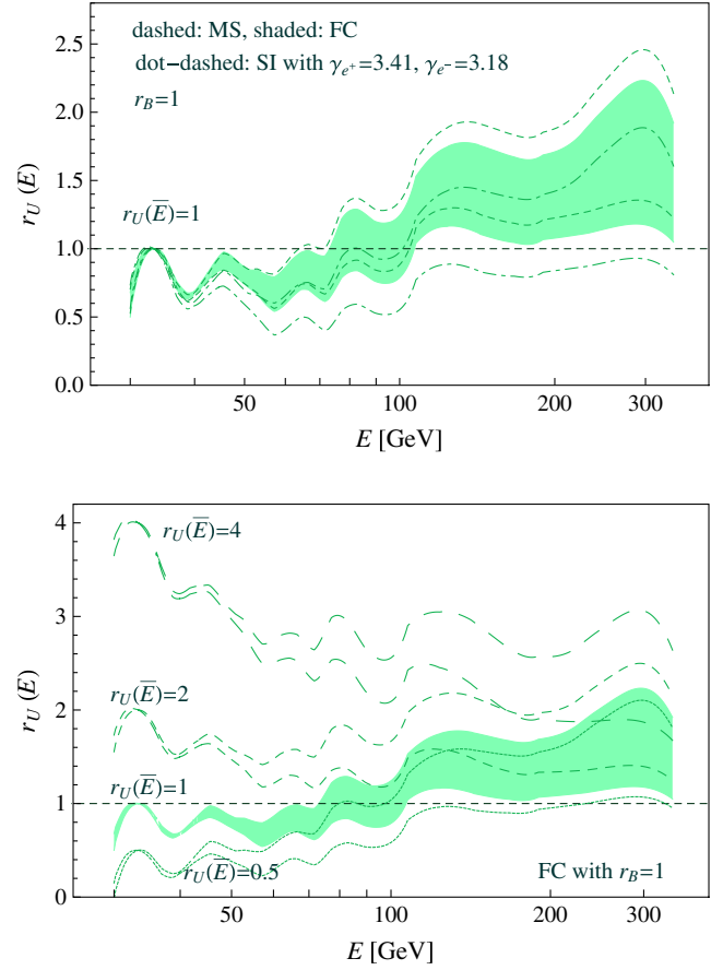
FIG. 5 (color online). Ratio r_U(E) according to Eq. (15). Top panel: For the MS (dashed), FC (shaded) and SI (dot-dashed) models with r_B = 1 and r_U(\bar{E}) = 1 . Bottom panel: For the FC model with r_B = 1 and various values of r_U(\bar{E}) . The thickness of the curves corresponds to the 1\sigma ranges of AMS-02 [4] and Fermi-LAT [5].
