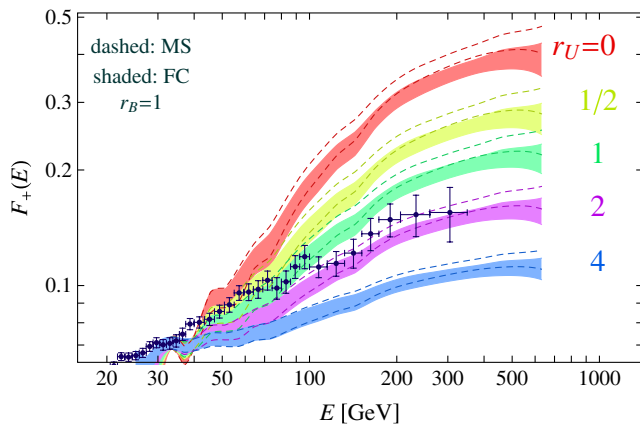
FIG. 3 (color online). Positron fraction F_+(E) for different values of r_U , according to Eq. (11). The shaded (dashed) curves refer to the FC (MS) background model with r_B = 1 . The AMS-02 data [4] with 1\sigma error bars (statistical and systematic combined in quadrature) are shown for comparison.
