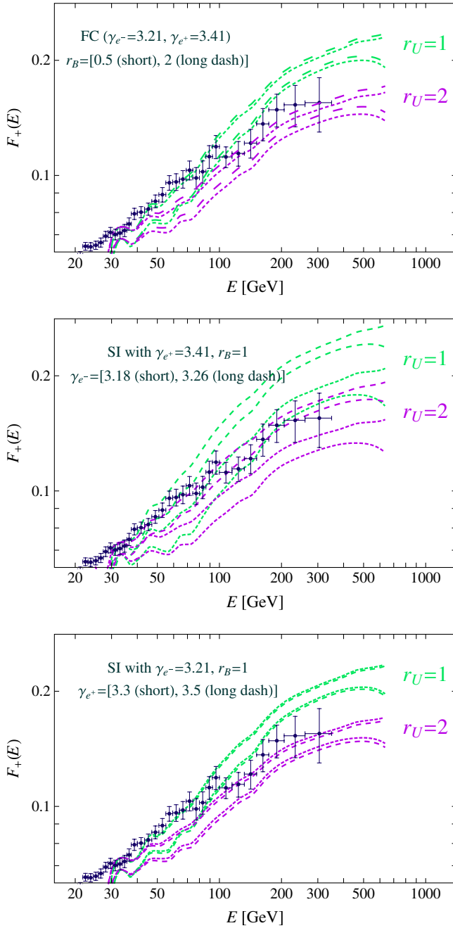
FIG. 4 (color online). Positron fraction F_+(E) for different values of r_U . The AMS-02 data [4] with 1\sigma error bars are shown for comparison. Top panel: Dependence on r_B for the FC model. Middle panel: Dependence on \gamma_{e^-} for the SI model with \gamma_{e^+} = 3.41 and r_B = 1 . Bottom panel: Dependence on \gamma_{e^+} for the SI model with \gamma_{e^-} = 3.21 and r_B = 1 .
