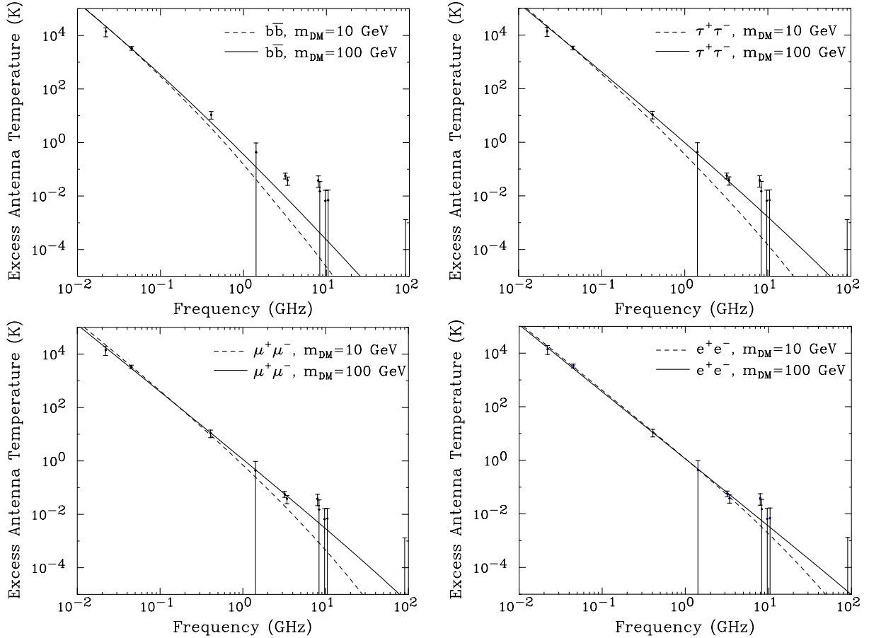
FIG. 3 (color online). The contribution to the isotropic radio background from annihilating dark matter particles with masses of 10 or 100 GeV, and annihilating to b\bar{b} , \tau^+\tau^- , \mu^+\mu^- , or e^+e^- . In each case, we have used our default magnetic field models and dark matter distributions, and substructure as favored by the Via Lactea simulation (see Sec. II). In each case, the annihilation cross section was selected to best fit the observed radio excess. In the case of annihilations to b\bar{b} , we find a very poor fit to the observed spectrum, corresponding to \chi^2 = 44.2 and 34.7 for 10 and 100 GeV masses, respectively, over 12 degrees of freedom. We find similarly poor fits for annihilations to other hadronic final states, and for annihilations to gauge or Higgs bosons. Other choices of the magnetic field and substructure models do not significantly alter this conclusion. In contrast, annihilations to leptonic final states can provide a good fit to the spectrum of the observed excess. Annihilations of a 10 GeV dark matter particle to taus, muons, or electrons yield a \chi^2 of 36.0, 24.8, and 12.3, respectively. For a 100 GeV mass, these channels yield a \chi^2 of 14.4, 12.1, and 13.1. The quality of these fits can change somewhat with variations of the magnetic field model, although realistic models universally favor leptonic annihilation channels.
