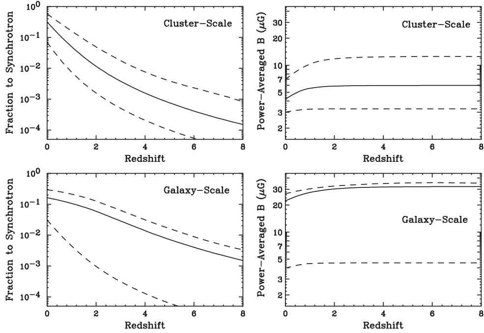
FIG. 2. The fraction of energy in electron/positron dark matter annihilation products which is lost to synchrotron emission (left) and the power-averaged magnetic field strength which contributes to that synchrotron emission (right). In the upper and lower frames, we show results for our models for the largest dark matter halos ( M > 10^{13} M_\odot ) and somewhat smaller halos ( 10^{10}-10^{13} M_\odot ), respectively. In each frame, the solid lines denote the results for our default magnetic field and dark matter distribution models. The dashed lines represent the range of values found using the variety of models described in Sec. IV. In each case shown, we use the Via Lactea substructure model.
