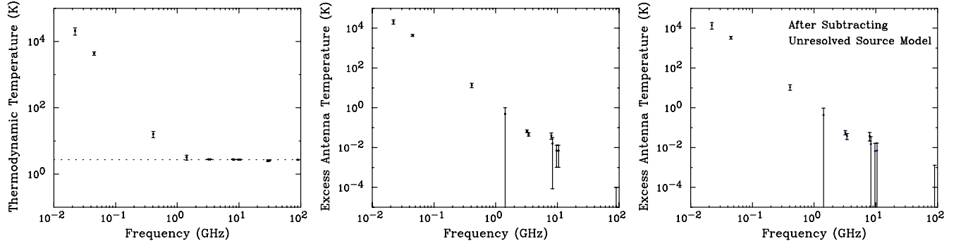
FIG. 1 (color online). Measurements of the isotropic radio background, as reported by Roger et al. (0.022 GHz) [3], Guzman et al. (0.045 GHz) [4], Haslam et al. (0.408 GHz) [5], Reich and Reich (1.42 GHz) [6], and by the ARCADE-2 Collaboration (3.20 to 90 GHz) [1] (see also, Ref. [2]). In the left frame, the total observed background is shown, including the contribution of the CMB (shown as a dotted line). In the middle frame, the CMB has been subtracted, revealing a power-law spectrum of isotropic emission. In the right frame, an estimate of the contribution from unresolved radio sources has been subtracted as well. See text for more details.
