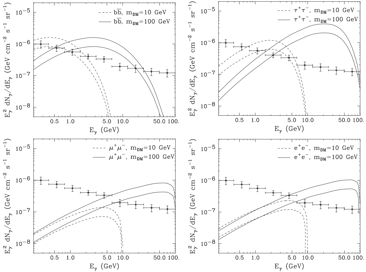
FIG. 4. The contribution to the isotropic gamma-ray background from annihilating dark matter, in the same models as shown in Fig. 3. In each case, the upper curve use an extrapolation to determine the concentration of halos lighter than 10^5 M_\odot , whereas the lower curve fixes the concentration below this mass. When these contributions are compared to the isotropic gamma-ray background observed by Fermi, we see that annihilations of heavy ( m_{\text{DM}} \gg 10 GeV) dark matter particles, or dark matter particles which annihilate primarily to hadronic or \tau^+\tau^- channels, are unable to produce the observed radio background without also exceeding the observed gamma-ray spectrum.
