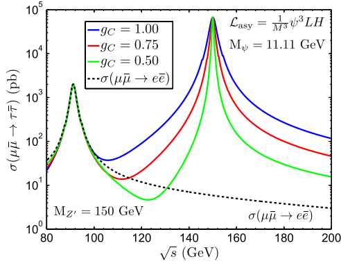
FIG. 4 (color online). An exhibition of the relative strength of the \tau^+\tau^- vs e^+e^- signal at a muon collider. The presence of a detectable Z' resonance in the \mu^+\mu^- \rightarrow \tau^+\tau^- channel provides a smoking gun signature for the gauged L_\mu - L_\tau AsyDM model. A similar resonance is also present in the \mu^+\mu^- \rightarrow \mu^+\mu^- channel while \mu^+\mu^- \rightarrow e^+e^- cross section shows no such enhancement in the Z' region.
