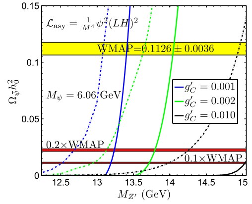
FIG. 5 (color online). A display of the thermal relic density of \psi as a function of M_{Z'} for the model with a gauged B - L for different couplings with \gamma = 0 (dashed line) and \gamma = \gamma_0 = 1.3 \times 10^{-10} (solid line). It is seen that resonant annihilation of thermal dark matter via the Z' pole allows the relic density of this component to be reduced to below 10% of the WMAP value for values of Z' around twice the mass of the dark particle.
