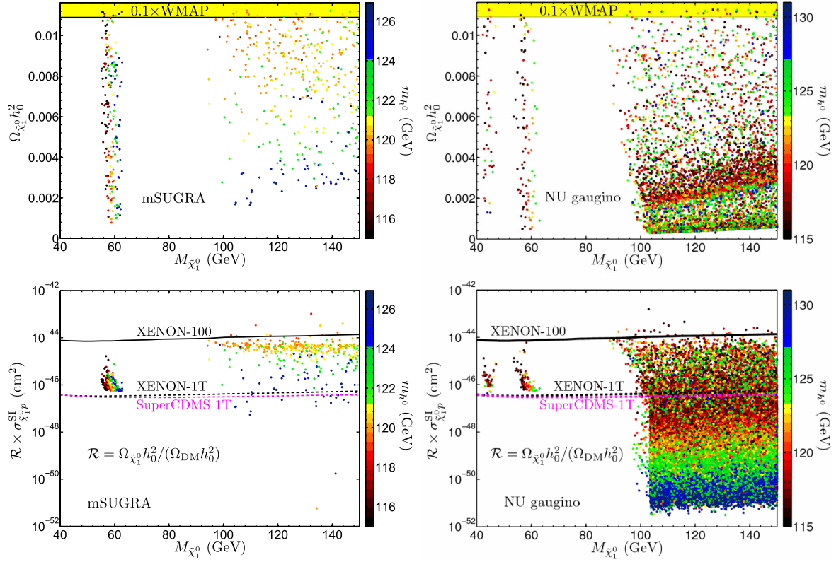
FIG. 2 (color online). Top panel: An exhibition of the depletion of the MSSM neutralino dark matter below 10% of the WMAP relic density for cold dark matter. Parameter points are displayed by their light CP -even Higgs mass and the yellow band corresponds to 10% of the WMAP-7 observed limit. Bottom panel: An exhibition of the neutralino-proton spin-independent cross section as a function of the neutralino mass. To account for the reduced relic density of the neutralino component of dark matter, the spin-independent cross section has been corrected by a factor \mathcal{R} = \Omega_{\tilde{\chi}_1^0} h_0^2 / (\Omega_{\text{DM}} h_0^2) . The present experimental limits (solid line) [52] as well as the future projections (dashed lines) are shown [53,54]. The left panel shows the parameter points of mSUGRA and the right panel shows the nonuniversal gaugino parameter points. All parameter points shown pass the general constraints.
