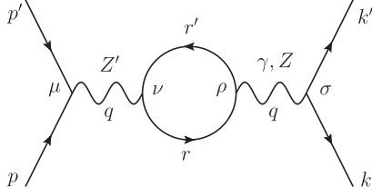
FIG. 7. Z' - \gamma and Z' - Z exchange via \mu^+ \mu^- , \nu_\mu \bar{\nu}_\mu , \tau^+ \tau^- , \nu_\tau \bar{\nu}_\tau loops.
