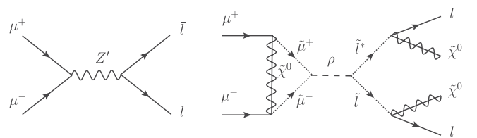
FIG. 3. Left: Leptonic final states in a \mu^+ \mu^- collider where the \mu^+ \mu^- \rightarrow \bar{l} l , with l = \mu, \nu_\mu, \tau, \nu_\tau , final state arising from direct channel poles involving Z' . The Z' pole does not allow for a e^+ e^- final state and thus the relative production cross section for \mu^+ \mu^- \rightarrow \tau^+ \tau^- vs \mu^+ \mu^- \rightarrow e^+ e^- can be used to detect the existence of a L_\mu - L_\tau gauged boson. Right: A similar analysis is possible for \rho but its production is suppressed relative to Z' since it must be produced at the loop level.
