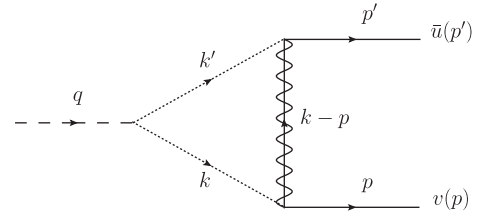
FIG. 6. A generic diagram showing the decay of the \rho to one of the final states which could be \mu^+ \mu^- , \nu_\mu \bar{\nu}_\mu , \tau^+ \tau^- , \nu_\tau \bar{\nu}_\tau via exchange of sleptons, charginos and neutralinos at one loop.
