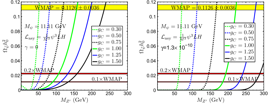
FIG. 1 (color online). An exhibition of the thermal relic density of \bar{\psi} as a function of M_{Z'} in the model with gauged L_\mu - L_\tau for different values of the coupling constant. The left panel shows the case \gamma = 0 and the right panel shows \gamma = 1.3 \times 10^{-10} . In both cases, the analysis shows that the component of dark matter that is thermally produced can be efficiently depleted by resonant annihilation via the Z' pole.
