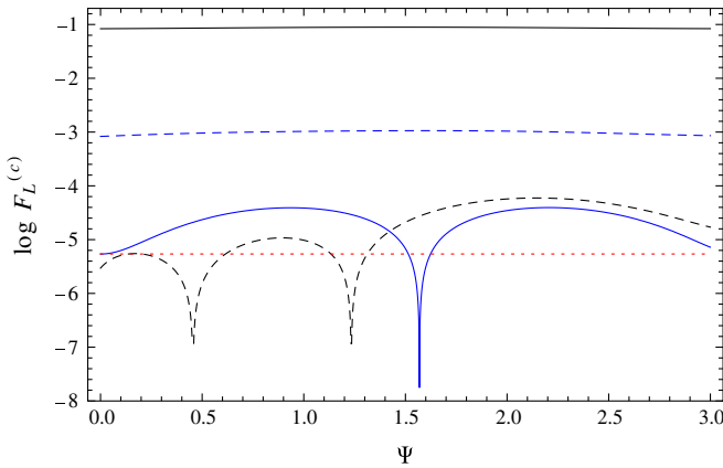
FIG. 1 (color online). F_L^{(c)} for our toy model as a function of the sneutrino left-right mixing angle \Psi and for different values of \kappa : 10^{-4} (blue line), 10^{-2} (black dashed line), 0.1 (blue dashed line), and 1.0 (black line).
