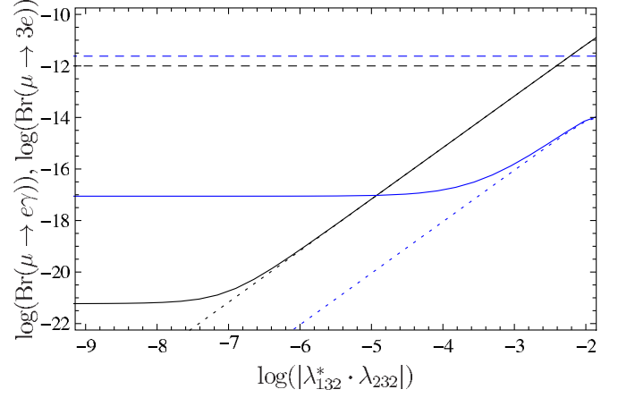
FIG. 3 (color online). \text{Br}(\mu \rightarrow 3e) (black line) and \text{Br}(\mu \rightarrow e\gamma) (blue line) varying \lambda_{132} \cdot \lambda_{232} in a mixed bilinear and trilinear (solid lines) and a pure trilinear (dotted line) RpV scenario. The dashed lines show the experimental limits.
