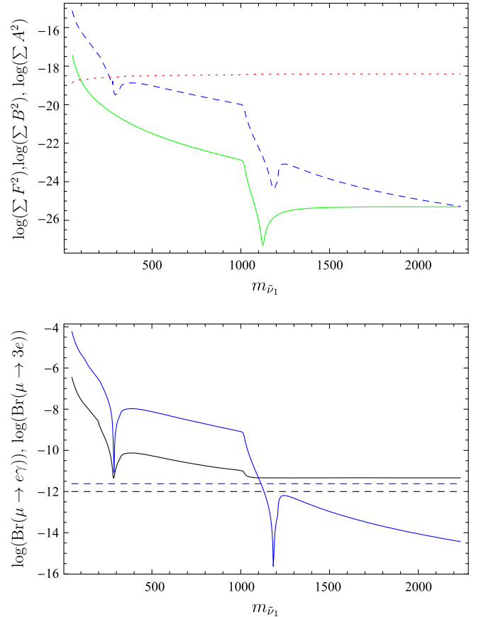
FIG. 2 (color online). Top: Different contributions to \text{Br}(\mu \rightarrow 3e) as function of the lightest sneutrino mass: Z^0 -penguins (red dotted line), photonic penguins (blue dashed line), combined Higgs-penguins/box diagrams (green line). Bottom: \text{Br}(\mu \rightarrow 3e) (black line) and \text{Br}(\mu \rightarrow e\gamma) (blue line) and the current experimental bounds (dashed lines). The dips are an effect of a mass crossing between charginos and sneutrinos.
