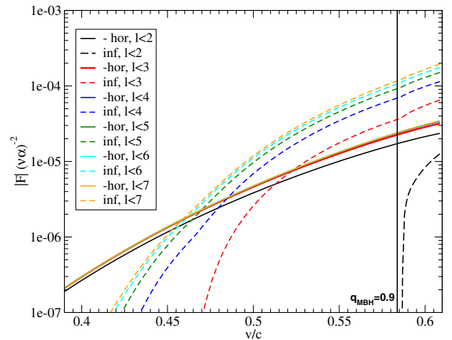
FIG. 5 (color online). Scalar energy flux, normalized by (\alpha\nu)^2 , carried to infinity and into the supermassive black hole horizon as a function of the velocity for \mu_s M_{\text{MBH}} = 0.2 and q_{\text{MBH}} = 0.9 . Different curves are obtained by truncating the series in Eq. (46) at different values of l . Observe that below a certain velocity, \nu \lesssim 0.4 , the contribution to infinity vanishes in accordance with Eq. (54). The resonance corresponding to l = m = 1 is also shown.
