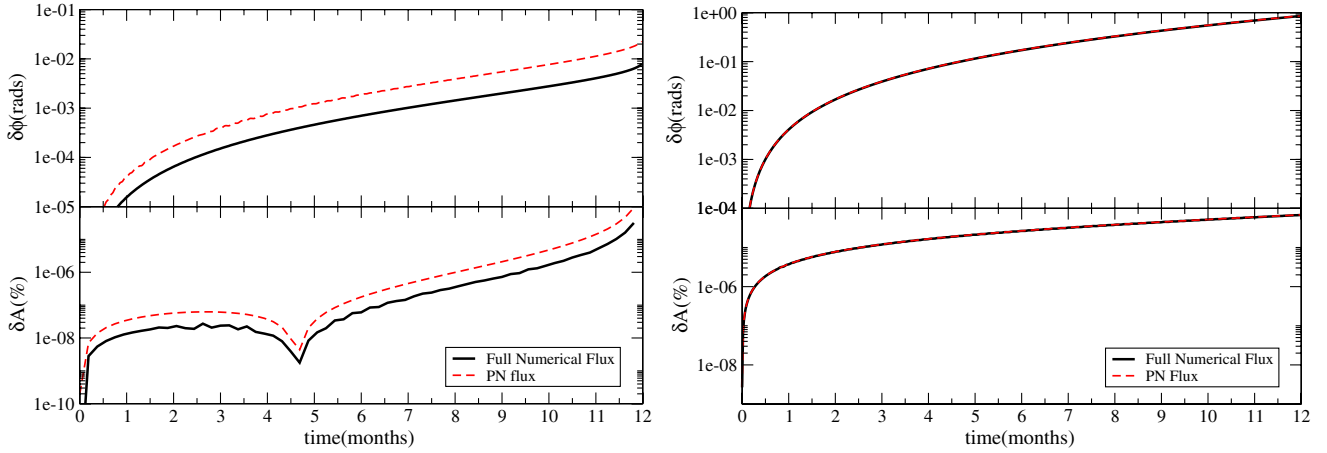
FIG. 6 (color online). Dephasing and normalized amplitude difference as a function of time in units of months for system F (left panel) and system R (right panel). The black and red curves are obtained by using the numerical fluxes constructed in Sec. III and their PN approximation in Eq. (44), respectively. We consider a Brans-Dicke parameter which saturates the Solar System bound, \omega_{\text{BD}} = 4 \times 10^4 .
