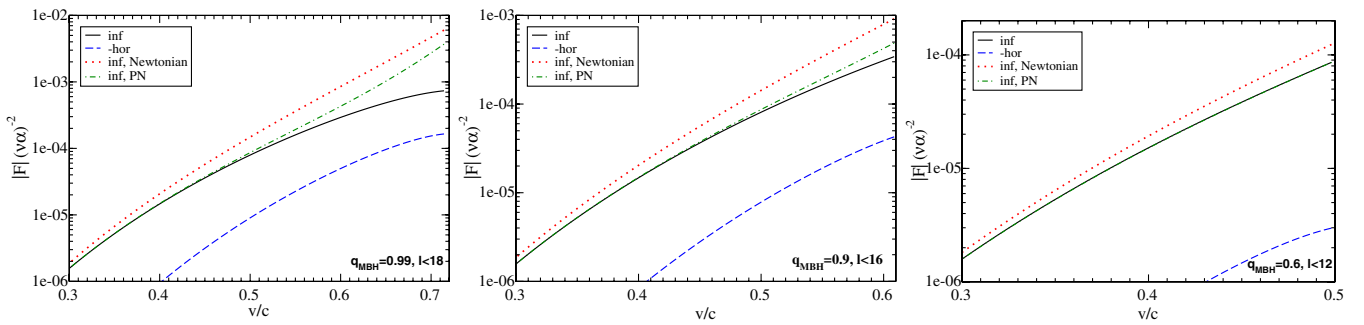
FIG. 3 (color online). Scalar flux at infinity (black solid curve) and at the horizon (blue dashed curve) for a generic massless scalar-tensor theory, normalized by (\alpha v)^2 as functions of the velocity v for \mu_s = 0 , q_{\text{MBH}} = 0.99 (left panel), q_{\text{MBH}} = 0.9 (middle panel), and q_{\text{MBH}} = 0.6 (right panel). For comparison, we show the PN formula (44) (green dot-dashed line) and its truncation at -1 PN order (red dotted line).
