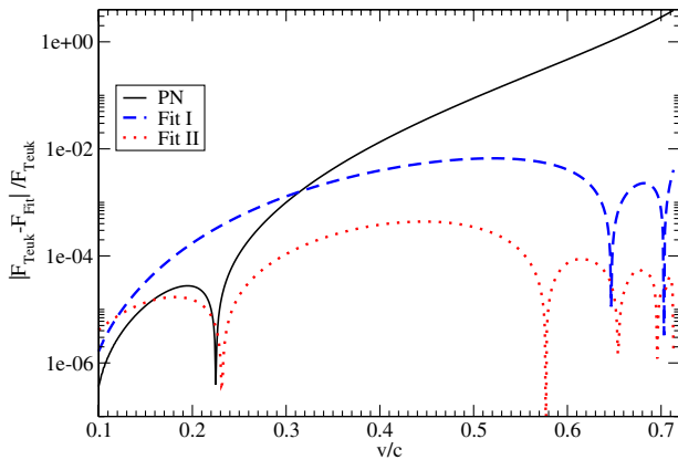
FIG. 4 (color online). Fractional difference between the fits, \mathcal{F}_{\infty}^{s, \text{massless}} , with parameters from Table I and Teukolsky-based fluxes, \mathcal{F}_{\text{Teuk}} , as a function of velocity for spin q_{\text{MBH}} = 0.99 and compared with the fractional difference with the PN flux (44). These curves are an upper bound of the fit error: the fractional difference for fit I, fit II, and for the PN formula decreases for smaller values of q_{\text{MBH}} .
