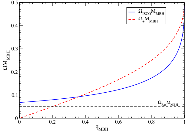
FIG. 7 (color online). The ISCO frequency and angular velocity at the horizon as functions of the spin parameter for a Kerr black hole. In massive scalar-tensor theories, resonances occur for particles in circular orbits at \Omega_{\text{orb}} \sim \mu_s + \mathcal{O}(\mu_s^2) . The stability of the orbit implies \Omega_{\text{orb}} < \Omega_{\text{ISCO}} ; i.e. the relevant region is below the blue line. For q_{\text{MBH}} \geq 0.36 , these frequencies always satisfy the superradiant condition for m = 1 , \Omega_{\text{orb}} < \Omega_+ . For q_{\text{MBH}} \leq 0.36 , the resonant frequency may also be nonsuperradiant in the region limited by the blue line and the red dashed line. Note that resonances may occur even for Schwarzschild black holes.
