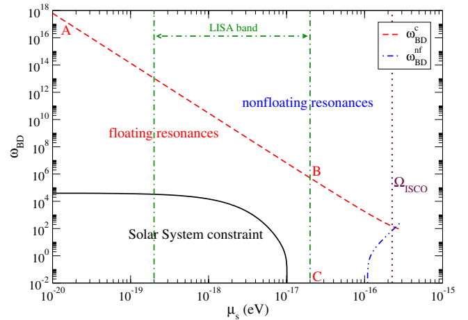
FIG. 1 (color online). Parameter space of massive Brans-Dicke theory for a quasicircular EMRI with typical neutron star sensitivity s_{\text{SCO}} = 0.188 , supermassive black hole spin a_{\text{MBH}}/M_{\text{MBH}} = 0.9 , and mass M_{\text{MBH}} = 10^5 M_\odot . The red dashed curve is the boundary of the region in (\omega_{\text{BD}}, \mu_s) space that separates floating and nonfloating resonances [cf. Eq. (69)]. The area below the black curve shows the region that is ruled out by Solar System experiments [38,54]. The area between the green dot-dashed curves shows the region where a resonance would occur inside the classic-LISA sensitivity band [(10^{-4}, 10^{-2}) \text{ Hz}] . Because of a large dephasing introduced by floating resonances, any detection of an EMRI in a LISA-like mission would rule out the (open) region delimited by ABC. The dot-dashed blue line shows the values of (\omega_{\text{BD}}, \mu_s) below which nonfloating resonances lead to dephasings larger than 1 rad (see Sec. VII C). The ISCO frequency \Omega_{\text{ISCO}} is shown by a vertical dotted line. The curves \omega_{\text{BD}}^{\text{c}} and \omega_{\text{BD}}^{\text{nf}} terminate at \mu_s \sim \Omega_{\text{orb}} \sim \Omega_{\text{ISCO}} \sim 0.22/M_{\text{MBH}} .
