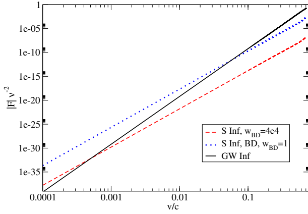
FIG. 2 (color online). PN expansion of the ( v^2 -normalized) gravitational-wave energy flux (black solid curve) and the scalar energy flux carried out to infinity for Brans-Dicke theory with \omega_{\text{BD}} = 4 \times 10^4 (dashed red curve) and \omega_{\text{BD}} = 1 (dotted blue curve) as a function of velocity for a supermassive black hole with spin q = 0.99 and a small compact object with s_{\text{SCO}} = 0.188 . Observe that the scalar flux dominates over the GR one at sufficiently small velocities.
