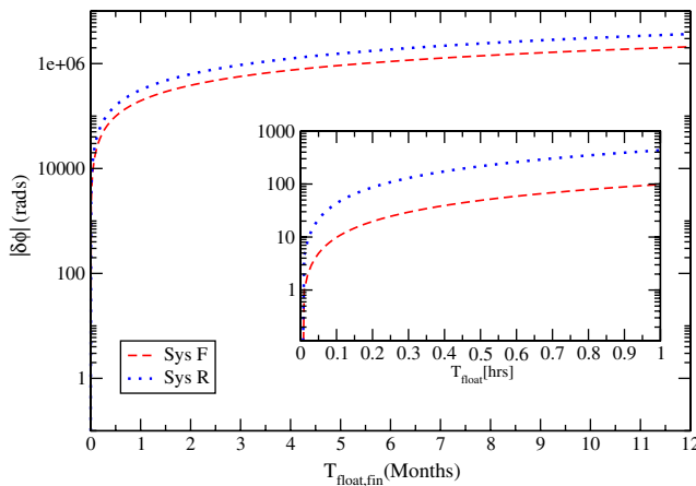
FIG. 9 (color online). Dephasing in radians for systems F and R as a function of the floating time T_{\text{float,fin}} , which can be mapped to \mu_s via Eq. (121).
