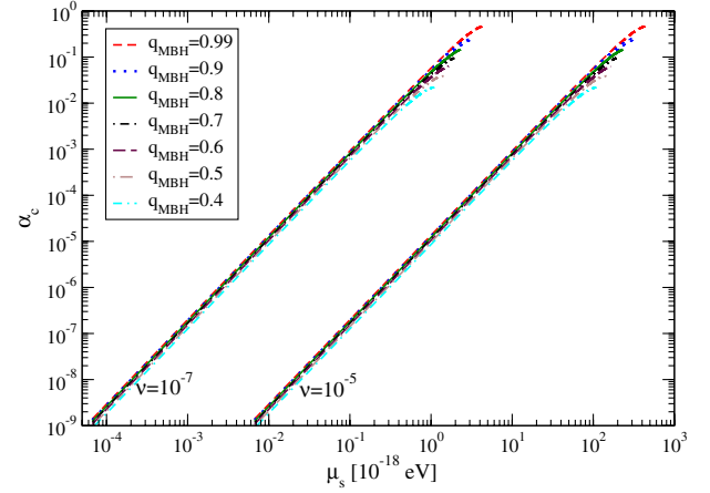
FIG. 8 (color online). The critical value \alpha_c as a function of the scalar mass \mu_s , for several values of q_{\text{MBH}} and for M_{\text{MBH}} = 10^5 M_\odot (lower curves) and M_{\text{MBH}} = 10^7 M_\odot (upper curves). The floating orbit exists for those values of \alpha above the curves and for q \geq 0.36 . Curves terminate when \mu_s \sim \Omega_{\text{ISCO}} .
