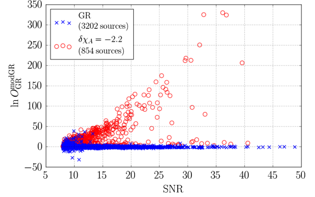
FIG. 13 (color online). The log odds ratios for individual sources for injections with an anomalous frequency dependence in the phase. The blue crosses represent GR injections, while the red circles are for signals that have a contribution to the phase with a frequency dependence in between that of the 1PN and 1.5PN terms (1.25PN). As with the \delta\chi_3 = 0.1 example, a separation between the two is visible for \text{SNR} \gtrsim 10 and becomes more pronounced as the SNR increases.
