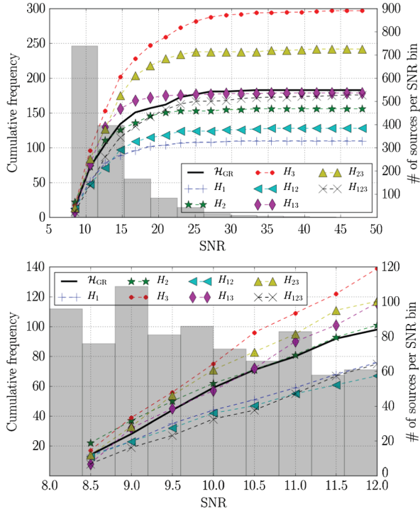
FIG. 6 (color online). Top panel. Curves and left vertical axis: For a given SNR, the cumulative number of times that the Bayes factor against noise for a particular component hypothesis is the largest for injections with that SNR or below, for \delta\chi_3 = 0.1 . All 1471 simulated sources were used. As expected, B_{\text{noise}}^3 dominates, and Bayes factors for hypotheses that let \psi_3 be non-GR tend to outperform those that do not. The GR model outperforms the one with the largest number of free parameters. Histogram and right vertical axis: The number of sources per SNR bin. Bottom panel: The same as above, but restricting to sources with \text{SNR} < 12 . A similar behavior as for the full set of 1471 sources is observed. Note that, already at SNR close to threshold, the GR hypothesis is more likely to be disfavored.
