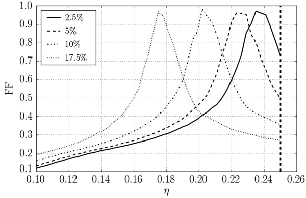
FIG. 3. The fitting factors for a range of \eta , once the other parameters are maximized over. Here a deviation of \psi_3 from 2.5% to 17.5% is used for a (1.4, 1.4)M_\odot system. The vertical dashed line represents the true value of \eta , while the maximum is offset to compensate for the modification in the phase.
