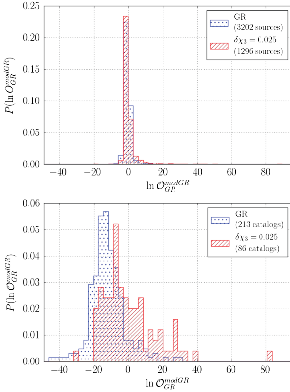
FIG. 8 (color online). Top panel: The normalized distribution P(\ln O_{GR}^{\text{modGR}}) of log odds ratios for individual sources, where the injections are either GR or have \delta\chi_3 = 0.025 . Bottom panel: The normalized distribution P(\ln O_{GR}^{\text{modGR}}) of logs of the combined odds ratios for GR injections and injections with \delta\chi_3 = 0.025 , for catalogs of 15 sources each. For individual sources, the two distributions essentially lie on top of each other. However, when sources are combined into catalogs, it is possible for an outlier to boost the odds ratio of the entire catalog.
