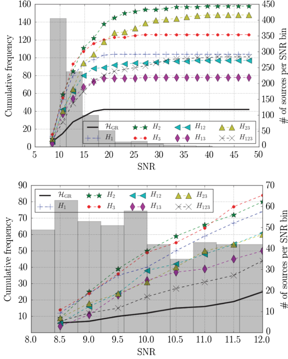
FIG. 15 (color online). Top panel. Curves and left vertical axis: The cumulative number of times that the Bayes factor against noise for a particular component hypothesis is the largest, with increasing SNR, for individual sources with \delta\chi_A = -2.2 . All 854 simulated sources were used. Histogram and right vertical axis: The number of sources per SNR bin. Bottom panel: The same as above, but now for sources with SNR < 12 . Close to threshold, no single hypothesis is the dominant one.
