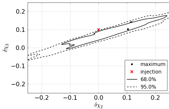
FIG. 20 (color online). The 68% and 95% confidence contours of the two-dimensional PDF for \{\delta\chi_2, \delta\chi_3\} , still for an injection with \delta\chi_3 = 0.1 , and with a waveform that has \{\vec{\theta}, \delta\chi_1, \delta\chi_2, \delta\chi_3\} as free parameters. The maximum of the PDF is given by the black dot, and the injection values are represented by the red cross.
