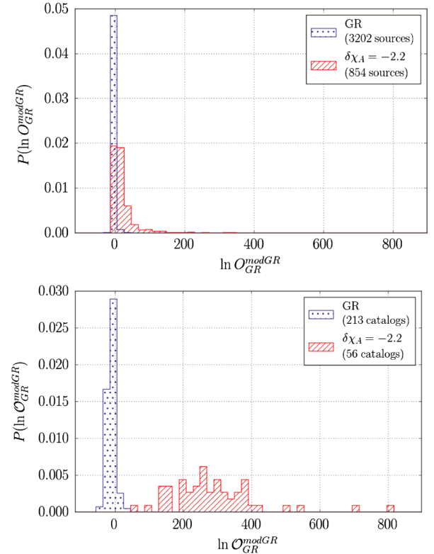
FIG. 14 (color online). Top panel: The normalized distribution P(\ln O_{\text{GR}}^{\text{modGR}}) of log odds ratios for individual sources, where the injections are either GR or have the anomalous frequency dependence. Bottom panel: The normalized distribution P(\ln O_{\text{GR}}^{\text{modGR}}) of logs of the combined odds ratios for GR injections and injections for catalogs of 15 sources each.
