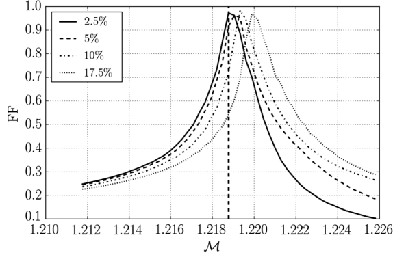
FIG. 2. The fitting factors for a range of \mathcal{M} , once the other parameters are maximized over. Here a deviation of \psi_3 from 2.5% to 17.5% is used for a (1.4, 1.4)M_\odot system. The vertical dashed line represents the true value of \mathcal{M} , while the maximum is offset to compensate for the modification in the phase.
