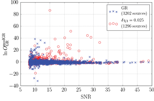
FIG. 7 (color online). The log odds ratios for individual sources. The blue crosses are for signals with standard GR waveforms, and the red circles are for signals with a constant 2.5% relative offset in \psi_3 . This time, there is little separation between the two, although there are outliers for \text{SNR} \approx 15 .
