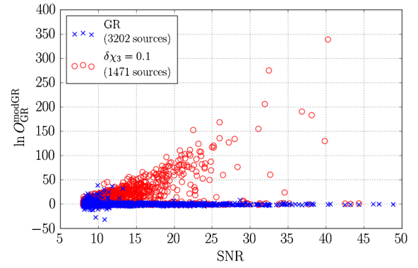
FIG. 4 (color online). The log odds ratios for individual sources. The blue crosses represent signals with standard GR waveforms, the red circles are signals with a constant 10% relative offset in \psi_3 . A separation between the two is visible for \text{SNR} \geq 10 and becomes more pronounced as the SNR increases.
