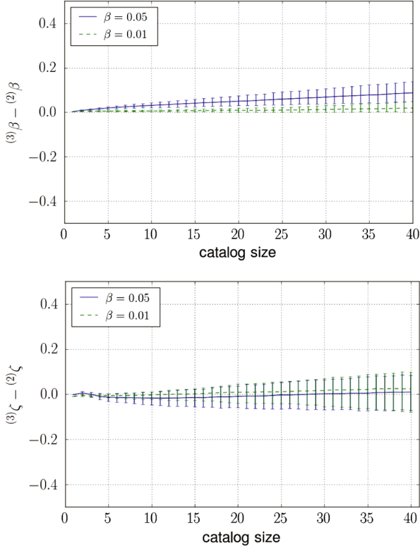
FIG. 11 (color online). Top panel: The change in FAPs in going from two to three testing parameters, but keeping the odds ratio thresholds fixed. Bottom panel: The change in efficiencies when keeping the false alarm probabilities fixed. The plots shown are for the case where the signals have \delta\chi_3 = 0.025 . We see that increasing the number of testing parameters has only a moderate effect on the FAPs, while for fixed FAPs, the efficiencies do not change appreciably. Note, however, that when the evidence for a deviation from GR is marginal, the use of as many hypotheses as possible can be pivotal in finding the violation (see Figs. 9 and 16).
