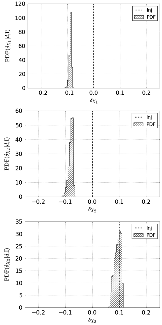
FIG. 18. Posterior PDFs for a single injection with \delta\chi_3 = 0.1 and network SNR of 23.2. Top panel: \delta\chi_1 measured with a waveform that has \{\hat{\theta}, \delta\chi_1\} free. Middle panel: \delta\chi_2 measured with a waveform that has \{\hat{\theta}, \delta\chi_2\} free. Bottom panel: \delta\chi_3 measured with a waveform that has \{\hat{\theta}, \delta\chi_3\} free. As expected, the bottom PDF is sharply peaked at the correct value of \delta\chi_3 = 0.1 , with a standard deviation of 0.012. For the top and middle PDFs, the one test parameter that is used differs from the parameter in the signal that has the shift. The parameters in the waveform will rearrange themselves such as to best accommodate the properties of the signal. Both \delta\chi_1 and \delta\chi_2 end up being sharply peaked, but not at the correct value of zero.
