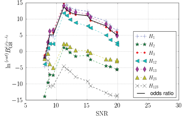
FIG. 9 (color online). The buildup of cumulative Bayes factors against GR for individual hypotheses, and the odds ratio, for a typical catalog with \delta\chi_3 = 0.025 . Note that on the basis of the Bayes factor against GR of the most inclusive hypothesis H_{123} alone, one can conclude that the GR model is in fact the favored one. Even the log Bayes factor for H_{23} ends up being negative. Additionally, the hypothesis with the largest Bayes factor is not H_3 but H_1 . This illustrates that it is necessary to include as many hypotheses as possible in the analysis.
