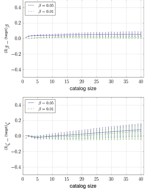
FIG. 12 (color online). Top panel: The difference of false alarm probabilities, (3)\beta - (\text{target})\beta , for fixed log odds ratio thresholds and signals having \delta\chi_3 = 0.025 , between our three-parameter test and a “targeted search” which only looks for a deviation in \psi_3 , i.e., only tests the hypothesis H_3 against GR. We see that the difference is minor. Bottom panel: The difference in efficiencies (which is more important), (3)\zeta - (\text{target})\zeta , for fixed false alarm probabilities. Especially for a large number of sources per catalog, our three-parameter test is actually more efficient than the “targeted search,” at least for this particular example. This is because the Bayes factor against GR for H_3 will not be the largest in every catalog, but our method naturally compensates for that. Of course, we do not expect our method to outperform a targeted search in the case of a more complicated deviation from GR.
