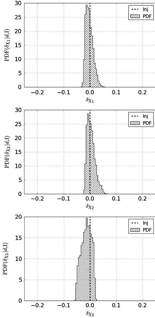
FIG. 17. Posterior PDFs for a single GR injection with network SNR of 23.0. Top panel: \delta\chi_1 measured with a waveform that has \{\hat{\theta}, \delta\chi_1\} as free parameters. Middle panel: \delta\chi_2 measured with a waveform that has \{\hat{\theta}, \delta\chi_2\} free. Bottom panel: \delta\chi_3 measured with a waveform that has \{\hat{\theta}, \delta\chi_3\} free. In each case the distribution is tightly centered on zero, with standard deviations of 0.014, 0.015, and 0.019, respectively.
