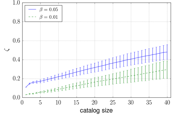
FIG. 10 (color online). The efficiency of detecting a GR violation for sources with \delta\chi_3 = 0.025 , as a function of catalog size for false alarm probabilities \beta \in \{0.05, 0.01\} . The median and the 68% confidence interval from 5000 random catalog orderings are shown as the central curve and the error bars, respectively. The efficiency increases as a function of catalog size, once again underscoring the benefit of combining all available data.
