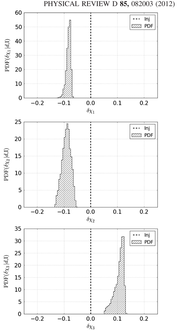
FIG. 22. The posterior PDFs for \delta\chi_1 (top panel), \delta\chi_2 (middle panel), and \delta\chi_3 (bottom panel) for a single injection with \delta\chi_A = -2.2 and network SNR of 22.4, recovered with waveforms where, respectively, \{\vec{\theta}, \delta\chi_1\} , \{\vec{\theta}, \delta\chi_2\} , and \{\vec{\theta}, \delta\chi_3\} are free. The distribution of \delta\chi_3 has its median at 0.11 and a standard deviation of 0.017. Note the remarkable resemblance with Fig. 18, where the signal had \delta\chi_3 = 0.1 . Also for \delta\chi_1 and \delta\chi_2 , the distributions are very similar to the ones for a signal with \delta\chi_3 = 0.1 .
