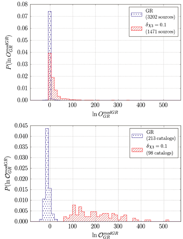
FIG. 5 (color online). Top panel: The normalized distribution P(\ln O_{\text{GR}}^{\text{modGR}}) of log odds ratios for individual sources, where the injections are either GR or have \delta\chi_3 = 0.1 . Bottom panel: The normalized distribution P(\ln O_{\text{GR}}^{\text{modGR}}) of logs of the combined odds ratios for GR injections and injections with \delta\chi_3 = 0.1 , for catalogs of 15 sources each. The effectiveness of the catalog approach to testing for deviations from GR comes from the combination of multiple sources, each source contributing to the overall result in proportion to its own Bayes factors.
