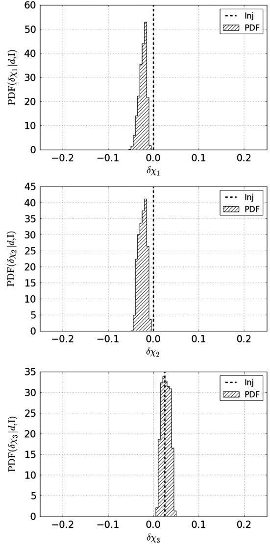
FIG. 21. The posterior PDFs for \delta\chi_1 (top panel), \delta\chi_2 (middle panel), and \delta\chi_3 (bottom panel) for a single injection with \delta\chi_3 = 0.025 and network SNR of 20.6, recovered with waveforms where, respectively, \{\vec{\theta}, \delta\chi_1\} , \{\vec{\theta}, \delta\chi_2\} , and \{\vec{\theta}, \delta\chi_3\} are free. Again, \delta\chi_3 is peaked at close to the correct value, with a median of 0.027 and a standard deviation of 0.0092, but both \delta\chi_1 and \delta\chi_2 are strongly peaked at incorrect values.
