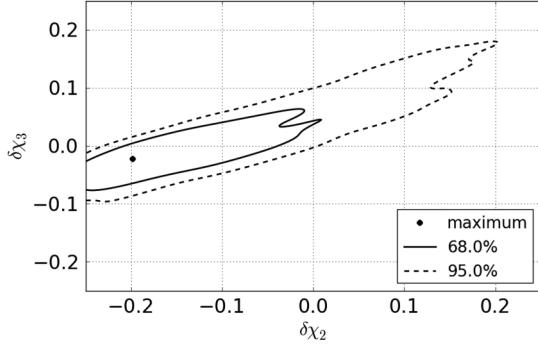
FIG. 23. The 68% and 95% confidence contours of the two-dimensional PDF for \{\delta\chi_2, \delta\chi_3\} , for an injection with \delta\chi_A = -2.2 , and with a waveform that has \{\tilde{\theta}, \delta\chi_1, \delta\chi_2, \delta\chi_3\} as free parameters. The maximum of the PDF is given by the black dot. Here the distribution is quite different from the case with \delta\chi_3 = 0.1 (Fig. 20).
