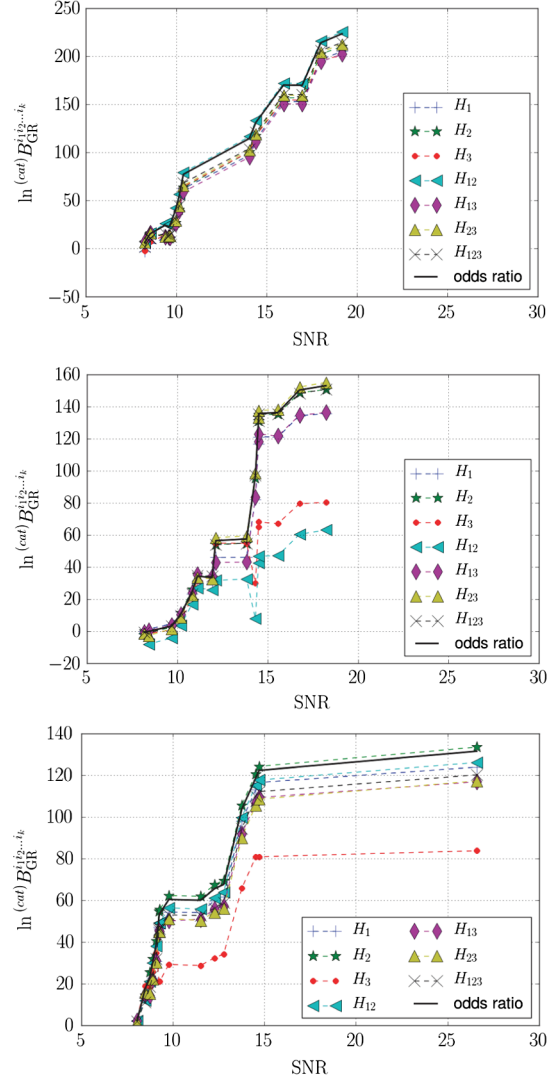
FIG. 16 (color online). A few examples of how cumulative Bayes factors against GR for individual hypotheses, and the odds ratio, grow as sources with increasing SNR are being added within three different catalogs of 15 sources in total. Top and middle panels: Catalogs where sources have only modest SNRs ( < 20 ). Note the large differences in contributions from different hypotheses, and in the ordering of Bayes factors, between these two catalogs. Bottom panel: A catalog with a high SNR source; note, however, that the source with the highest SNR does not cause a particularly large “boost,” and the cumulative log odds ratio ends up being considerably lower than in the top and middle examples.
