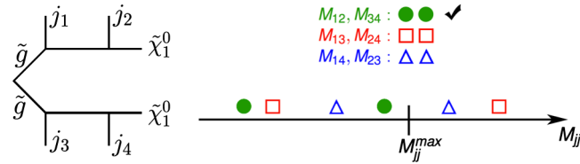
FIG. 6 (color online). This illustrates a special type of event for which we can identify the correct decay chain assignment. The correct decay chain assignment is labeled with a circle, while the incorrect ones are labeled by a square and triangle. If one or both of the invariant masses of each of the wrong pairings lie above M_{jj}^{\max} and both invariant masses of the correct pairing lie below M_{jj}^{\max} (which is guaranteed at parton level in the absence of measurement errors) then we can identify the correct pairing for this event.
