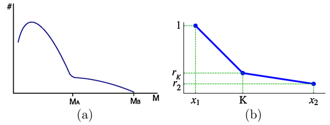
FIG. 1 (color online). (a) A schematic example of a distribution in some kinematic variable M which features two edges/end points at M = M_A, M_B . (b) The linear kink fit function used in our procedure. For each fit with chosen fit domain (x_1, x_2) , the variables K, r_K, r_2 float, with K being the kink position.
