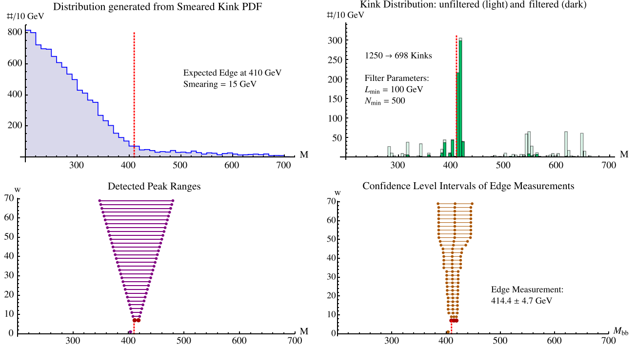
FIG. 5 (color online). Applying the edge-to-bump method to a distribution of 10 000 points generated from a smeared kink PDF. The dotted line indicates the expected edge position, and the peak range and confidence interval used for the final edge measurement are marked in bold.
