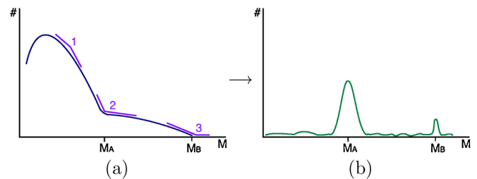
FIG. 2 (color online). (a) The data is fit to the linear kink function over all the generated domains, here shown for three examples. Each domain yields a kink position value K . (b) After applying some basic filters we plot the distribution of the obtained values of K . Edges in the data show up as peaks in the kink distribution.
