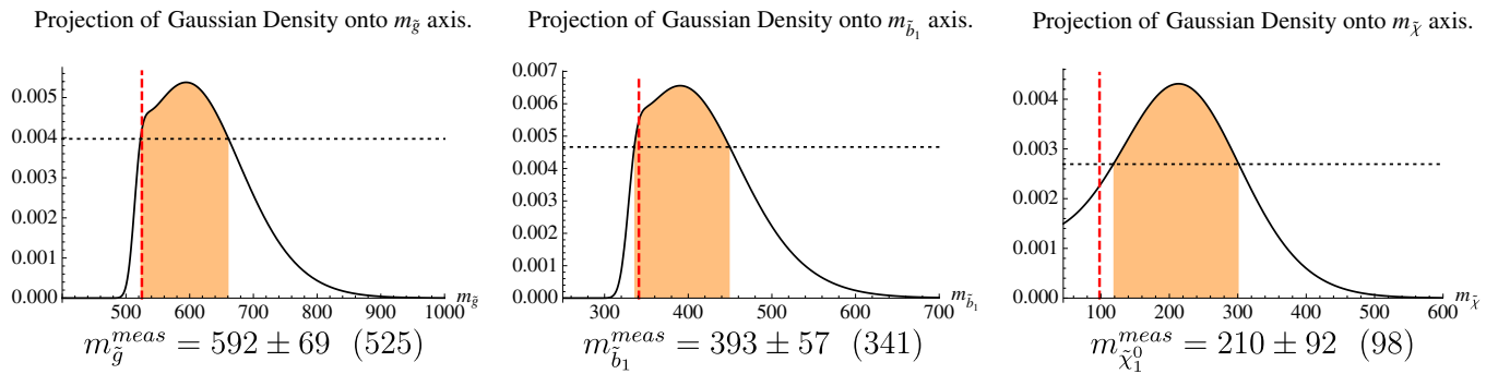
FIG. 11 (color online). Mass measurements for the first Monte Carlo study in GeV (actual masses in brackets). The plots show the Gaussian density projections for the three masses. The 1\text{-}\sigma confidence level interval is shaded, and the true mass value is indicated with the vertical dashed line. The dotted line indicates the value of \mathcal{D}_{\min} which defines the confidence interval.
