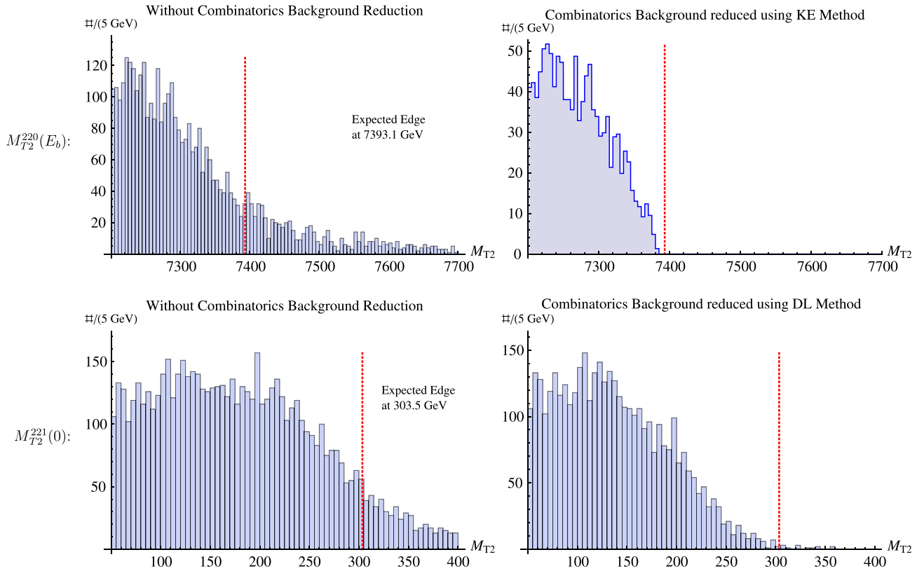
FIG. 9 (color online). Examples of reduced combinatorics background: KE method applied to the M_{T2}^{220}(E_b) distribution (top), and DL method applied to the M_{T2}^{221}(0) distribution (bottom) from our first Monte Carlo study in Sec. V. ( p_T^{\text{ISR}} cutoff used to control ISR smearing. All units in GeV. Includes detector effects and hadronization/showering.)
