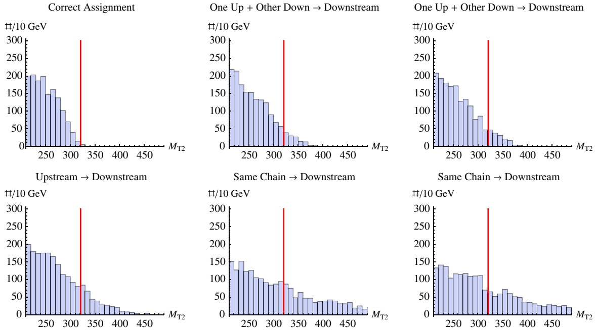
FIG. 8 (color online). The M_{T2}^{210}(0) distributions for the six possible ways to assign two of the four b -jets in the process pp \rightarrow \tilde{g} \tilde{g} \rightarrow 2\tilde{b} + 2b \rightarrow 4b + 2\chi_1^0 as downstream. The test mass is zero and the MSSM parameters for the parton level simulation were the same as for our first Monte Carlo study in Sec. V. The vertical line indicates the expected position of M_{T2}^{210}(0)^{\max} .
