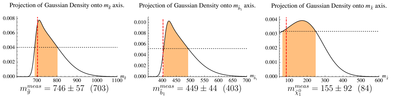
FIG. 12 (color online). Mass measurements for the second Monte Carlo study in GeV (actual masses in brackets). The plots show the Gaussian density projections for the three masses. The 1\sigma confidence level interval is shaded, and the true mass value is indicated with the vertical dashed line. The dotted line indicates the value of \mathcal{D}_{\min} which defines the confidence interval.
