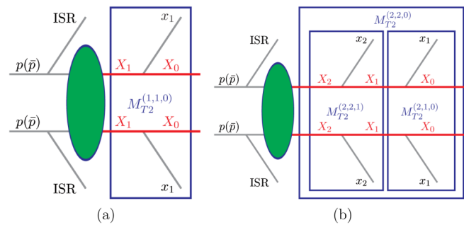
FIG. 7 (color online). (a) A simple 1-step symmetric decay chain. A hard process produces two particles X_1 , which decay to invisible particles X_0 and SM daughters x_1 . The box represents the particles entering the construction of the simple M_{T2} variable. (b) A 2-step symmetric decay chain with the particles entering the respective M_{T2} -subsystem variables indicated. In each case we use (1) and (2) superscripts to distinguish transverse momenta from the two decay chains. Figure reproduced from [7] with permission of the authors.
