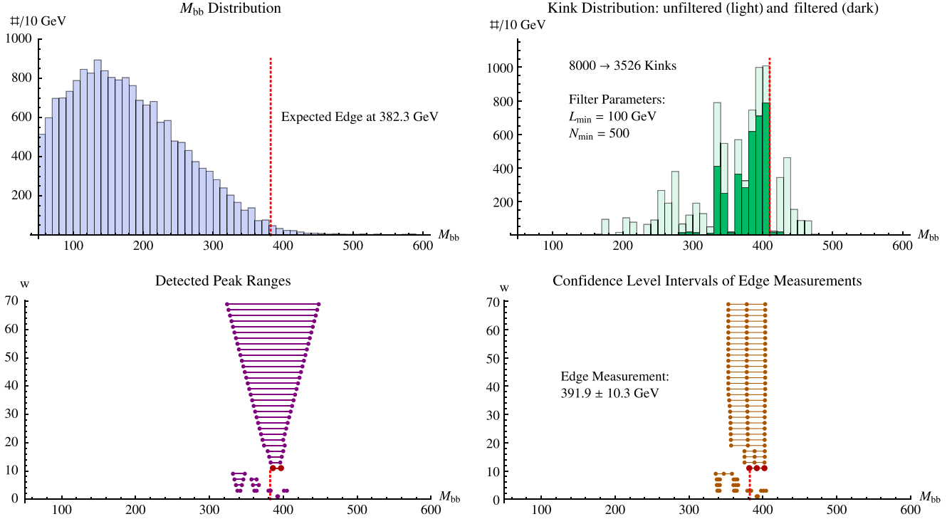
FIG. 4 (color online). Applying the edge-to-bump method to measure the kinematic-edge in the cleaned up M_{bb} distribution of 18 770 points from our first Monte Carlo study. Note how the physical edge reliably shows up as a growing upside down cone in the peak range plot and is distinguished from noise at small w . The dotted line indicates the expected edge position, and the peak range and confidence interval used for the final edge measurement are marked in bold.
