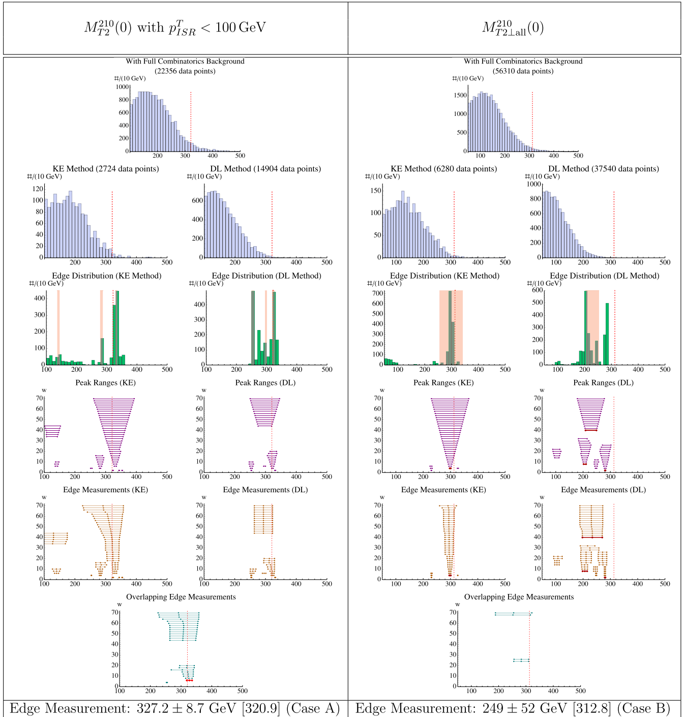
FIG. 10 (color online). The complete edge measurements for two of the 14 examined M_{T2} distributions in the first Monte Carlo study. (Expected end point locations in square brackets.) See the Appendix for the other measurements.
