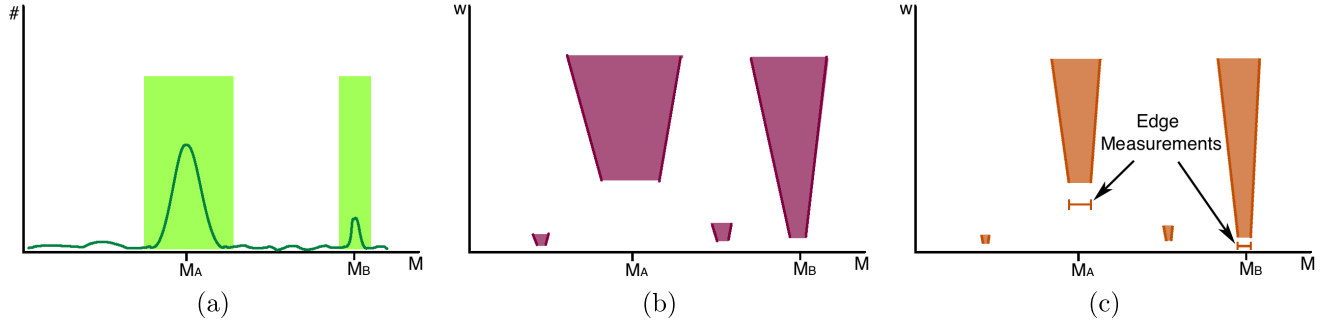
FIG. 3 (color online). (a) For a given w , we detected two peaks in the kink distribution (peak intervals shaded). (b) A plot of the found peak intervals as a function of w . Note how the two real peaks are reliably detected above some minimum w (which depends on the size of the peak), while small-scale fluctuations only show up at small w . (c) Plot of 1\text{-}\sigma confidence level intervals of the peak's position for each w . For the two physical peaks, keep the measurement with the smallest error as the final measurement of the peak/edge position.
