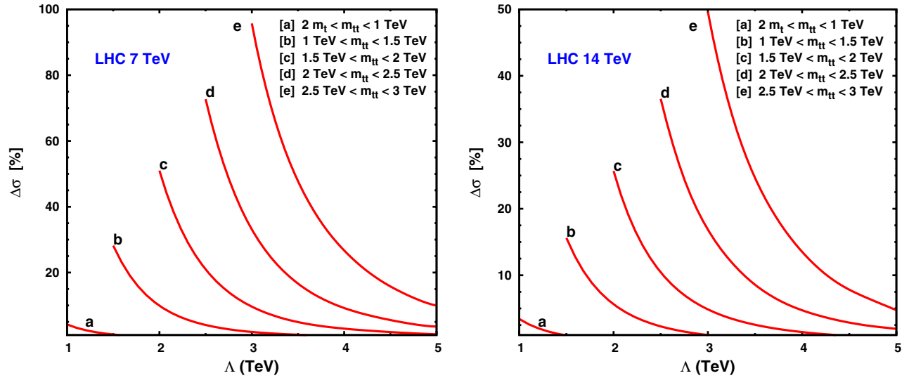
FIG. 9 (color online). Percentage variation \Delta\sigma of the total cross section for pp \rightarrow t\bar{t} at LHC, with pp center of mass energies \sqrt{S} = 7 TeV (left plots) and \sqrt{S} = 14 TeV (right plot) for m_t = 172 GeV, as a function of the scale \Lambda in TeV, for several regions ([a-e]) of t\bar{t} -invariant mass m_{t\bar{t}} .
