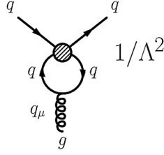
FIG. 1. Feynman diagram in the effective low-energy theory that generates the effective axial-vector coupling of gluon, where \Lambda is the scale related to the contact 4-quarks operator.
