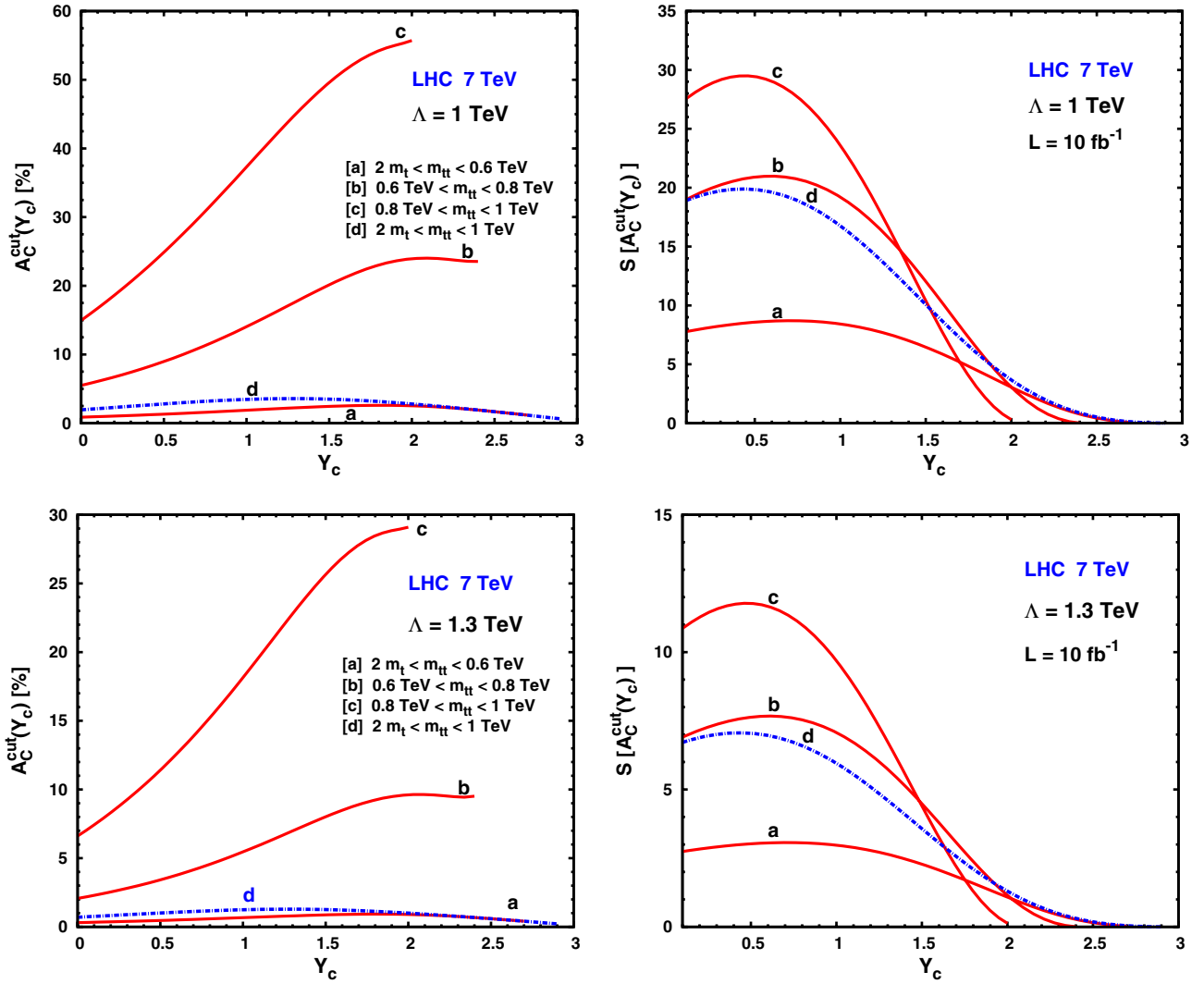
FIG. 7 (color online). Cut-dependent pair charge asymmetry A_C^{\text{cut}}(Y_c) in percentage (left plots) and corresponding statistical significance S[A_C^{\text{cut}}(Y_c)] (right plots) at LHC, with pp center of mass energy \sqrt{S} = 7 TeV and integrated luminosity L = 10 \text{ fb}^{-1} , with m_t = 172 GeV, as a function of the cuts on the mean rapidity |Y| > Y_c (in the lab frame), for several regions ([a-d]) of t\bar{t} -invariant mass m_{t\bar{t}} . Up and down plots correspond to the scale \Lambda = 1 TeV and \Lambda = 1.3 TeV, respectively.
