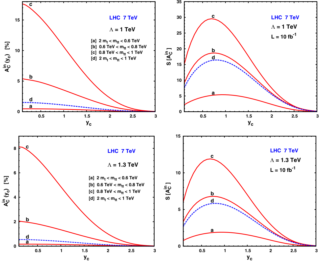
FIG. 4 (color online). The t\bar{t} charge asymmetry A_C^{\text{in}}(y_c) in percentage (left plots) and corresponding statistical significance S[A_C^{\text{in}}] (right plots) at LHC, with pp center of mass energy \sqrt{S} = 7 TeV and integrated luminosity L = 10 \text{ fb}^{-1} , with m_t = 172 GeV, as a function of the cuts on the t\bar{t} -quark rapidity y_c (in the lab frame) and for several regions ([a-d]) of t\bar{t} -invariant mass m_{t\bar{t}} . Up and down plots correspond to the scale \Lambda = 1 TeV and \Lambda = 1.3 TeV, respectively.
