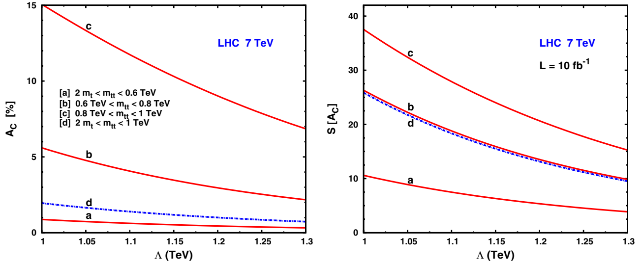
FIG. 6 (color online). The cut-independent t\bar{t} charge asymmetry A_C in percentage (left plots) and corresponding statistical significance S[A_C] (right plots) at LHC, with pp center of mass energy \sqrt{S} = 7 \text{ TeV} and integrated luminosity L = 10 \text{ fb}^{-1} , with m_t = 172 \text{ GeV} , as a function of the scale \Lambda in TeV, for several regions ([a-d]) of t\bar{t} -invariant mass m_{t\bar{t}} .
