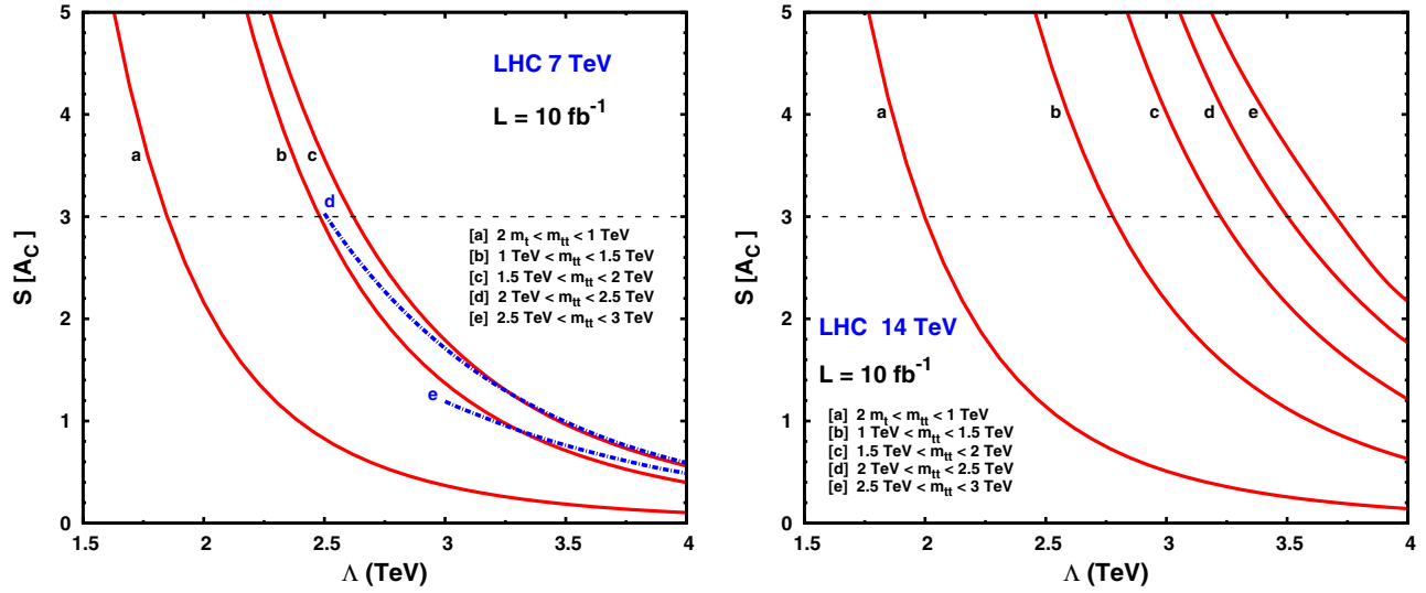
FIG. 8 (color online). Statistical significance S[A_C] of the cut-independent t\bar{t} charge asymmetry A_C at LHC, with pp center of mass energies \sqrt{S} = 7 TeV (left plots) and \sqrt{S} = 14 TeV (right plot) with integrated luminosity L = 10 \text{ fb}^{-1} , with m_t = 172 GeV, as a function of the scale \Lambda in TeV, for several regions ([a-e]) of t\bar{t} -invariant mass m_{t\bar{t}} .
