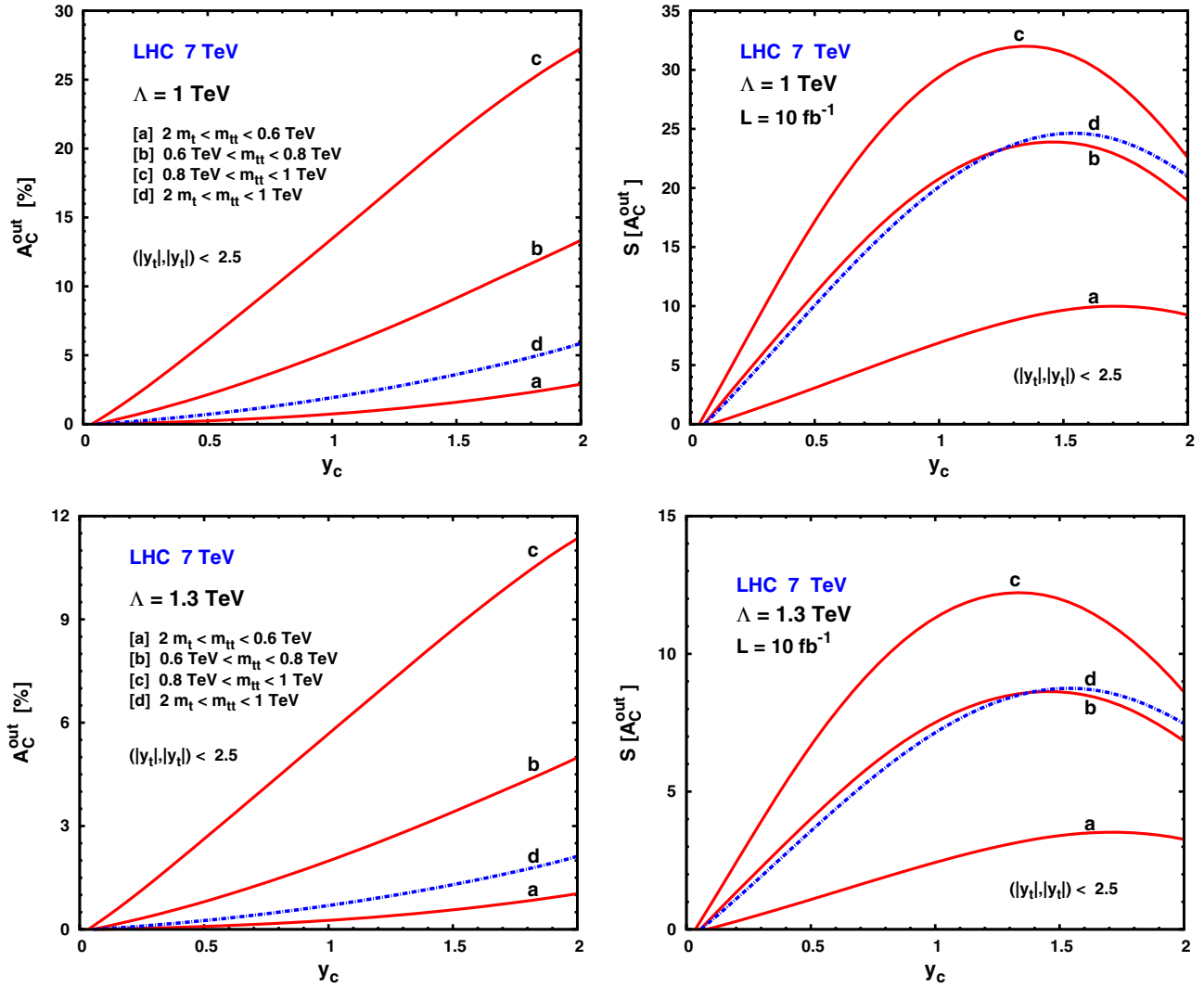
FIG. 5 (color online). The t\bar{t} charge asymmetry A_C^{\text{out}}(y_c) in percentage (left plots) and corresponding statistical significance S[A_C^{\text{out}}] (right plots) at LHC, with pp center of mass energy \sqrt{S} = 7 TeV and integrated luminosity L = 10 \text{ fb}^{-1} , with m_t = 172 GeV, as a function of the cuts on the t\bar{t} -quark rapidity y_c (in the lab frame), for several regions ([a-d]) of t\bar{t} -invariant mass m_{t\bar{t}} . The upper constraints on rapidities (|y_t|, |y_{\bar{t}}|) < 2.5 is imposed. Up and down plots correspond to the scale \Lambda = 1 TeV and \Lambda = 1.3 TeV, respectively.
