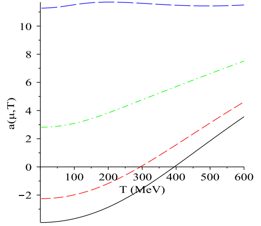
FIG. 11 (color online). Coefficient of \sigma^2 , a(\mu, T) , for various values of the chemical potential (solid = 0, dash = 150 MeV, dot-dash = 300 MeV, long-dash = 450 MeV). For a < 0 the \sigma^2 term favors spontaneous formation of a chiral condensate.
