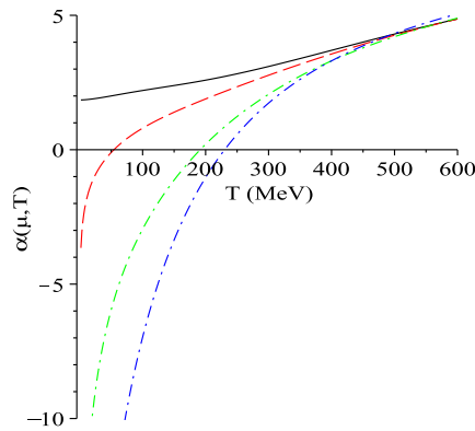
FIG. 12 (color online). (a) Coefficient of |d|^2 , \alpha(\mu, T) , for various values of the chemical potential (same as Fig. 11). For \alpha < 0 the |d|^2 term favors spontaneous formation of a diquark condensate. (b) Coefficient of \Phi , A(\mu, T) , for various values of the chemical potential. For A(T) < 0 the linear term favors the formation of a nonzero \Phi .
