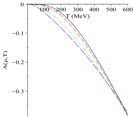
FIG. 12 (color online). (a) Coefficient of |d|^2 , \alpha(\mu, T) , for various values of the chemical potential (same as Fig. 11). For \alpha < 0 the |d|^2 term favors spontaneous formation of a diquark condensate. (b) Coefficient of \Phi , A(\mu, T) , for various values of the chemical potential. For A(T) < 0 the linear term favors the formation of a nonzero \Phi .
