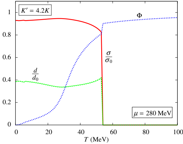
FIG. 10 (color online). Plot of the normalized chiral and diquark condensates and Polyakov loop for \mu = 280 MeV.
