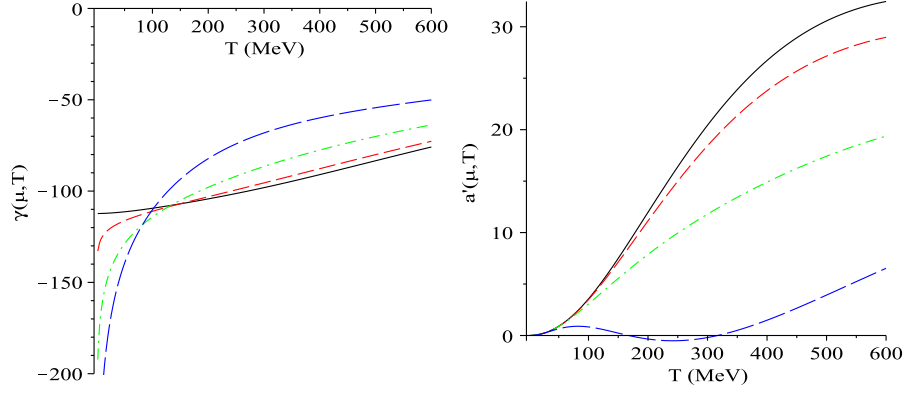
FIG. 13 (color online). (a) The coefficient of \sigma|d|^2 , \gamma(\mu, T) , for various values of the chemical potential (same as Fig. 11). For \gamma < 0 the system favors coexistence of chiral and diquark condensates. (b) Coefficient of \sigma^2\Phi , a'(\mu, T) , for various values of the chemical potential. For a' < 0 , the \sigma^2\Phi term favors simultaneous formation of a chiral condensate and deconfinement.
