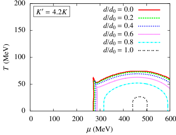
FIG. 9 (color online). Contour plot for the diquark condensate in the PNJL model.
