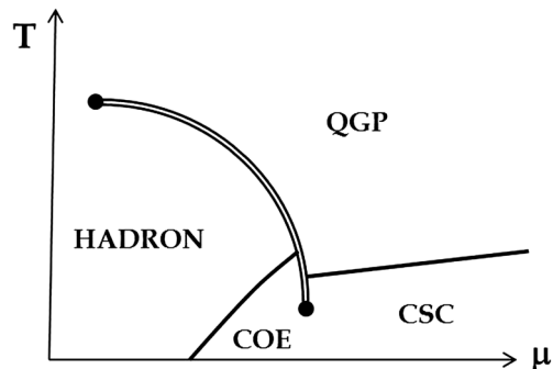
FIG. 1. Schematic QCD phase diagram showing regions of broken chiral symmetry (hadron), BCS quark pairing and color superconductivity (CSC), coexistence of chiral and diquark condensates (COE), and a deconfined quark-gluon plasma (QGP). Single lines denote second order phase transitions while double lines denote first-order transitions. Adapted from [10].
