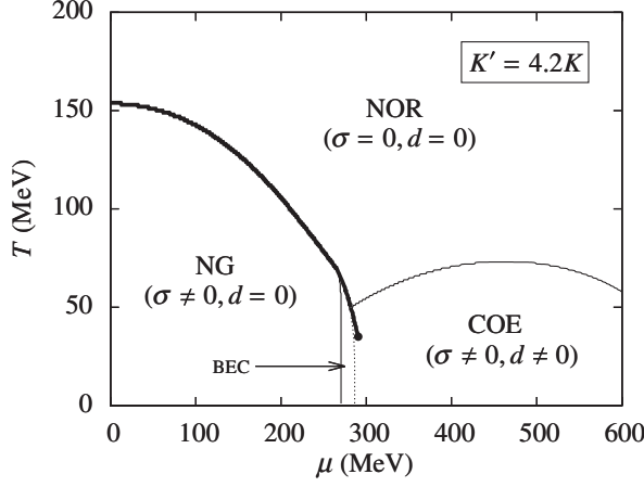
FIG. 3. Phase diagram for the three-flavor NJL model (no confinement). Thick lines represent first-order phase transitions while thin lines represent second order transitions. The dotted vertical line is the BEC-BCS crossover, defined by M(\mu, T) = \mu . The low T critical point is at (\mu, T) = (291 \text{ MeV}, 35 \text{ MeV}) .
