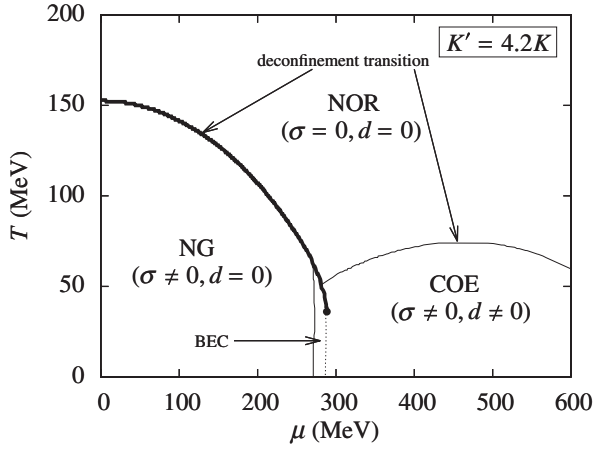
FIG. 6. Phase diagram for the three-flavor PNJL model. Thick lines represent first-order transitions, while thin lines represent second order transitions. The dotted vertical line is the BEC-BCS crossover, defined by M(\mu, T) = \mu . The low T critical point is at (\mu, T) = (288 \text{ MeV}, 36 \text{ MeV}) .
