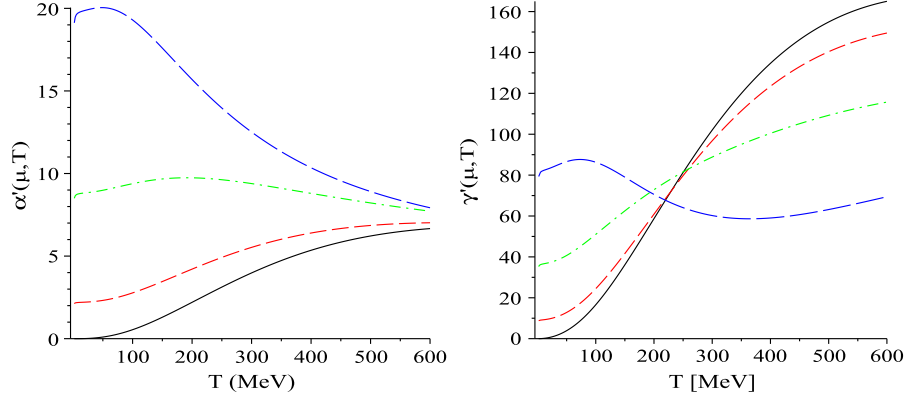
FIG. 14 (color online). (a) The coefficient of |d|^2\Phi , \alpha'(\mu, T) , for various values of the chemical potential (same as Fig. 11). For \alpha' < 0 , the |d|^2\Phi term favors the coexistence of a diquark condensate and deconfinement. (b) Coefficient of \sigma|d|^2\Phi , \gamma'(\mu, T) , for various values of the chemical potential. For \gamma' < 0 , the system favors the coexistence of \sigma , d , and \Phi .
