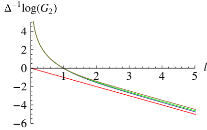
FIG. 1 (color online). Logarithm of the thermal correlator for different values of z . The different curves correspond to z = 1, 2, 6 , from bottom to top. The (red) line is a line with slope -1 . The figure shows that the thermal correlation function is fairly independent of the value of z .
