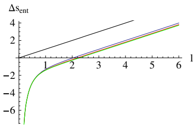
FIG. 8 (color online). The finite part of the entanglement entropy density as a function of the width of the strip l , in the thermal state. The different curves correspond to the values z = 2, 4, 6 from top to bottom. The straight line is a reference line with slope 1.
