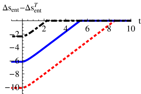
FIG. 10 (color online). Evolution of the entanglement entropy density in the quench state for z = 2 , with the thermal value subtracted. The different curves correspond to the values l = 4, 8, 12 .
