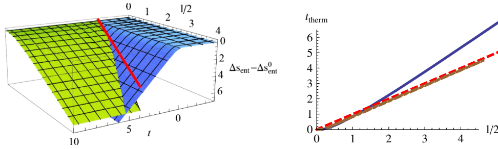
FIG. 9 (color online). (left-hand figure) The entanglement entropy density in the quench state as a function of the width of the strip l and the time t , for the case of z = 2 . The (red) line corresponds to the upper bound velocity, which in dimensionless coordinates is simply 1. (right-hand figure) The (blue) solid curve is the real thermalization time, while the (brown) dot-dashed curve is the lower bound for the thermalization time and the (red) dashed curve is a reference line with slope 1. As the figure shows, thermalization of the entanglement entropy really happens more slowly than the upper bound due to multiple surfaces contributing to the same values of (l, t) .
