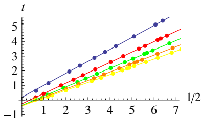
FIG. 3 (color online). Lower bounds for thermalization times for different values of z . The data points are obtained by numerical integration of the integral in (49). From top to bottom the different colored data points correspond to the values z = 1, 2, 3, 4, 5 . The lines with the corresponding colors are best fit lines with slopes given by (54).
