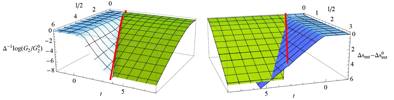
FIG. 11 (color online). (left-hand figure) The logarithm of the two-point correlation function with vacuum value subtracted, for z = 2 and 3 + 1 dimensional dual field theory. The (red) curve corresponds to the upper bound speed v = \sqrt{10} from (A4). (right-hand figure) The entanglement entropy density for the same d and z . The (red) curve corresponds to the upper bound speed v = \sqrt{10}/3 from (A10).
