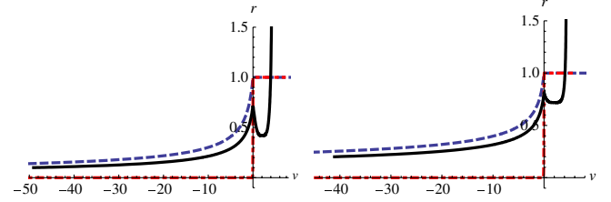
FIG. 2 (color online). In both of the figures the dot-dashed curve (red) corresponds to the apparent horizon, the dashed curve (blue) to the event horizon, and the solid curve (black) to a generic geodesic contributing to the two-point function. The left-hand figure corresponds to z = 2 and the right-hand figure to z = 3 . The geodesic is seen to pass through both horizons, once through the event horizon and twice through the apparent horizon.
