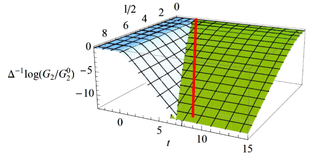
FIG. 5 (color online). Logarithm of the quench correlator for z = 2 , with the vacuum value subtracted. The (red) line is a reference line with slope dl/dt = 2 .
