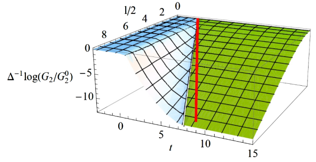
FIG. 4 (color online). Logarithm of the quench correlator for z = 1 , with the vacuum value subtracted. The (red) line corresponds to twice the speed of light. The narrow (blue) surface corresponds to geodesics passing through the matter shell, while the wide (green) surface corresponds to geodesics probing the u < 1 region.
