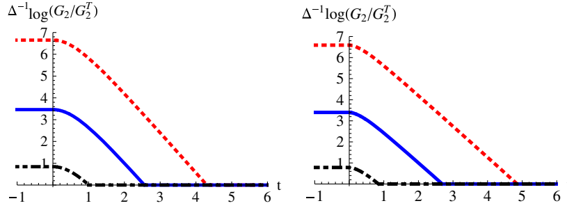
FIG. 7 (color online). Logarithm of the two-point correlator, with its thermal value subtracted. The different curves correspond to different values of l as l = 4, 8, 12 from bottom to top. The left-hand figure is for z = 2 while the right-hand figure is for z = 3 .
