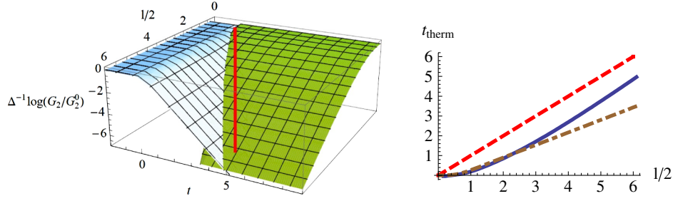
FIG. 6 (color online). (left-hand figure) Logarithm of the quench correlator for z = 3 with the vacuum value subtracted. The (red) line is a reference line with slope dl/dt = 2 . The thermalization is seen to happen very suddenly as there are several geodesics contributing. (right-hand figure) The (blue) solid line is the real thermalization time extracted from the correlator, while the (red) dashed line is a reference line with slope 1 and the (brown) dot-dashed line is the lower bound for the thermalization time as obtained from numerical integration of (48) and (49).
