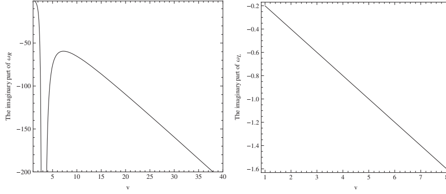
FIG. 2. Variety of the imaginary part of the fundamental quasinormal modes \omega_R (the left) and \omega_L (the right) with the parameters \nu for fixed \eta = 0 . Here, we set r_+ = 1 , r_- = 0.1 , k = 2 , L = 10 , and m = 0.01 .
