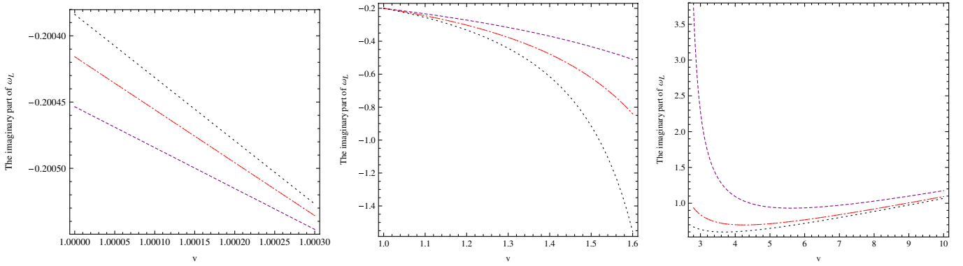
FIG. 4 (color online). Variety of the imaginary part of the fundamental quasinormal modes \omega_L with the parameters \nu and \eta . The dashed, dash-dotted, and dotted curves are for \eta = 10, 20 , and 30 , respectively. Here, we set r_+ = 1 , r_- = 0.1 , k = 2 , L = 10 , and m = 0.01 .
