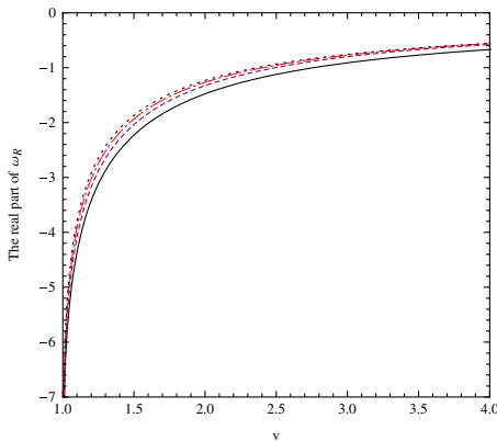
FIG. 1 (color online). Variety of the real part of the fundamental quasinormal modes \omega_R with the parameters v and \eta . The solid, dashed, dash-dotted, and dotted curves are for \eta = 0, 10, 20 , and 30 , respectively. Here, we set r_+ = 1 , r_- = 0.1 , k = 2 , L = 10 , and m = 0.01 .
