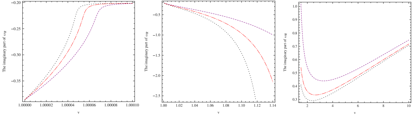
FIG. 3 (color online). Variety of the imaginary part of the fundamental quasinormal modes \omega_R with the parameters \nu and \eta . The dashed, dash-dotted, and dotted curves are for \eta = 10, 20 , and 30 , respectively. Here, we set r_+ = 1 , r_- = 0.1 , k = 2 , L = 10 , and m = 0.01 .
