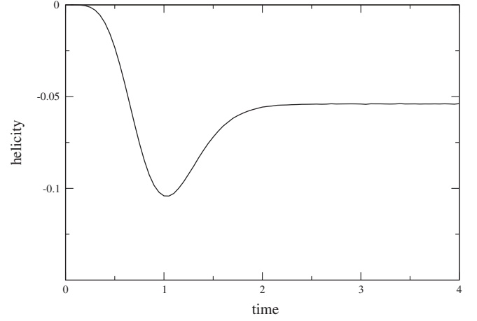
FIG. 1. \mathcal{F}(t) versus t/r_t for r_t = r_f = r_h .
