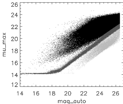
FIG. 1. Resolved galaxies (black points) are a distinct population. Also shown are point sources (dark gray) including stars, and spurious objects (light gray) that are too small to be consistent with the PSF.
