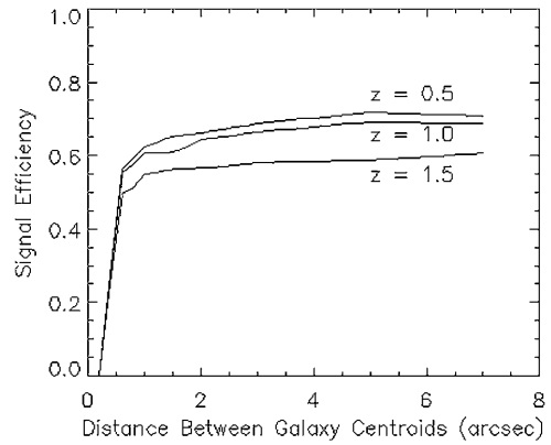
FIG. 4. Efficiency of detecting pairs of galaxies lensed by a cosmic string as a function of pair opening angle and redshift.
