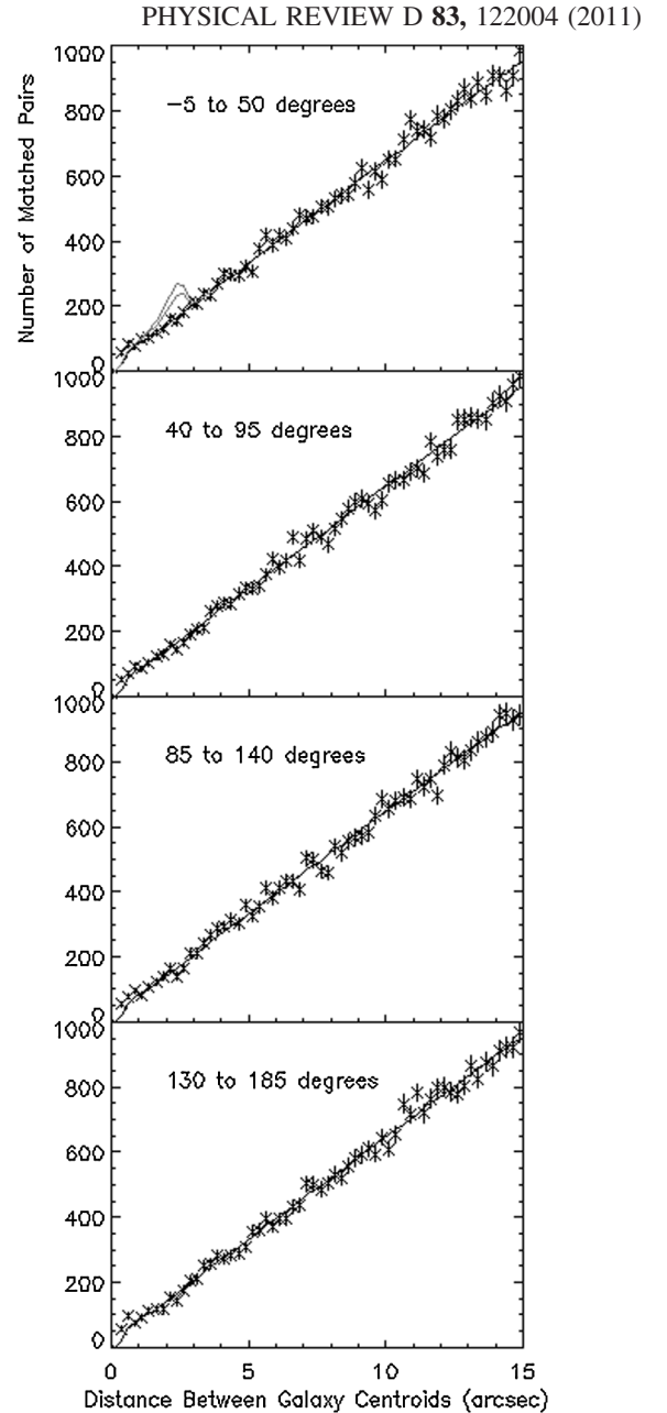
FIG. 2. Pairs of galaxies in four angular bins (points) are compared to background (solid line). The top panel shows one example of a simulated string (grey). The upper simulated string is the total number of pairs expected from the simulation with string length of 1.19^\circ , redshift of 0.5, and \delta \sin\beta of 4'' . The lower simulated string includes measurement inefficiencies.
