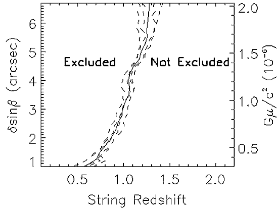
FIG. 5. 95% upper limits for lensed galaxies produced by a cosmic string as a function of the string mass and redshift. Dashed lines are the individual limits from each angular bin shown in Fig. 2. The solid line is the average limit for all directions.
