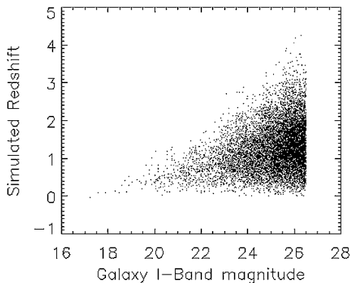
FIG. 3. The simulated redshift distribution for galaxies in a typical COSMOS tile.
