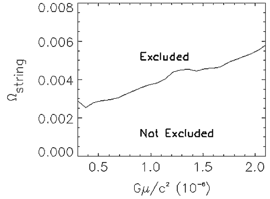
FIG. 6. 95% upper limits on the global parameter, \Omega_{\text{strings}} , as a function of the string mass.
