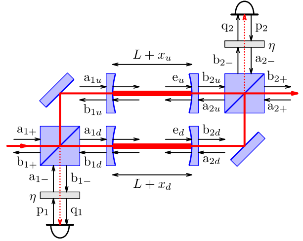
FIG. 7 (color online). To calculation of the Mach-Zehnder/Fabry-Perot interferometer quantum noises.
