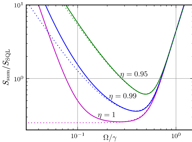
FIG. 6 (color online). Plots of \frac{\mu\Omega^2}{\hbar} S_{\text{sum}} [see Eq. (31)] for m/M = 0.01 (solid lines) and m/M \rightarrow 0 (dots). For all plots, \mathcal{K}_0 = 2 .
