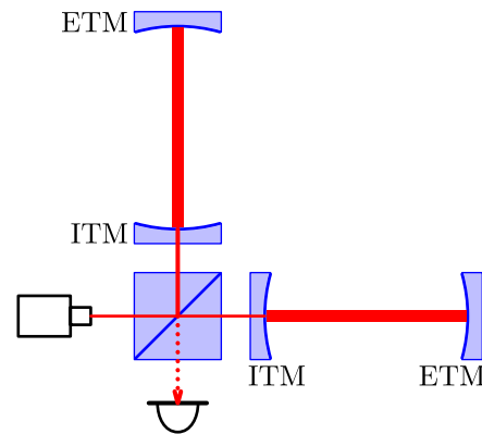
FIG. 1 (color online). Simplified scheme of the Michelson interferometer topology of laser gravitational-wave detectors. ITM: input test masses; ETM: end test masses.
