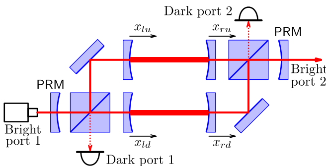
FIG. 2 (color online). The scheme of Mach-Zehnder/Fabry-Perot interferometer.
