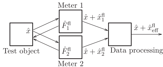
FIG. 3. Generalized scheme of the dual linear quantum meter.
