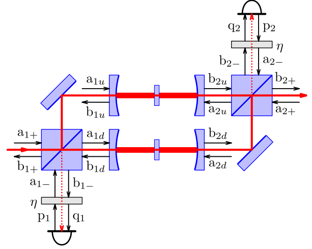
FIG. 9 (color online). To calculation of the Mach-Zehnder/Fabry-Perot speed meter quantum noises.
