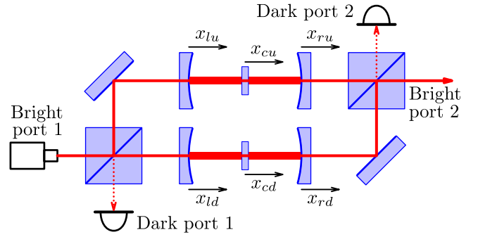
FIG. 4 (color online). The scheme of the Mach-Zehnder/Fabry-Perot quantum speed meter.
