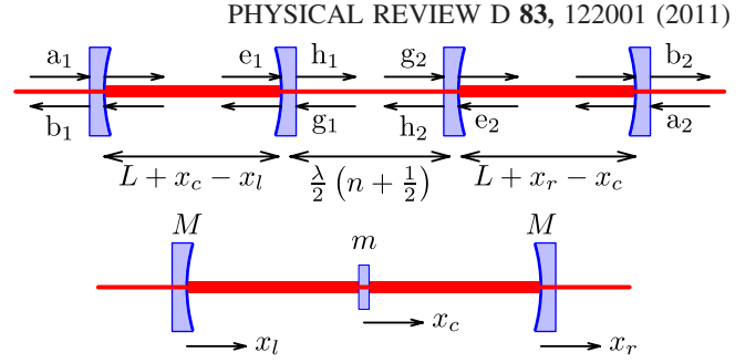
FIG. 8 (color online). One arm of the two-port speed meter: top—optical scheme, bottom—mechanical scheme.
