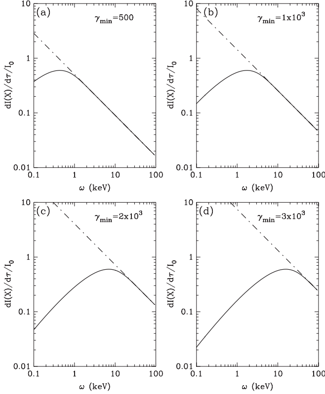
FIG. 5. Plotting of dI(X)/d\tau as a function of the photon energy \omega in X-ray energy regions for a typical value \sigma = 2.5 . Figures 5(a)–5(d) correspond to \gamma_{\min} = 500 , 1 \times 10^3 , 2 \times 10^3 , and 3 \times 10^3 , respectively. The solid curve corresponds to the full calculation of Eq. (56). The dash-dotted curve is the power-law approximation of Eq. (59).
