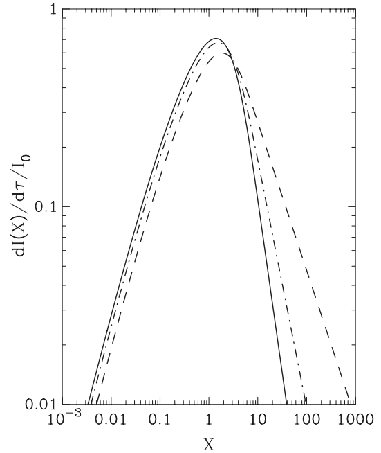
FIG. 3. Plotting of dI(X)/d\tau . The dashed curve, dash-dotted curve, and solid curve correspond to \sigma = 2.5, 3.5 , and 4.5 , respectively.
