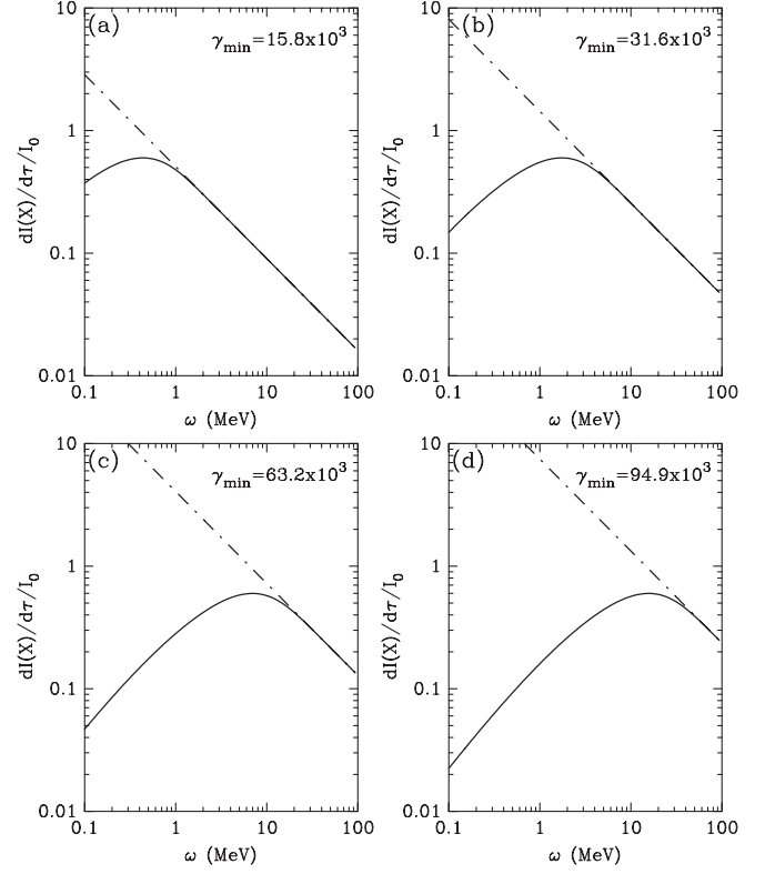
FIG. 6. Plotting of dI(X)/d\tau as a function of the photon energy \omega in gamma-ray energy regions for a typical value \sigma = 2.5 . Figures 6(a)–6(d) correspond to \gamma_{\min} = 15.8 \times 10^3 , 31.6 \times 10^3 , 63.2 \times 10^3 , and 94.9 \times 10^3 , respectively. The solid curve corresponds to the full calculation of Eq. (56). The dash-dotted curve is the power-law approximation of Eq. (59).
