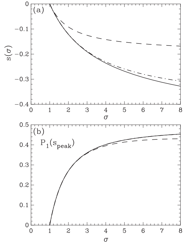
FIG. 2. Plotting of s(\sigma) and P_1(s_{\text{peak}}) . Figures 2(a) and 2(b) are s(\sigma) and P_1(s_{\text{peak}}) , respectively. The dashed curve, dash-dotted curve, and solid curve correspond to the first-order approximation, third-order approximation, and numerical solution, respectively.
