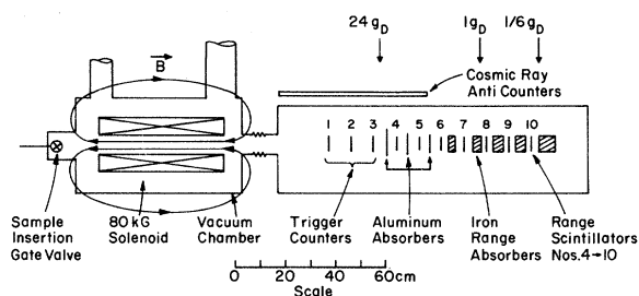
FIG. 1. Schematic diagram of monopole accelerator solenoid and detector system. The arrows indicate stopping positions in the range absorbers of monopoles with 24, 1, \frac{1}{6} Dirac charges. An iron backstop 2.0 cm thick is placed behind the sample to catch any poles of opposite polarity.
