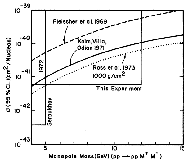
FIG. 2. Upper limit for the cross section of monopole production in p -nucleon collisions. Relevant cross sections based on A^{2/3} are shown. The 12-GeV limit is the result of this experiment. The 5-GeV limit is Serpukhov (Ref. 11). The dashed line is Fleischer et al. (Ref. 10), the dotted line is Ross et al. (Ref. 8), and the solid line is Kolm et al. (Ref. 9).
