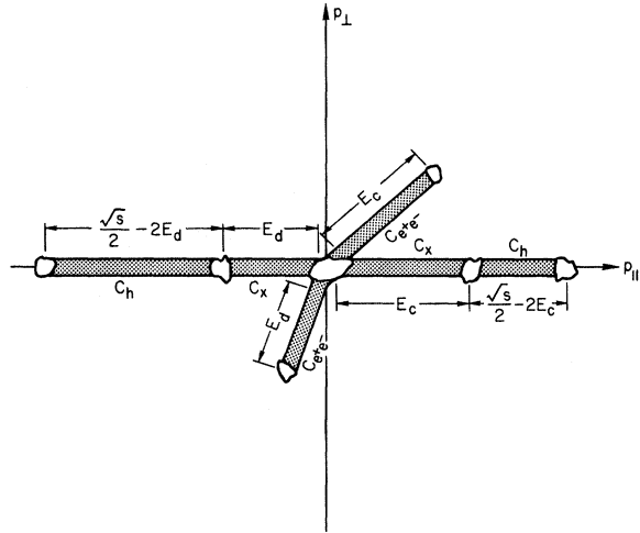
FIG. 2. Average final-hadron distribution for a typical deep-scattering event.
