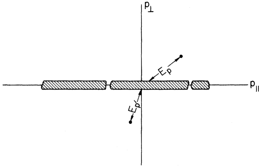
FIG. 1. Parton distribution immediately after hard parton-parton scattering.
