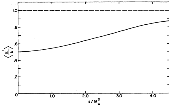
FIG. 1. The mean energy of the muon in the presence of an intermediate vector boson as a function of s / M_W^2 .
