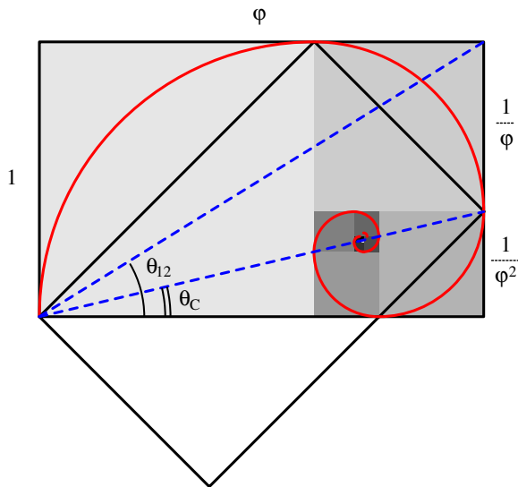
FIG. 1 (color online). Geometrical illustration of the connection between our predictions for \theta_{12} and \theta_C and the golden rectangle. The two dashed lines are the reflection axis of the Z_2 symmetry for the neutrino mass matrix and for the up-quark mass matrix.
