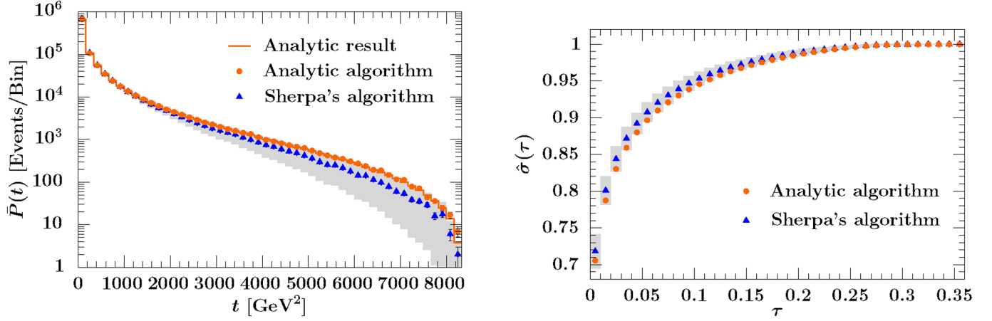
FIG. 4 (color online). Comparison of the analytic parton shower [medium (orange) dots] and SHERPA's parton shower [dark (blue) triangles]. Left panel: The function \bar{P}(t) as defined in Eq. (40). The solid (orange) line shows the result obtained from Eq. (37), and the gray shading gives an estimate of the expected size of power corrections. Right panel: The integrated thrust distribution, where the gray shading shows the expected size of finite perturbative corrections. The error bars show the statistical uncertainties.
