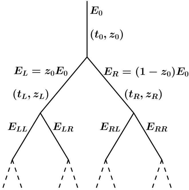
FIG. 1. Diagrammatic representation of a tree of branches.
