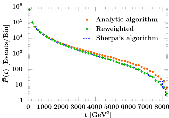
FIG. 6 (color online). The function \bar{P}(t) , as defined in Eq. (40), for the analytic parton shower [medium (orange) dots], after reweighting [light (green) diamonds], and for SHERPA's parton shower [dashed (blue) line]. Error bars indicate statistical uncertainties. See text for further explanation.
