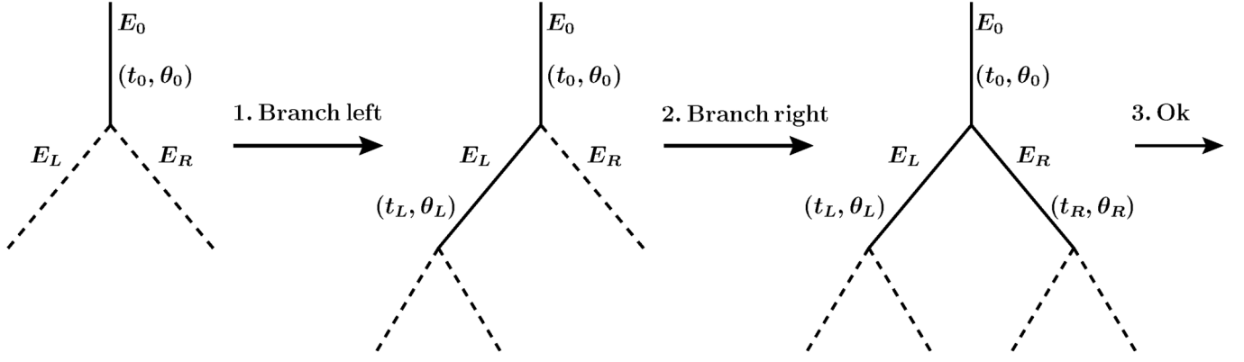
FIG. 3. Diagrammatic representation of the analytic algorithm. Solid lines represent off-shell partons with nonzero invariant mass, while dashed lines represent unbranched, on-shell partons. The evolution of t_L in step 1 starts at t_{\text{ini}} = t_0 , and that of t_R in step 2 at t_{\text{ini}} = (\sqrt{t_0} - \sqrt{t_L})^2 .
