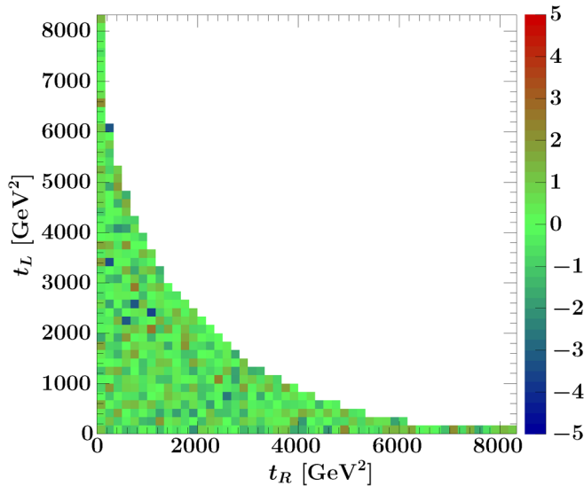
FIG. 5 (color online). Pull distribution for the double branch probability P(t_L, t_R) defined in Eq. (42). See text for further explanation.
