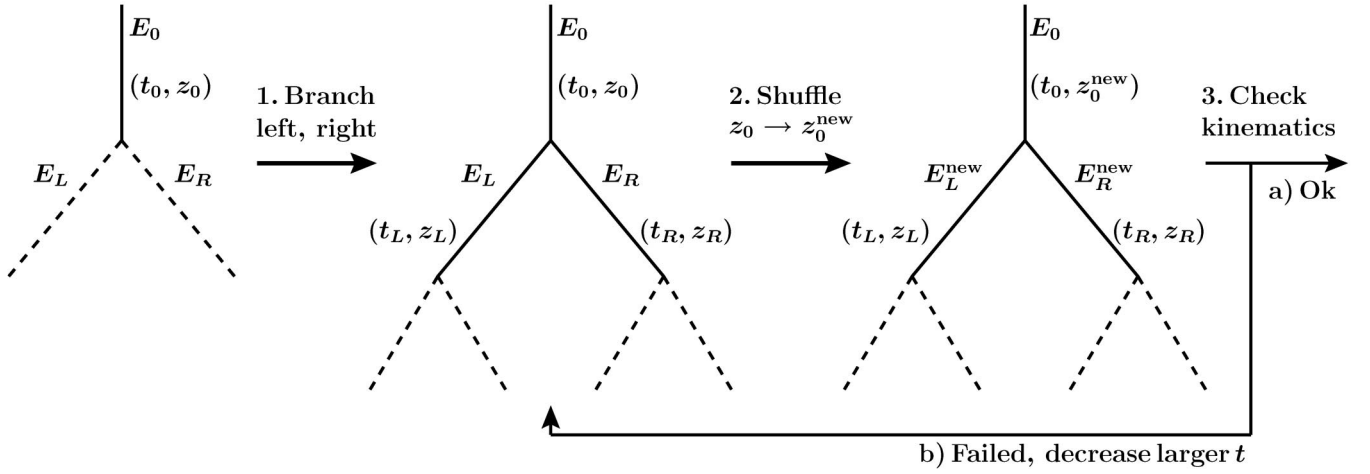
FIG. 2. Diagrammatic representation of a standard parton shower algorithm. Solid lines represent off-shell partons with nonzero invariant mass, while dashed lines represent unbranched, on-shell partons.
