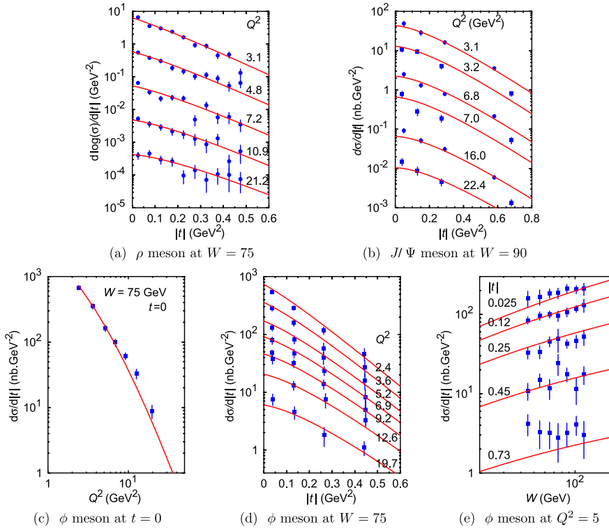
FIG. 3 (color online). Fit results for the \rho (H1 [20]), \phi (ZEUS [21]), and J/\Psi (ZEUS [22], H1 [23]) differential cross section.
