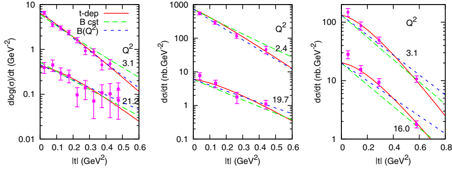
FIG. 4 (color online). Comparison of the three parametrizations for differential cross sections. The left plot shows the \rho -meson production at Q^2 = 3.1 and 21.2 \text{GeV}^2 , the middle one displays the \phi meson at Q^2 = 2.4 and 19.7 \text{GeV}^2 , and the rightmost corresponds to the J/\Psi meson at Q^2 = 3.1 and 16.0 \text{GeV}^2 . Continuous lines: t -dependent saturation; fat-dashed lines: t -independent saturation, fixed slope; thin-dashed lines: Q^2 -dependent slope.
