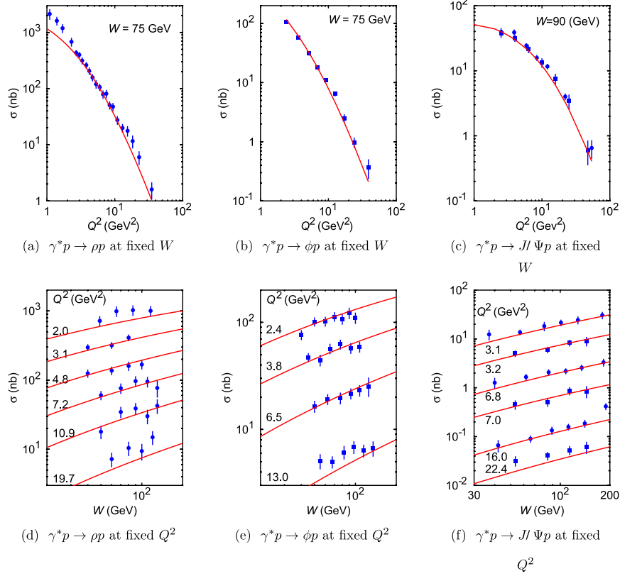
FIG. 2 (color online). Fit results for the \rho (H1 [20]), \phi (ZEUS [21]), and J/\Psi (ZEUS [22]) elastic cross sections.
