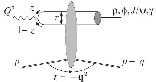
FIG. 1. Vector-particle production in the dipole frame. The amplitude factorizes as a product of vertex functions and elastic dipole-proton interaction amplitude (see formula (3)).
