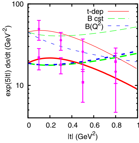
FIG. 6 (color online). Predictions of the three models studied in this paper for the DVCS diffractive cross section. For more clarity, we have multiplied the differential cross section by \exp(5|t|) . The thin lines are related to Q^2 = 4 \text{ GeV}^2 and W = 71 \text{ GeV} , while the thick ones are obtained with Q^2 = 8 \text{ GeV}^2 and W = 82 \text{ GeV} .
