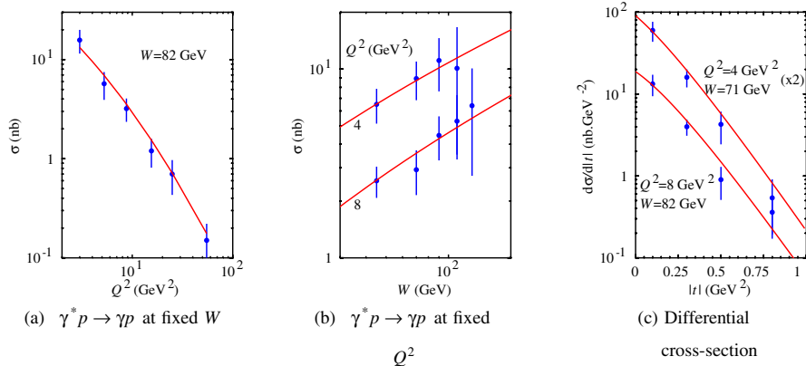
FIG. 5 (color online). Predictions for the DVCS measurements. The data are from H1 [25].
