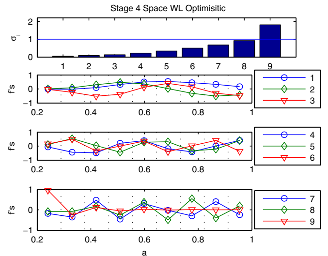
FIG. 2 (color online). The impact of the DETF “Stage 4 space weak lensing optimistic” data model: This is a much higher quality data set vs Stage 2. More modes are well measured and the well measured modes reach to higher redshift (lower a ). This plot has the same format as Fig. 1.
