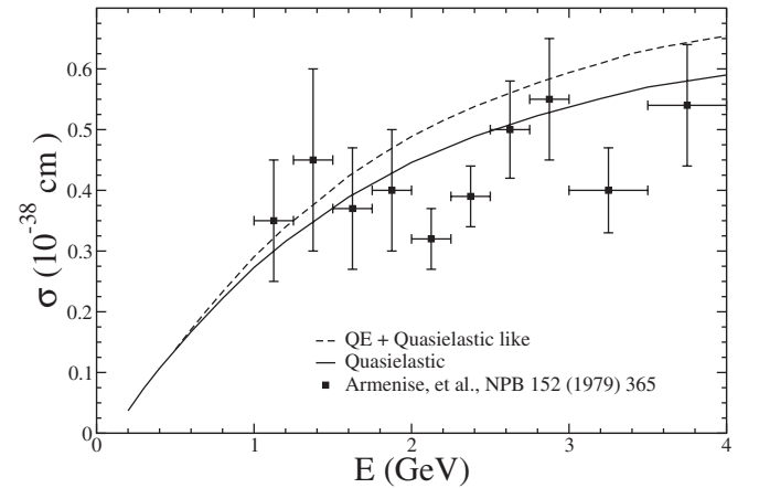
FIG. 11. Charged current lepton production cross section per nucleon induced by \bar{\nu}_\mu on freon-propane ( \text{CF}_3\text{Br} - \text{C}_3\text{H}_8 ). The result shown by solid line is the quasielastic lepton production cross section with nuclear medium effects including RPA, and the result shown by dashed line also includes the quasielastic like lepton production cross section in the delta dominance model. The experimental points are taken from Armenise et al. [6].
