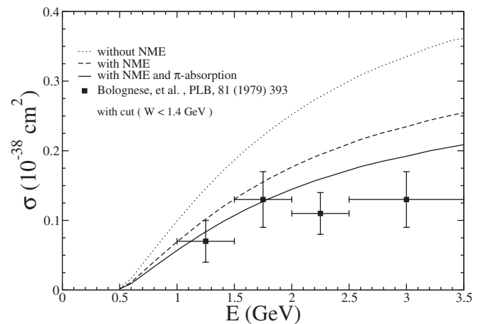
FIG. 17. Charged current 1\pi^- production cross section per neutron induced by \bar{\nu}_\mu on freon-propane ( \text{CF}_3\text{Br} - \text{C}_3\text{H}_8 ) target, with and without nuclear medium effects (NME), and with nuclear medium and pion absorption effects. The experimental points are taken from Bolognese et al. [10].
