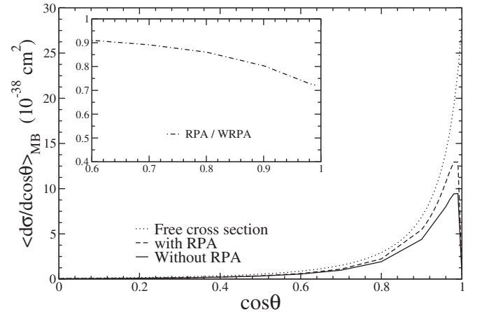
FIG. 8. \langle \frac{d\sigma}{d\cos\theta} \rangle vs \cos\theta for \bar{\nu}_\mu on ^{12}\text{C} target averaged over the MiniBooNE spectrum for the charged current quasielastic lepton production process, for the free case and with nuclear medium effects including RPA (without RPA). In the inset the ratio of \langle \frac{d\sigma}{d\cos\theta} \rangle with and without RPA effects has been shown.
