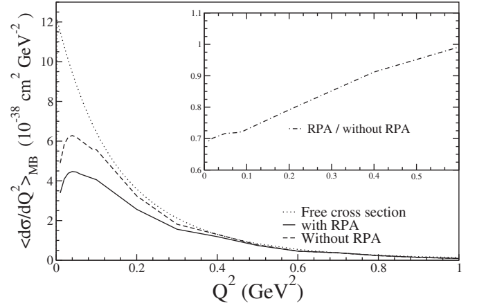
FIG. 7. \langle \frac{d\sigma}{dQ^2} \rangle vs Q^2 for \bar{\nu}_\mu on ^{12}\text{C} target averaged over the MiniBooNE spectrum for the charged current quasielastic lepton production process, for the free case and with nuclear medium effects including RPA (without RPA). In the inset the ratio of \langle \frac{d\sigma}{dQ^2} \rangle with and without RPA effects has been shown.
