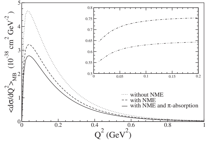
FIG. 13. \langle \frac{d\sigma}{dQ^2} \rangle vs Q^2 for \bar{\nu}_\mu on {}^{12}\text{C} target averaged over the MiniBooNE spectrum for the inelastic charged current lepton production process accompanied by a pion, with (without) nuclear medium effects (NME), and with nuclear medium and pion absorption effects. In the inset, ratio of the differential cross section in {}^{12}\text{C} as a function of Q^2 is shown. The dashed-dotted line (dashed double-dotted line) is the result of the ratio when the cross section is calculated including nuclear medium effects without (with) pion absorption effects to the cross section calculated without the nuclear medium effects.
