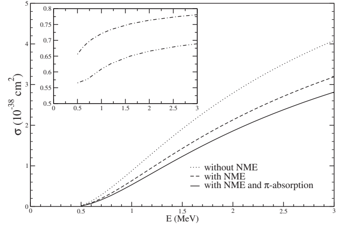
FIG. 16. Inelastic charged current one \pi^- production cross section induced by \bar{\nu}_\mu on ^{12}\text{C} target with and without nuclear medium effects (NME), and with nuclear medium and pion absorption effects. In the inset, ratio of the cross section in ^{12}\text{C} as a function of neutrino energy is shown. The dashed double-dotted line (dashed double-dotted line) is the result of the ratio when the cross section is calculated including nuclear medium effects without (with) pion absorption effects to the cross section calculated without the nuclear medium effects.
