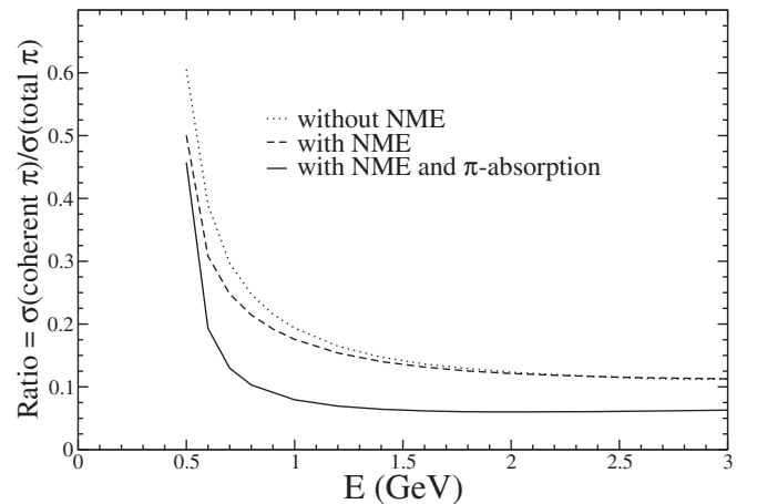
FIG. 22. Ratio of coherent charged current 1\pi^- production cross section to the total charged current 1\pi^- production cross section (incoherent + coherent) i.e. \frac{\sigma_{\text{coh}}}{\sigma_{\text{total}}} without nuclear medium effects (NME), with nuclear medium effects and with nuclear medium and pion absorption effects.
