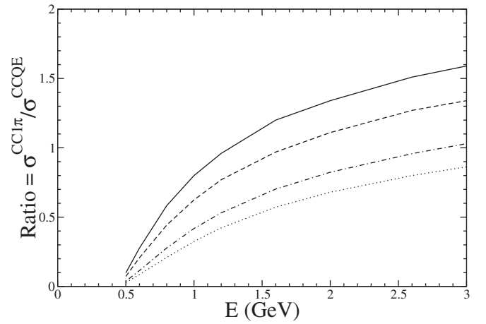
FIG. 25. Ratio of total 1\pi^- production cross section induced by \bar{\nu}_\mu on ^{12}\text{C} target to the charged current quasielastic lepton production cross section i.e. \frac{\sigma_{CC1\pi^-}}{\sigma_{CCQE}} . Result with solid (dashed) line is the ratio of the charged current induced 1\pi^- cross section calculated without nuclear medium effect to the charged current quasielastic cross section in local Fermi gas model with (without) RPA correlations, and the results with dashed-dotted (dotted) line is the ratio of the charged current induced 1\pi^- cross section calculated with nuclear medium and pion absorption effects to the charged current quasielastic cross section in local Fermi gas model with (without) RPA correlations.
