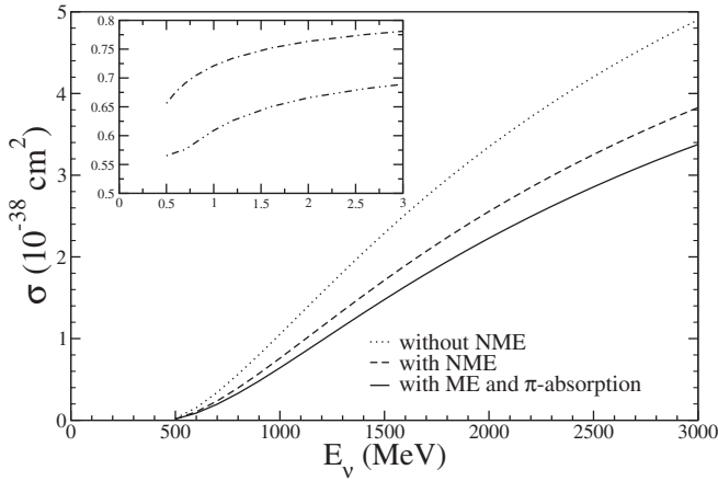
FIG. 12. The cross section for inelastic charged current lepton production accompanied by a pion induced by \bar{\nu}_\mu on {}^{12}\text{C} target, with (without) nuclear medium effects (NME) and with nuclear medium and pion absorption effects. In the inset, ratio of the cross section in {}^{12}\text{C} as a function of antineutrino energy is shown. The dashed-dotted line (dashed double-dotted line) is the result of the ratio when the cross section is calculated including nuclear medium effects without (with) pion absorption effects to the cross section calculated without the nuclear medium effects.
