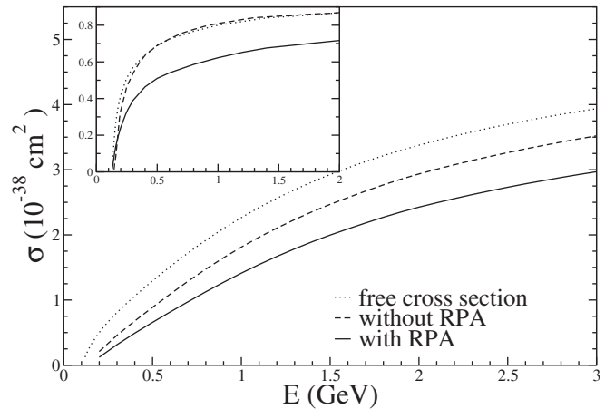
FIG. 4. Quasielastic charged current lepton production cross section induced by \bar{\nu}_\mu on {}^{12}\text{C} target for the free protons and including nuclear medium effects with (without) RPA correlations. In the inset, ratio of the cross section per nucleon in {}^{12}\text{C} to the free proton cross section as a function of neutrino energy is shown. The solid line (dashed line) is the result for this ratio for the cross section calculated with nuclear medium effects with (without) RPA correlations. The dotted line is the prediction from the NUANCE Monte Carlo generator [12].
