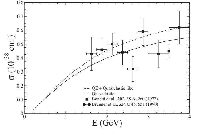
FIG. 10. Charged current lepton production cross section per nucleon induced by \bar{\nu}_\mu on freon ( \text{CF}_3\text{Br} ). The result shown by solid line is the quasielastic lepton production cross section with nuclear medium effects including RPA, and the result shown by dashed line also includes the quasielastic like lepton production cross section in the delta dominance model. The experimental points are taken from Bonetti et al. [5] and Brunner et al. [9].
