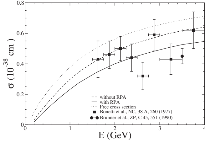
FIG. 5. Charged current quasielastic lepton production cross section per nucleon induced by \bar{\nu}_\mu on freon ( \text{CF}_3\text{Br} ), for the free case and including nuclear medium effects with (without) RPA correlations. The experimental points are taken from Bonetti et al. [5] and Brunner et al. [9].
