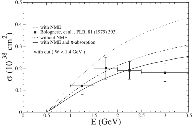
FIG. 18. Charged current 1\pi^- production cross section per nucleon induced by \bar{\nu}_\mu on freon-propane ( \text{CF}_3\text{Br} - \text{C}_3\text{H}_8 ) target, with and without nuclear medium effects (NME), and with nuclear medium and pion absorption effects. The experimental points are taken Bolognese et al. [10].
