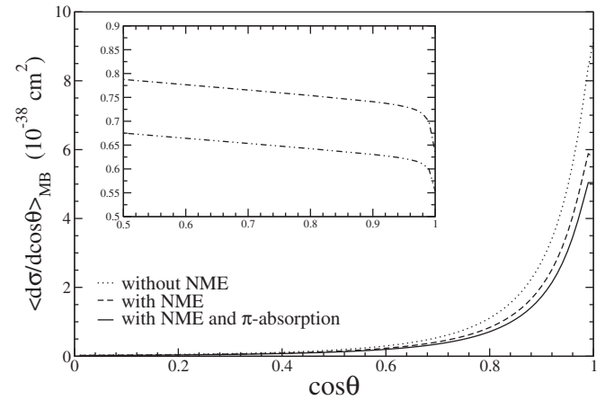
FIG. 20. \langle \frac{d\sigma}{d\cos\theta} \rangle vs \cos\theta for \bar{\nu}_\mu on ^{12}\text{C} target averaged over the MiniBooNE spectrum for the inelastic charged current lepton production process accompanied by a \pi^- , with and without nuclear medium effects (NME), and with nuclear medium and pion absorption effects. In the inset, the dashed-dotted line (dashed double-dotted line) is the result of the ratio when the cross section is calculated including nuclear medium effects without (with) pion absorption effects to the cross section calculated without the nuclear medium effects.
