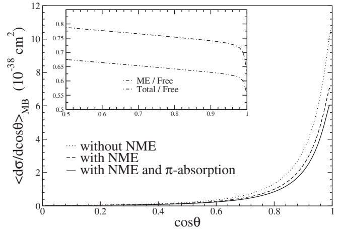
FIG. 14. \langle \frac{d\sigma}{d\cos\theta} \rangle vs \cos\theta for \bar{\nu}_\mu on {}^{12}\text{C} target averaged over the MiniBooNE spectrum for the inelastic charged current lepton production process accompanied by a pion, with (without) nuclear medium effects (NME), and with nuclear medium and pion absorption effects. In the inset, ratio of the angular distribution in {}^{12}\text{C} as a function of lepton angle is shown. The dashed-dotted line (dashed double-dotted line) is the result of the ratio when the cross section is calculated including nuclear medium effects without (with) pion absorption effects to the cross section calculated without the nuclear medium effects.
