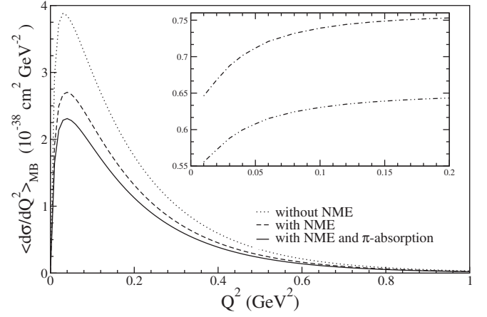
FIG. 19. \langle \frac{d\sigma}{dQ^2} \rangle vs Q^2 for \bar{\nu}_\mu on ^{12}\text{C} target averaged over the MiniBooNE spectrum for the inelastic charged current lepton production process accompanied by a \pi^- , with and without nuclear medium effects (NME), and with nuclear medium and pion absorption effects. In the inset, the dashed-dotted line (dashed double-dotted line) is the result of the ratio when the cross section is calculated including nuclear medium effects without (with) pion absorption effects to the cross section calculated without the nuclear medium effects.
