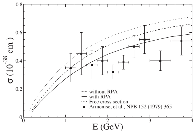
FIG. 6. Charged current quasielastic lepton production cross section per nucleon induced by \bar{\nu}_\mu on freon-propane ( \text{CF}_3\text{Br} - \text{C}_3\text{H}_8 ), for the free case and including nuclear medium effects with (without) RPA correlations. The experimental points are taken from Armenise et al. [6].
