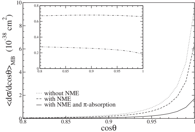
FIG. 24. \langle \frac{d\sigma}{d\cos\theta} \rangle vs \cos\theta for \bar{\nu}_\mu on ^{12}\text{C} target averaged over the MiniBooNE spectrum for the coherent charged current 1\pi^- production process, with and without nuclear medium effects (NME), and with nuclear medium and pion absorption effects. In the inset, the dashed-dotted line (dashed double-dotted line) is the result of the ratio when the cross section is calculated including nuclear medium effects without (with) pion absorption effects to the cross section calculated without the nuclear medium effects.
