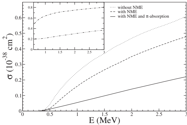
FIG. 21. Coherent charged current one pion production cross section induced by \bar{\nu}_\mu on {}^{12}\text{C} target, with and without nuclear medium effects (NME), and with nuclear medium and pion absorption effects. In the inset, the dashed-double-dotted line (dashed double-dotted line) is the result of the ratio when the cross section is calculated including nuclear medium effects without (with) pion absorption effects to the cross section calculated without the nuclear medium effects.
