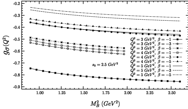
FIG. 4. The same as in Fig. 2, but for values of \beta : \beta = -1, \beta = -3, \beta = -5 .
