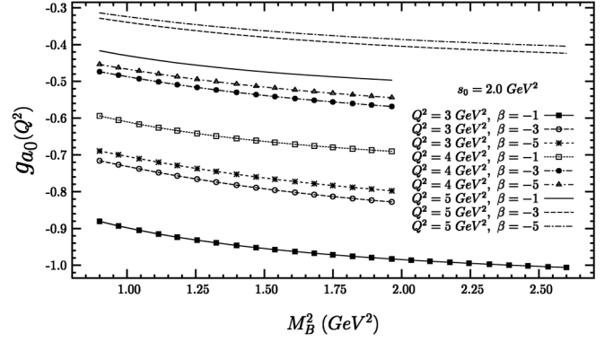
FIG. 7. The same as in Fig. 5, but for values of \beta : \beta = -1, \beta = -3, \beta = -5 .
