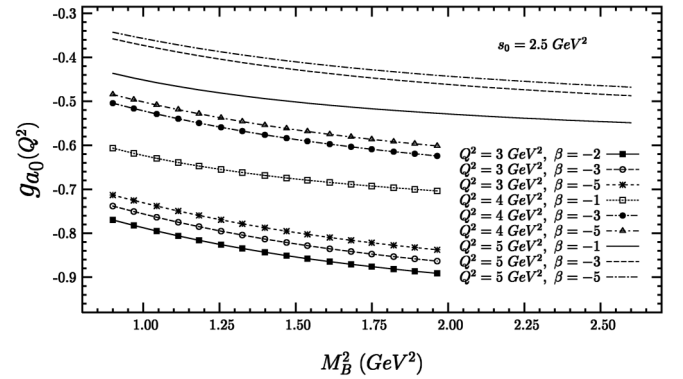
FIG. 8. The same as in Fig. 7, but at s_0 = 2.5 \text{ GeV}^2 .
