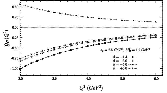
FIG. 10. The same as in Fig. 9, but at s_0 = 2.5 \text{ GeV}^2 .
