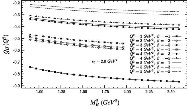
FIG. 3. The same as in Fig. 1, but for values of \beta : \beta = -1, -3, -5 .
