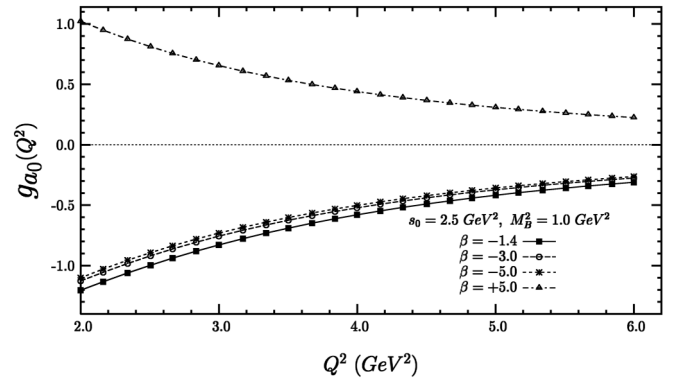
FIG. 12. The same as in Fig. 11, but at s_0 = 2.5 \text{ GeV}^2 .
