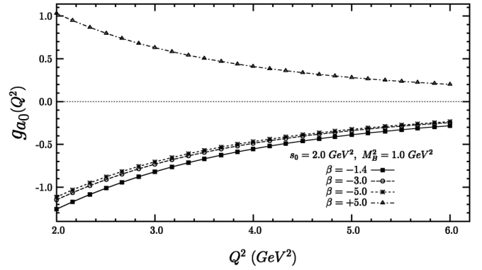
FIG. 11. The dependence of the scalar form factor induced by the scalar current with a_0 meson quantum numbers, on Q^2 at M_B^2 = 1 \text{ GeV}^2 and s_0 = 2 \text{ GeV}^2 , at fixed values of \beta = -1.4 , \beta = -3 , \beta = -5 , \beta = 5 .
