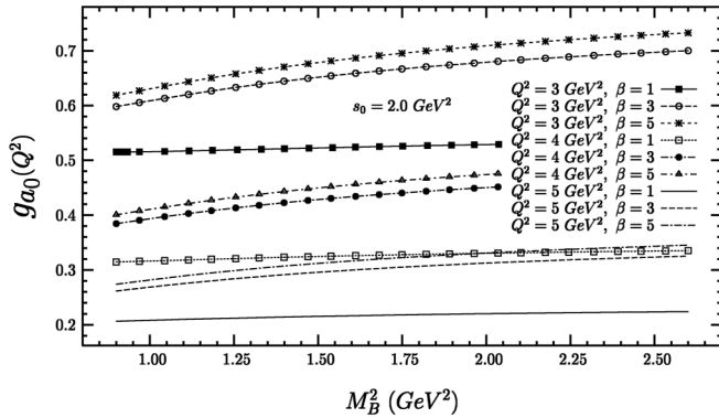
FIG. 5. The same as in Fig. 1, but for the scalar form factor induced by the scalar current with quantum number of a_0 meson.
