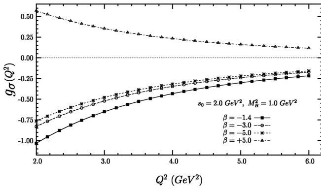
FIG. 9. The dependence of the scalar form factor induced by the scalar current with \sigma meson quantum numbers, on Q^2 at M_B^2 = 1 \text{ GeV}^2 and s_0 = 2 \text{ GeV}^2 , at fixed values of \beta = -1.4 , \beta = -3 , \beta = -5 , \beta = 5 .
