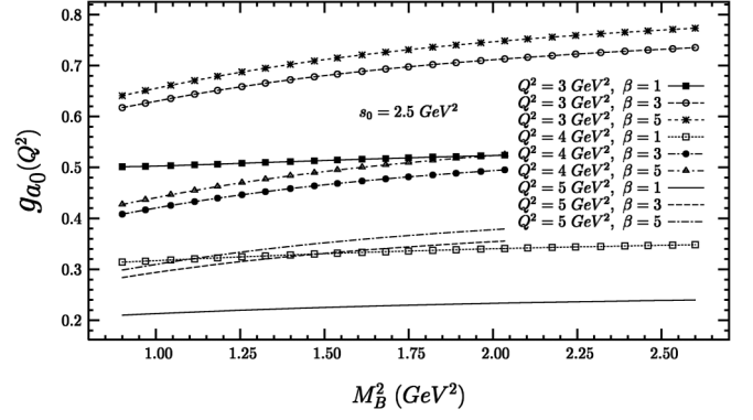
FIG. 6. The same as in Fig. 5, but at s_0 = 2.5 \text{ GeV}^2 .
