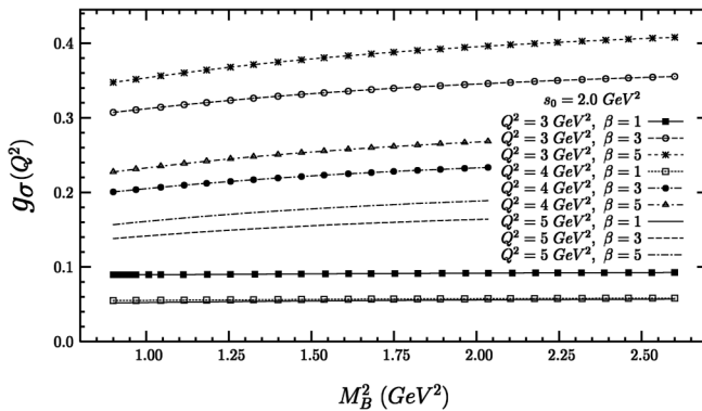
FIG. 1. The dependence of the scalar form factor of nucleon due to the scalar current with quantum numbers of \sigma meson, on Borel parameter M_B^2 at s_0 = 2 GeV 2 for three different values of Q^2 and \beta : Q^2 = 3 GeV 2 , Q^2 = 4 GeV 2 , Q^2 = 5 GeV 2 and \beta = 1 , \beta = 3 , \beta = 5 .
