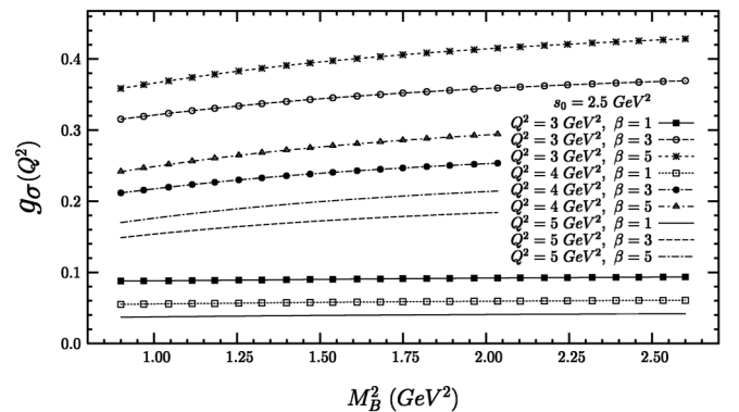
FIG. 2. The same as in Fig. 1, but at s_0 = 2.5 GeV 2 .
