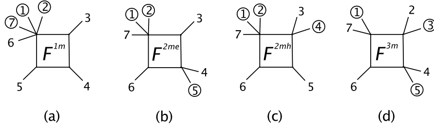
FIG. 2. Examples of box-integral functions B(i, j, k) appearing in seven-point amplitudes; the arguments i, j, k are circled: (a) the one-mass box B(1, 2, 7) = F^{1m}(s_{34}, s_{45}, s_{345}) , (b) the “easy” two-mass box B(1, 2, 5) = F^{2me}(s_{345}, s_{456}, s_{45}, s_{712}) , (c) the “hard” two-mass box B(1, 2, 4) = F^{2mh}(s_{56}, s_{345}, s_{712}, s_{34}) , and (d) the three-mass box B(1, 3, 5) = F^{3m}(s_{671}, s_{456}, s_{71}, s_{23}, s_{45}) .
