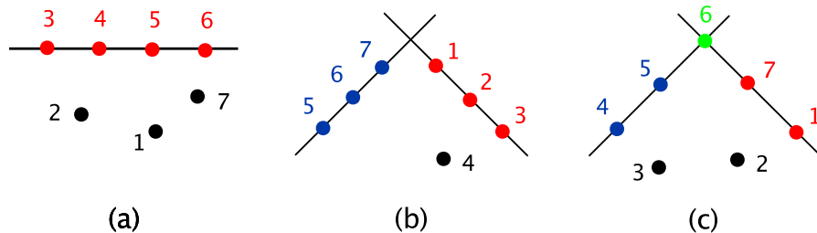
FIG. 5 (color online). Examples of twistor-space configurations for single-term box coefficients in the helicity amplitude A_{7,1}^{\mathcal{N}=4}(1^-, 2^-, 3^+, 4^-, 5^+, 6^+, 7^+) . In every case, all the points lie in a plane. (a) The easy two-mass box coefficient c_{125} , (b) the hard two-mass box coefficient c_{237} , (c) the three-mass box coefficient c_{135} .
