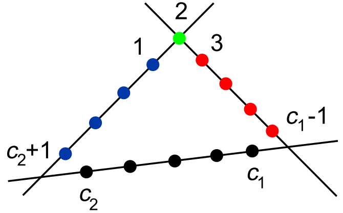
FIG. 6 (color online). The twistor-space configuration for the class of three-mass-box coefficients in the helicity amplitude (- - - + + \cdots + +) discussed in the text. All points lie in a plane.
