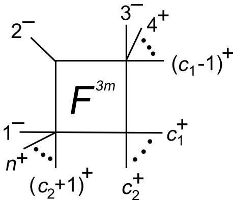
FIG. 4. The class of three-mass box functions whose coefficient is given in Eq. (199).
