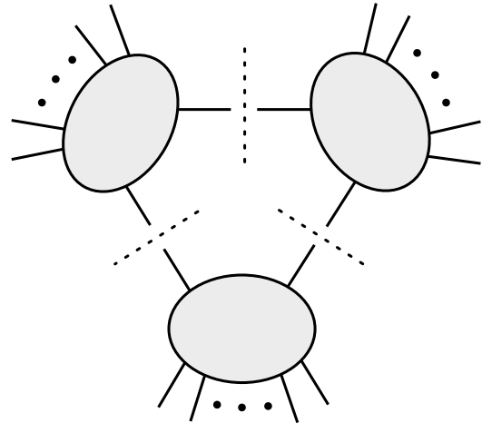
FIG. 1. A generalized “triple cut.” The three propagators cut by the dashed lines are required to be “open.”
