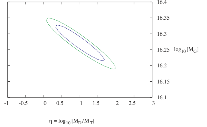
FIG. 2 (color online). Plot showing 95% and 99.73% contours in the plane of \eta and M_G . This clearly shows that from the viewpoint of unification a triplet lighter than a doublet is preferred.
