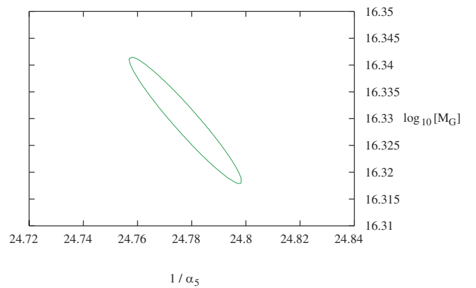
FIG. 1 (color online). Plot showing 99.73% contour for two loop SUSY running with only the MSSM particle content. \alpha_5 is the unified coupling constant at the GUT scale.
