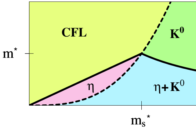
FIG. 2 (color online). The phase diagram as a function of light quark mass m and strange quark mass m_s . The phases marked CFL, K^0 , \eta , and \eta + K^0 are, respectively, the CFL phase without meson condensation, with kaon condensation, with \eta condensation, and with both \eta and K^0 condensation. Phase transitions are represented by a solid line if first order, a dashed line if second order. The location of the tetra-critical point is \{m_s^*, m^*\} , given in Eq. (16); including subleading effects causes it to split into two tricritical points.
