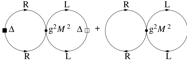
FIG. 1. Feynman diagrams corresponding to the g^2 M^2 terms in the effective potential. The open and solid squares denote insertions of the gap, and the dot is an effective vertex which describes chirality changing quark-quark scattering amplitudes.
