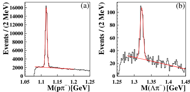
FIG. 1 (color online). (a) Invariant mass distribution of the p\pi^- system. (b) Invariant mass distribution of the p\pi^-\pi^- system. Both invariant mass distributions contain also the charge conjugate (c.c.) modes ( \bar{p}\pi^+ , \bar{p}\pi^+\pi^+ ) and are subject to the constraints in event topology discussed in the text.
