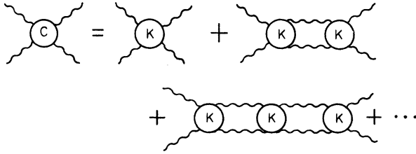
FIG. 2. Iteration of Fig. 1(b).
