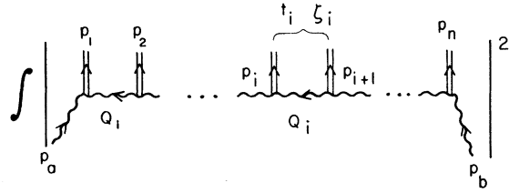
FIG. 3. Kinematics of the n -cluster contribution to the absorptive part.
