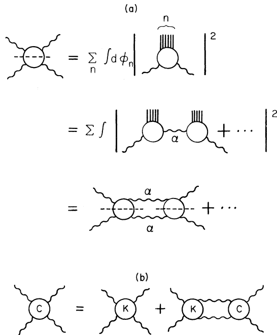
FIG. 1. (a) Generation of the two-Reggeon cut. (b) Exact equation for the two-Reggeon absorptive part.
