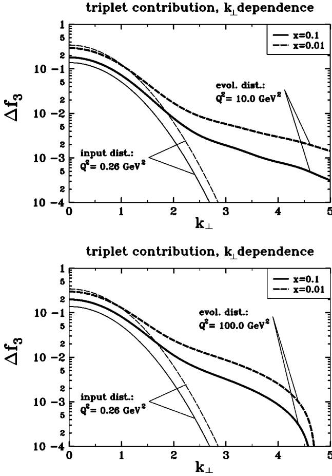
FIG. 2. Transverse momentum dependence for the triplet contribution \Delta f_3 = \frac{1}{6}(\Delta u + \Delta \bar{u} - \Delta d - \Delta \bar{d}) of the full modified pCCFM evolution (approximate form: Altarelli Parisi + ladder + nonladder). The thin lines show the input distributions GRSV LO standard scenario [17] for Q_0^2 = 0.26 \text{ GeV}^2 for x = 0.1 (solid) and x = 0.01 (dashed), while the bold lines show the same distribution evolved to Q^2 = 10 \text{ GeV}^2 (top) and Q^2 = 100 \text{ GeV}^2 (bottom). It can be seen from the logarithmical scale that the evolution leads to a k_\perp broadening away from the Gaussian shape to a mere simple exponential decay.
