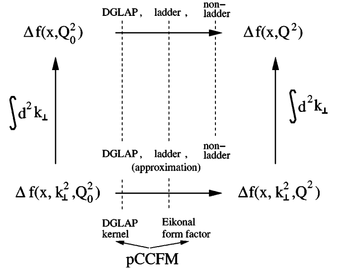
FIG. 3. Relationship between the pCCFM evolution and its modified approximate form for unintegrated parton distributions on the one hand and the evolution of integrated parton distributions on the other hand.
