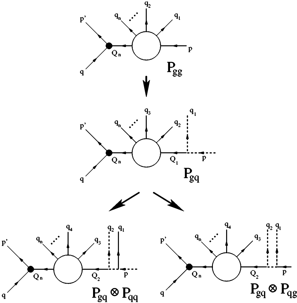
FIG. 1. Construction of the polarized CCFM equation for quarks from the one for gluons. The kernels for qq , qg , and gq splitting are subsequently constructed from the gg soft emission by amending the corresponding hard initial states. Here the solid line describes gluons while the dashed line denotes quarks.
