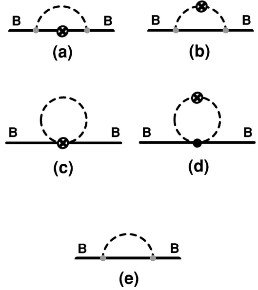
FIG. 3. One-loop diagrams that contribute to the matrix elements of the isovector twist-2 operators in mesons containing a heavy quark. The solid lines denote mesons containing a heavy quark, while the dashed lines denote light mesons. The crossed circle denotes an insertion of \mathcal{O}_{\mu_1\mu_2\ldots\mu_n}^{(n),a} while the small solid circle denotes a strong interaction \propto g_\pi .
