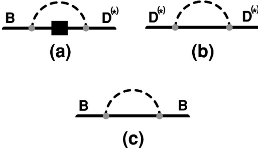
FIG. 1. One-loop diagrams that contribute to the matrix elements for B \rightarrow D^{(*)} . The solid lines denote mesons containing a heavy quark, while the dashed lines denote light mesons. The solid square corresponds to an insertion of the weak interaction vertex, while the small solid circles denote a strong interaction vertex \propto g_\pi . Diagram (a) is a vertex correction, while diagrams (b) and (c) correspond to wave function renormalization.
