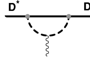
FIG. 2. One-loop diagrams that contribute to the radiative transitions D^* \rightarrow D\gamma . The solid lines denote mesons containing a heavy quark, the dashed lines denote light mesons and the small solid circle denotes a strong interaction \propto g_\pi .
