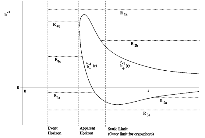
FIG. 4. Effective potential, \hat{b}_{\pm}^{-1} = \hat{E}/\hat{L} , versus r for light in a medium with both radial and azimuthal flow. Broken lines R_2 , R_3 , and R_4 refer to the three possible photon trajectories.
