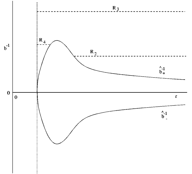
FIG. 2. Perfect sink: effective potential, \hat{b}_{\pm}^{-1} = \hat{E}/\hat{L} , versus r . Broken lines R_2 , R_3 , and R_4 refer to the three possible photon trajectories.
