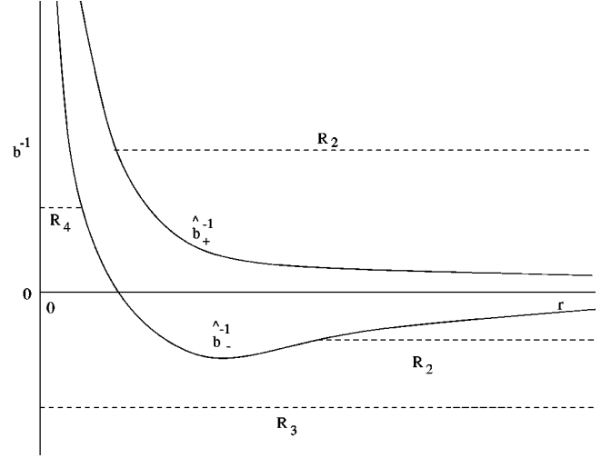
FIG. 3. Perfect vortex: effective potential, \hat{b}_\pm^{-1} = \hat{E}/\hat{L} , versus r . Broken lines R_2 , R_3 and R_4 refer to the three possible photon trajectories.
