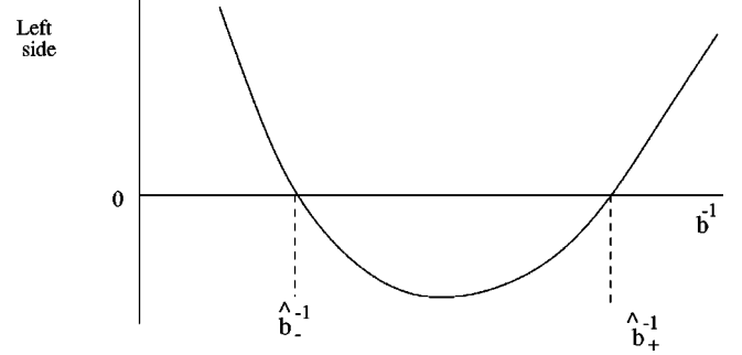
FIG. 1. Qualitative sketch of the left hand side of Eq. (32) versus b^{-1} , when r^2 > \kappa\Gamma^2 .
