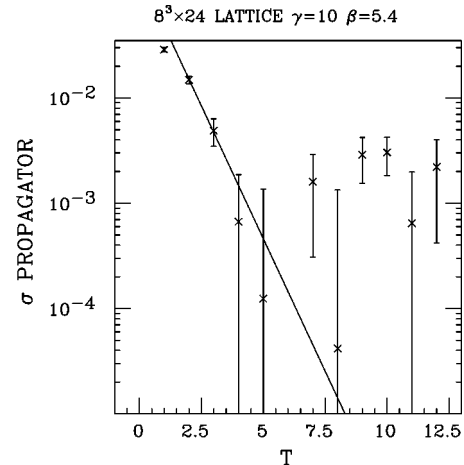
FIG. 3. The \sigma propagator at zero temperature; the curve is the single particle fit described in the text.
