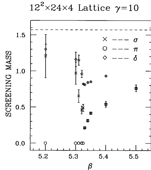
FIG. 7. The \sigma(f_0) and \pi screening masses as functions of \beta .
