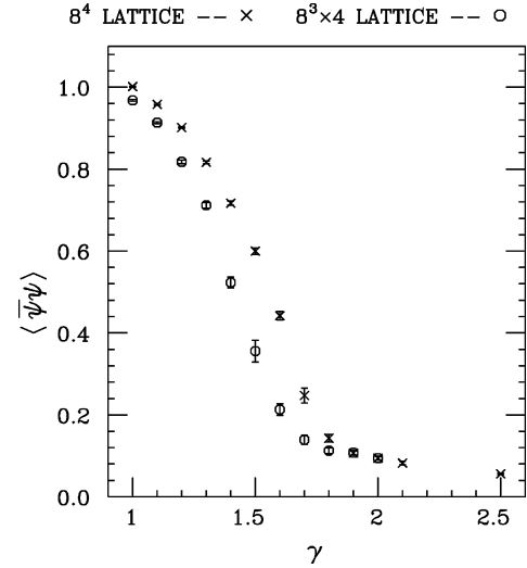
FIG. 1. \langle \bar{\psi}\psi \rangle as a function of \gamma for the pure 4-fermion theory for both zero and finite temperatures.
