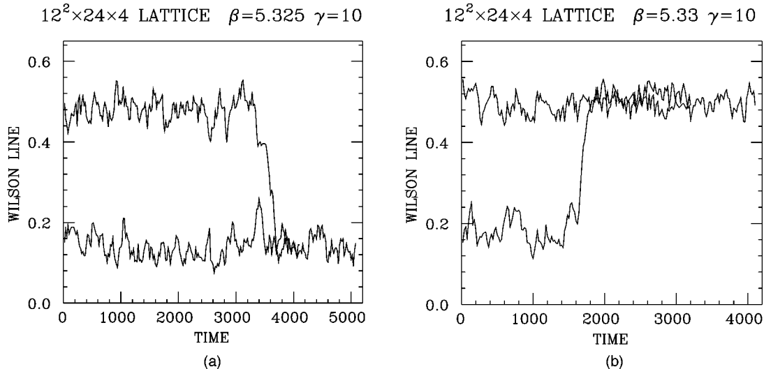
FIG. 6. Time evolution of the Wilson/Polyakov line on a 12^2 \times 24 \times 4 lattice (a) at \beta=5.325 and (b) at \beta=5.33 .
