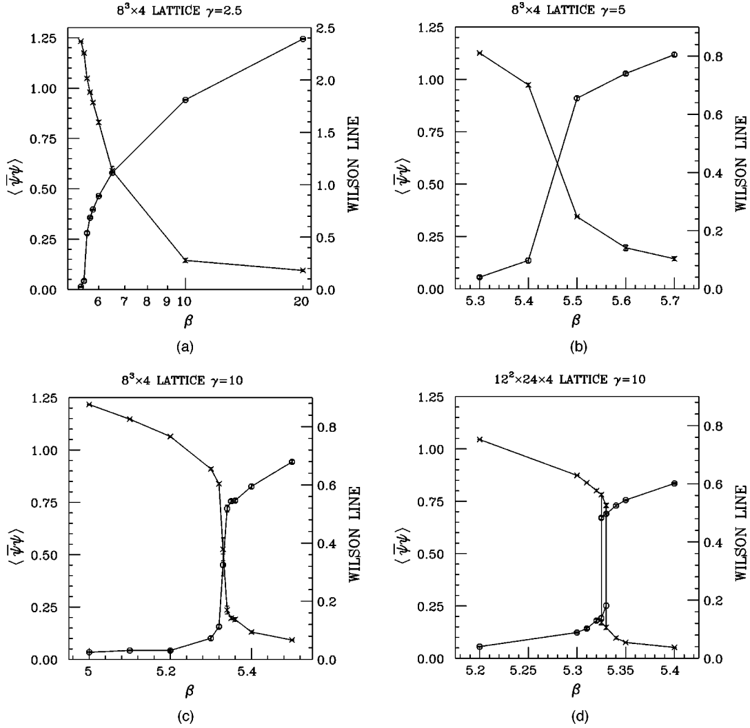
FIG. 4. Wilson/Polyakov line (circles) and \langle \bar{\psi}\psi \rangle (crosses) versus \beta for (a) an 8^3 \times 4 lattice at \gamma=2.5 , (b) an 8^3 \times 4 lattice at \gamma=5 , (c) an 8^3 \times 4 lattice at \gamma=10 , and (d) a 12^2 \times 24 \times 4 lattice at \gamma=10 .
