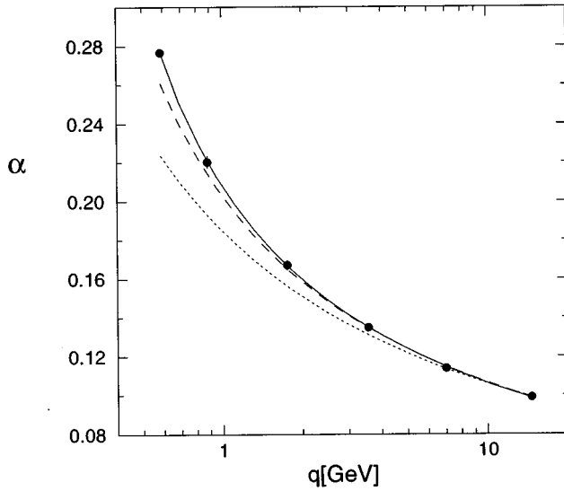
FIG. 1. The results of nonperturbative evaluation of particularly defined QCD running coupling \alpha_s^{\text{latt}}(\mu) on the lattice. Taken from Ref. [19].
