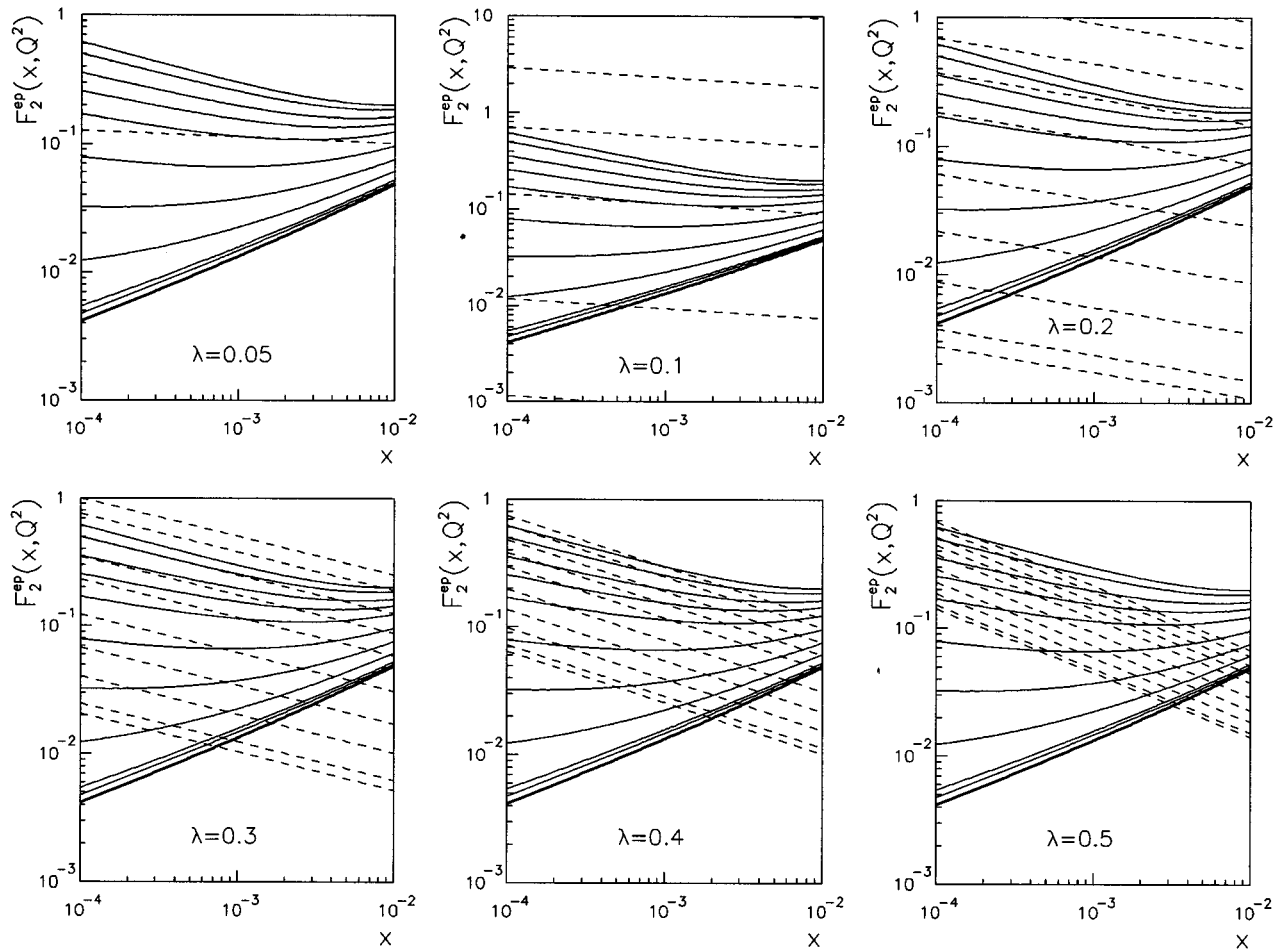
FIG. 4. The comparison of the GRV (solid curves) and conventional (dashed curves) results for F_2^{ep}(x, Q^2) separately for six values of \lambda in the latter approach.
