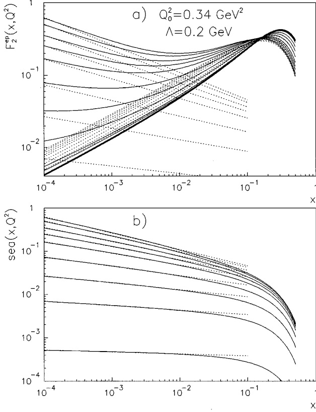
FIG. 2. (a) F_2^{ep}(x, Q^2) as a function of x for the initial distribution (8) and (9) and ten values of Q^2 defined in the text. In the low x region the curves are ordered from below in order of increasing Q^2 . The dotted lines correspond to the powerlike fits described in the text and the thick solid curve describes the initial F_2^{ep}(x, \mu) . (b) The same as in (a), but for the total sea component only.
