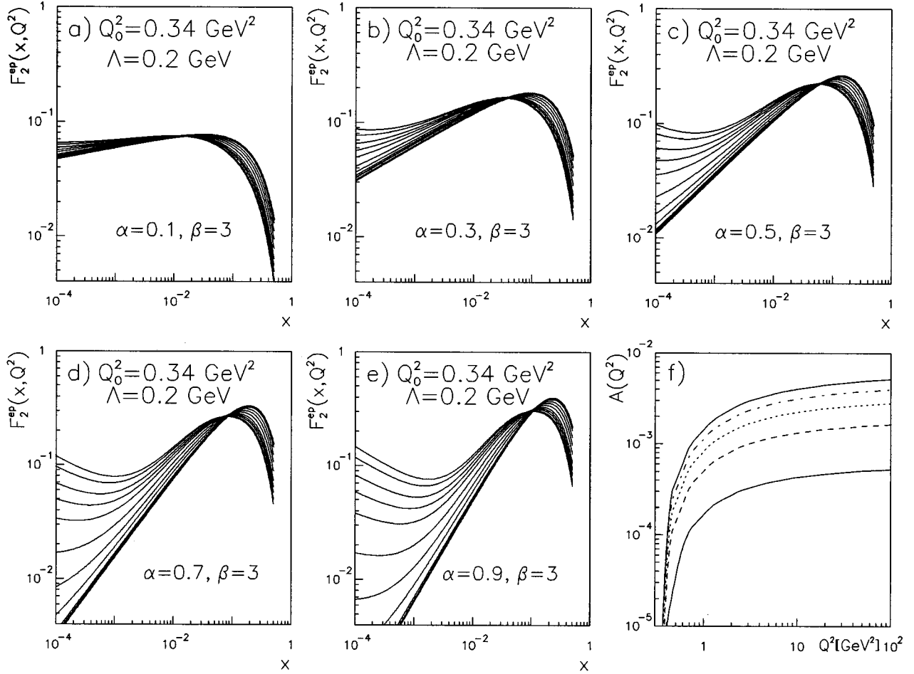
FIG. 5. The same as in Fig. 2(a) [5(a)–5(e)] and Fig. 3(a) [5(f)], but for \beta=3 and five values of \alpha in Eq. (54). In (f) the curves are ordered from above in order of increasing \alpha .
