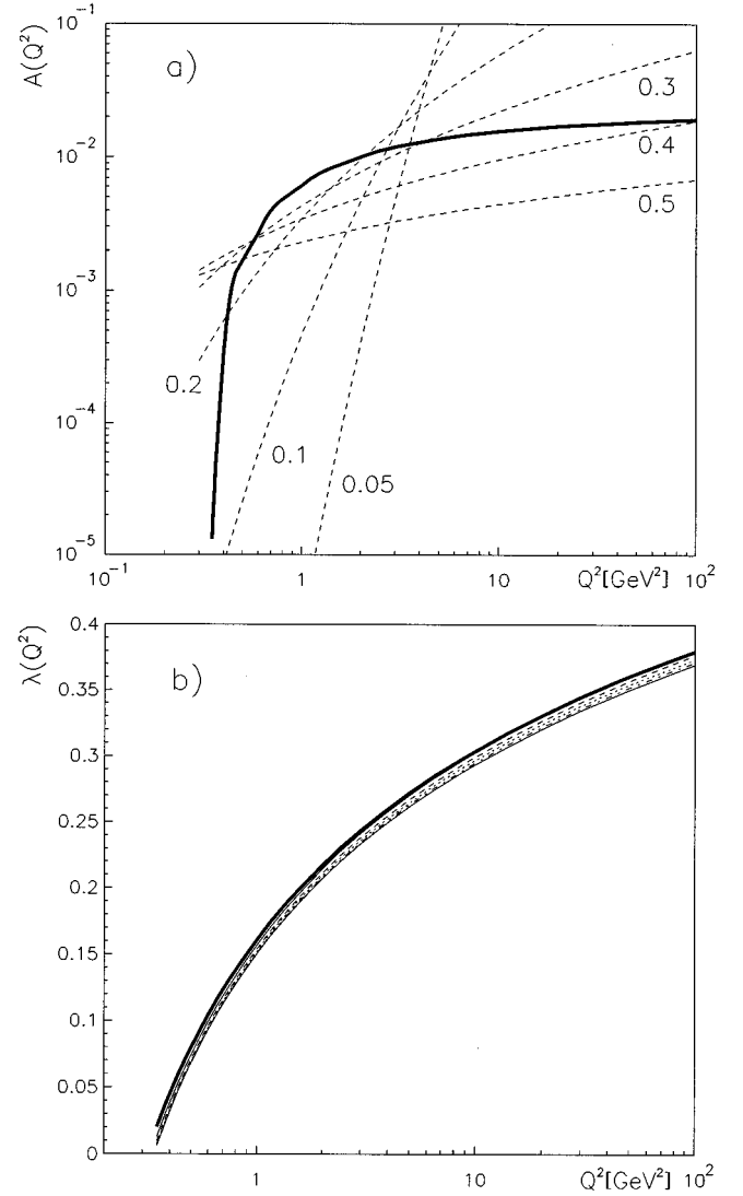
FIG. 3. Q^2 dependence of the normalization factor A(Q) (a) and the exponent \lambda(Q) (b). In (a) the thick solid curve is given by the powerlike fit of the GRV results, while the dashed lines, describing F_2^{ep}(Q, \lambda) of the conventional approach, correspond to six values of \lambda = 0.05, 0.1, 0.2, 0.3, 0.4 , and 0.5 . In (b) the thick solid curve describes again the GRV result for the initial distributions (8) and (9), while the other curves correspond (from above in decreasing order of \alpha ) to five initial distributions (54) with \beta = 3 and \alpha = 0.1, 0.3, 0.5, 0.7, 0.9 . In (b) similar curves for \beta = 4 would be essentially indistinguishable from those in the figure.
