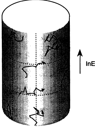
FIG. 2. Random walks in two-dimensional rapidity space (\ln E, \phi) .
