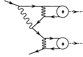
FIG. 3. One of the 14 Feynman diagrams contributing to the process q\bar{Q} \rightarrow HH' in the high-energy limit.
