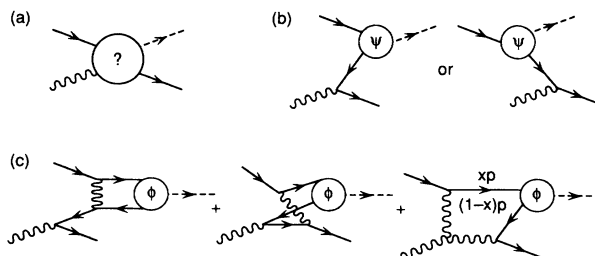
FIG. 1. Three ways of looking at the one-meson amplitude. (a) represents the full, nonperturbative amplitude, whose calculation will require extensive use of numerical methods. (b) shows the two LCPT graphs contributing to the amplitude to form the meson in its valence ( q\bar{q} ) Fock state. (c) shows the Feynman graphs which contribute in the high-energy limit.
