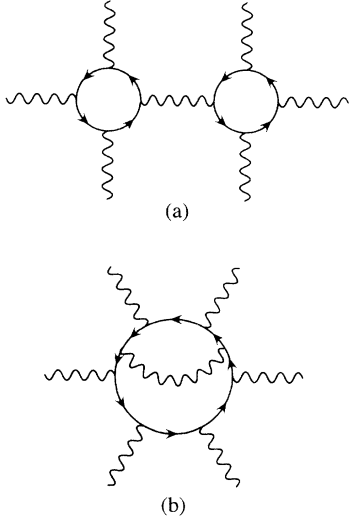
FIG. 2. Two of the two-loop diagrams for \gamma\gamma \rightarrow \gamma\gamma\gamma .
