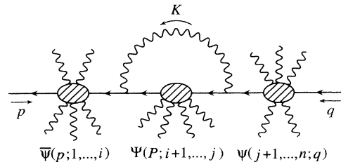
FIG. 4. The “jellyfish” diagram for the process e^+e^- \rightarrow \gamma\gamma \dots \gamma .
