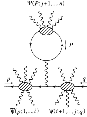
FIG. 3. The light-by-light diagram for the process e^+e^- \rightarrow \gamma\gamma \dots \gamma .
