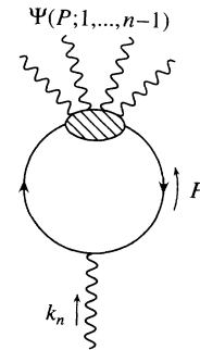
FIG. 1. The basic diagram for n -photon scattering. The blob represents the sum of all possible tree graphs with n-1 photons attached to a fermion line.
