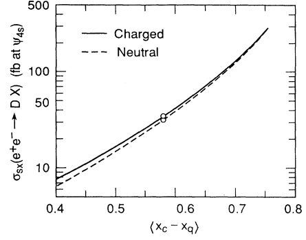
FIG. 6. The semiexclusive cross section \sigma_{sx}(e^+e^- \rightarrow DX) at B factory energies. Here we have used the toy wave function, Eq. (5). The points marked correspond to the prediction of [10] for \langle x \rangle ; [10] does not itself advance a model wave function.
