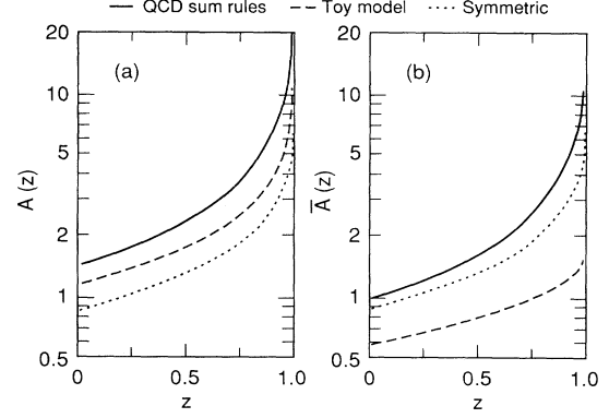
FIG. 3. The transforms A_K(z) and \bar{A}_K(z) of the distribution amplitudes in Fig. 2. When A \gg \bar{A} , as in the toy model, contributions from Feynman diagrams where the photon attaches to the light quark are suppressed.
