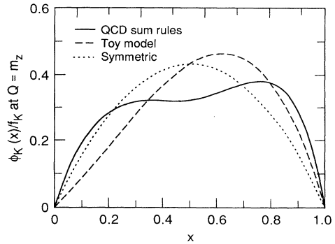
FIG. 7. The distribution amplitudes \phi_K(x; Q = m_Z) . We have used the evolution equation for the pion distribution amplitude [1].
