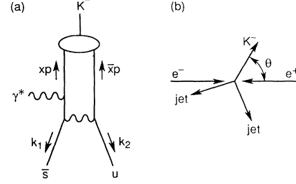
FIG. 1. (a) A Feynman diagram contributing to the semiexclusive process e^+e^- \rightarrow K^-X ; the other diagrams are obtained from different attachments of the photon line. The remaining u and \bar{s} quarks will hadronize nonperturbatively; at this level, we neglect final-state interactions and resonance physics. (b) The observed kinematics of a semiexclusive event. Note that the plane containing the K and jets need not contain the incoming beams.
