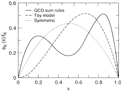
FIG. 2. Three models of the distribution amplitude \phi_K(x) . The double-humped structure of the ZZC wave function [10] is a striking result of the sum-rule calculation. Note that the exact shape of the sum-rule wave function is determined not only by the calculated moments but by the projection onto the first four Gegenbauer polynomials.
