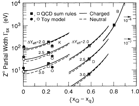
FIG. 8. Partial widths per channel d\Gamma_{sx}(Z^0 \rightarrow MX) for mesons M=K, D, B using the toy distribution amplitude, Eq. (5). The points marked on the curves for D and B mesons correspond to the values of \langle x \rangle derived in [10]. We also show points for each \phi_K(x) under consideration.
