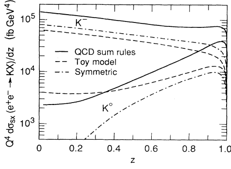
FIG. 4. The differential cross section for semiexclusive K production at Q near 10 GeV, from Eq. (4); here the y dependence has been integrated out.
