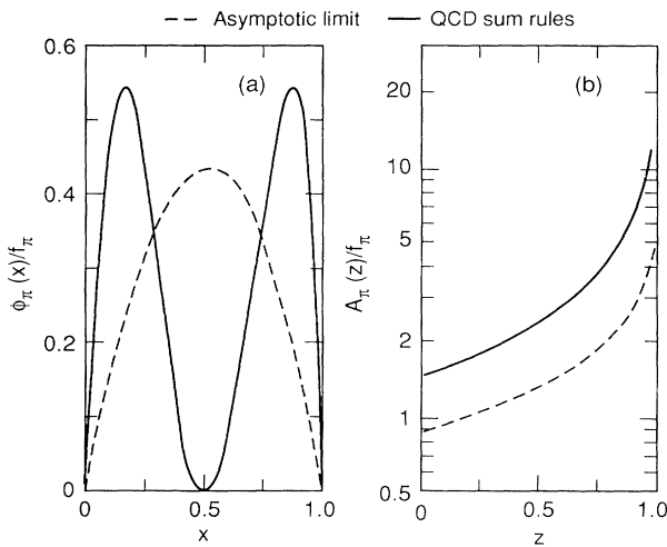
FIG. 5. (a) The distribution amplitude of [11] from QCD sum rules; and the asymptotic limit of \phi_\pi(x; Q^2) as q^2 \rightarrow \infty , the symmetric distribution [1]. (b) The resulting transforms A_\pi(z) = \bar{A}_\pi(z) . Because \phi(x) is more concentrated near the end points, A_\pi(z) is much larger for the sum-rule distribution than for the asymptotic.
