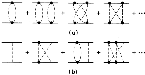
FIG. 1. Representative graphs considered in nucleon-nucleon scattering: (a) for the nonflip-nonflip helicity amplitude, (b) for the flip-flip helicity amplitude. The heavy dot indicates the correlations described in the text.
