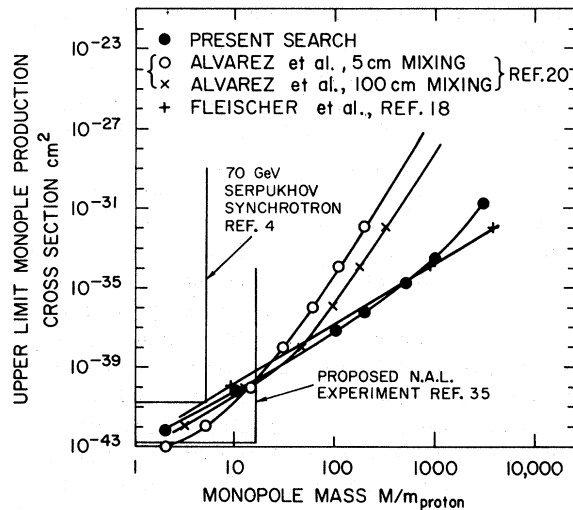
FIG. 7. Upper limit of monopole pair-production cross section (cm 2 ) versus monopole mass ( M/m_p ).
