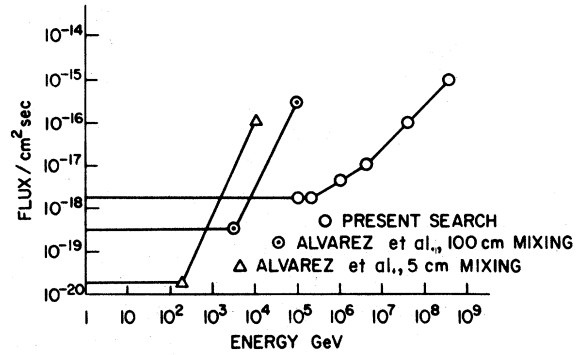
FIG. 6. Upper limit of monopole flux per (cm 2 sec) versus incident energy (GeV).
