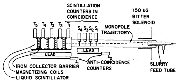
FIG. 4. Final version of monopole detector based on scintillation coincidence of minimum ionizing particles and reextraction from iron collector barriers.
