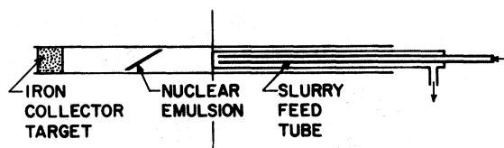
FIG. 2. Second version of monopole detector for continuous search.
