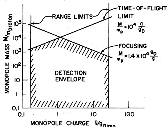
FIG. 5. Detection limits of the final apparatus.
