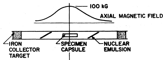
FIG. 1. First version of nuclear-track-plate camera for monopole detection.
