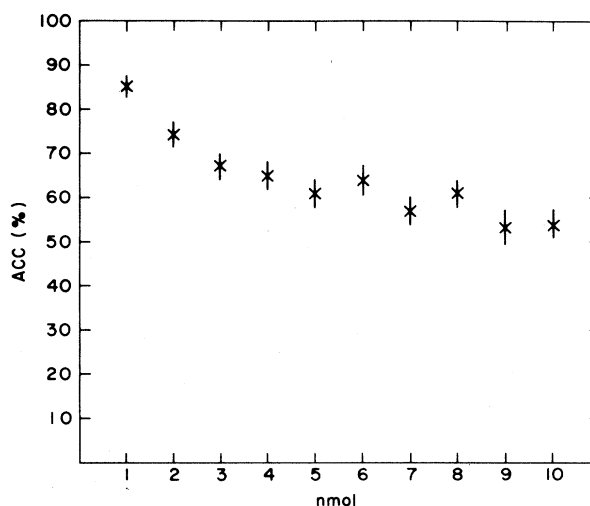
FIG. 2. Dependence of the acceptance rate on nmol , the number of iterations of Eqs. (1) between accept/reject steps. The data are obtained for \epsilon=0.01 and k=104 .
