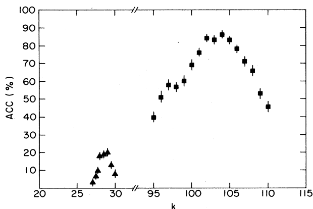
FIG. 1. Dependence of the acceptance rate on the distribution of the V_i for two values of \epsilon . The parameter k is defined by the first line in Eq. (12). Squares refer to \epsilon=0.01 and triangles refer to \epsilon=0.04 .
