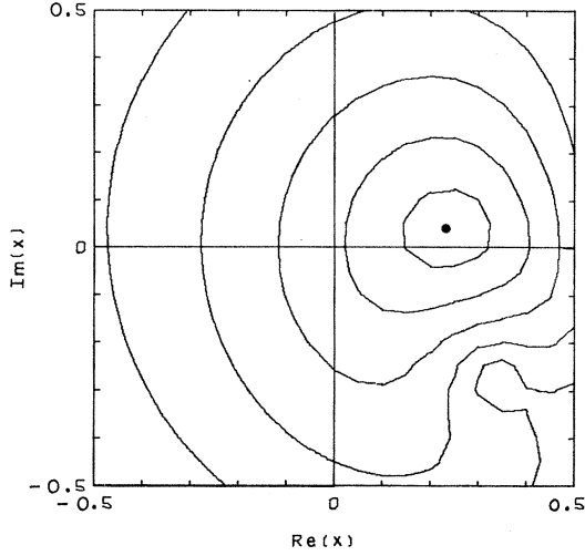
FIG. 6. Likelihood contours for the 119 identified leptonic decays. This likelihood function is the product of those in Figs. 4 and 5.
