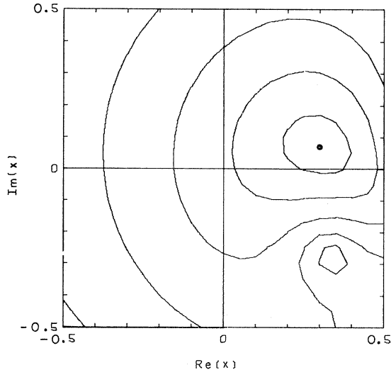
FIG. 4. Likelihood contours for the 81 identified electronic decays.
