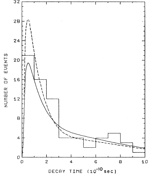
FIG. 2. Time distribution of the 73 negative leptonic decays. The solid and broken curves show the predictions for x=0 and x=0.25 , and their integrals over the first time bin are 15.0 and 21.6, respectively.
