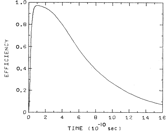
FIG. 7. Geometrical efficiency function.
