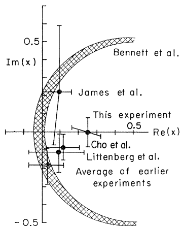
FIG. 10. Experimental results for the value of x .
