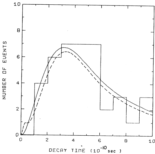
FIG. 1. Time distribution of the 46 positive leptonic decays. The solid and broken curves show the predictions for x=0 and x=0.25 , and their integrals over the first time bin are 0.92 and 0.90, respectively.
