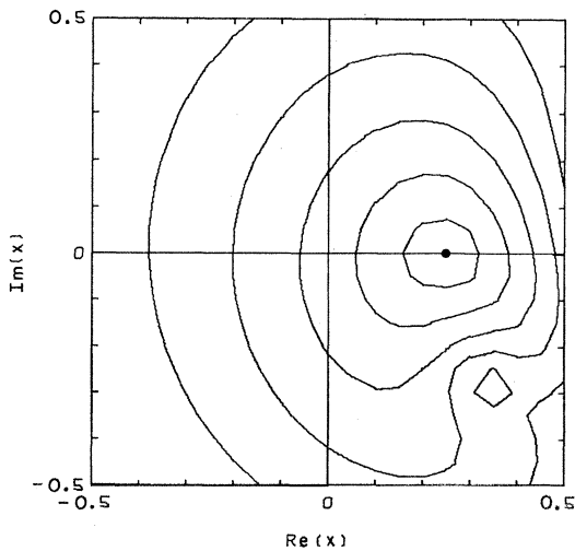
FIG. 9. Likelihood contours for all 252 events. This likelihood function is the product of those in Figs. 6 and 8.
