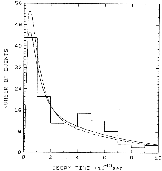
FIG. 3. Time distribution of the 133 unidentified events. The solid and broken curves show the predictions for x=0 and x=0.25 , and their integrals over the first time bin are 34.1 and 39.5, respectively.
