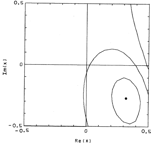
FIG. 8. Likelihood contours for the 133 unidentified events.
