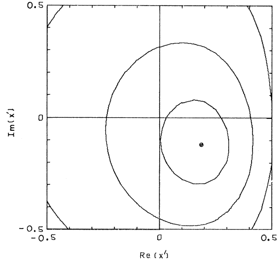
FIG. 5. Likelihood contours for the 38 identified muonic decays.
