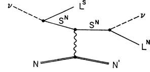
FIG. 1. Intermediate-magnetic-boson mechanism for the production of magnetic lepton pairs.
