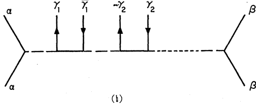
FIG. 3. (a) Diagram for quark-quark elastic scattering. (b) Diagram for the process qq \rightarrow qq + N(q\bar{q}) .
