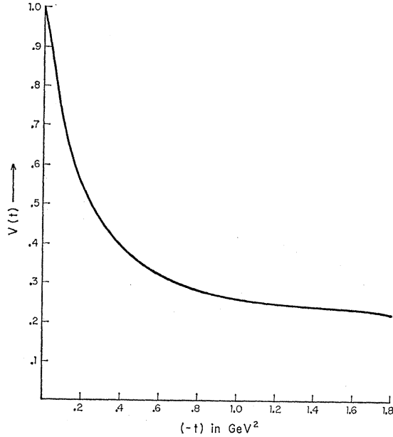
FIG. 5. Value of V(t) obtained from the calculated values of f(t) for pp and f(t) for qq .
